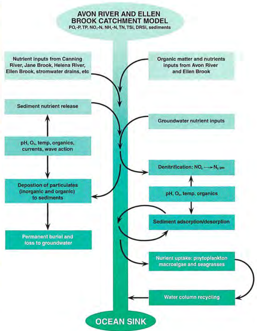
Figure 1: Major estuarine biogeological chemical processes
