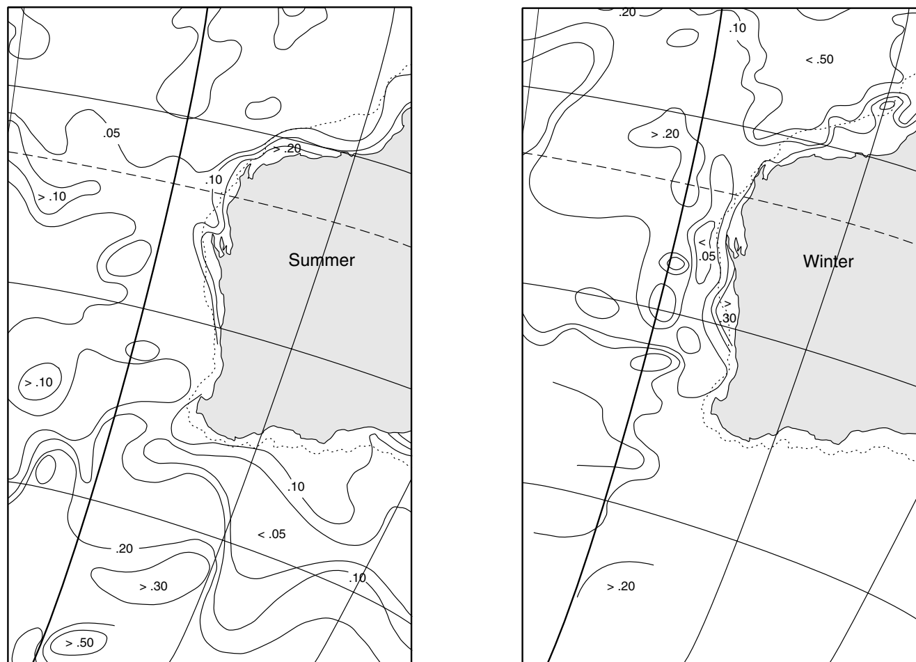
Figure 3 Surface chlorophyll concentrations ( \mu\text{g/L} ) in the south-eastern Indian Ocean in summer (November to April) (left) and winter (May to October) (right) from Krey and Babenerd (1976).
