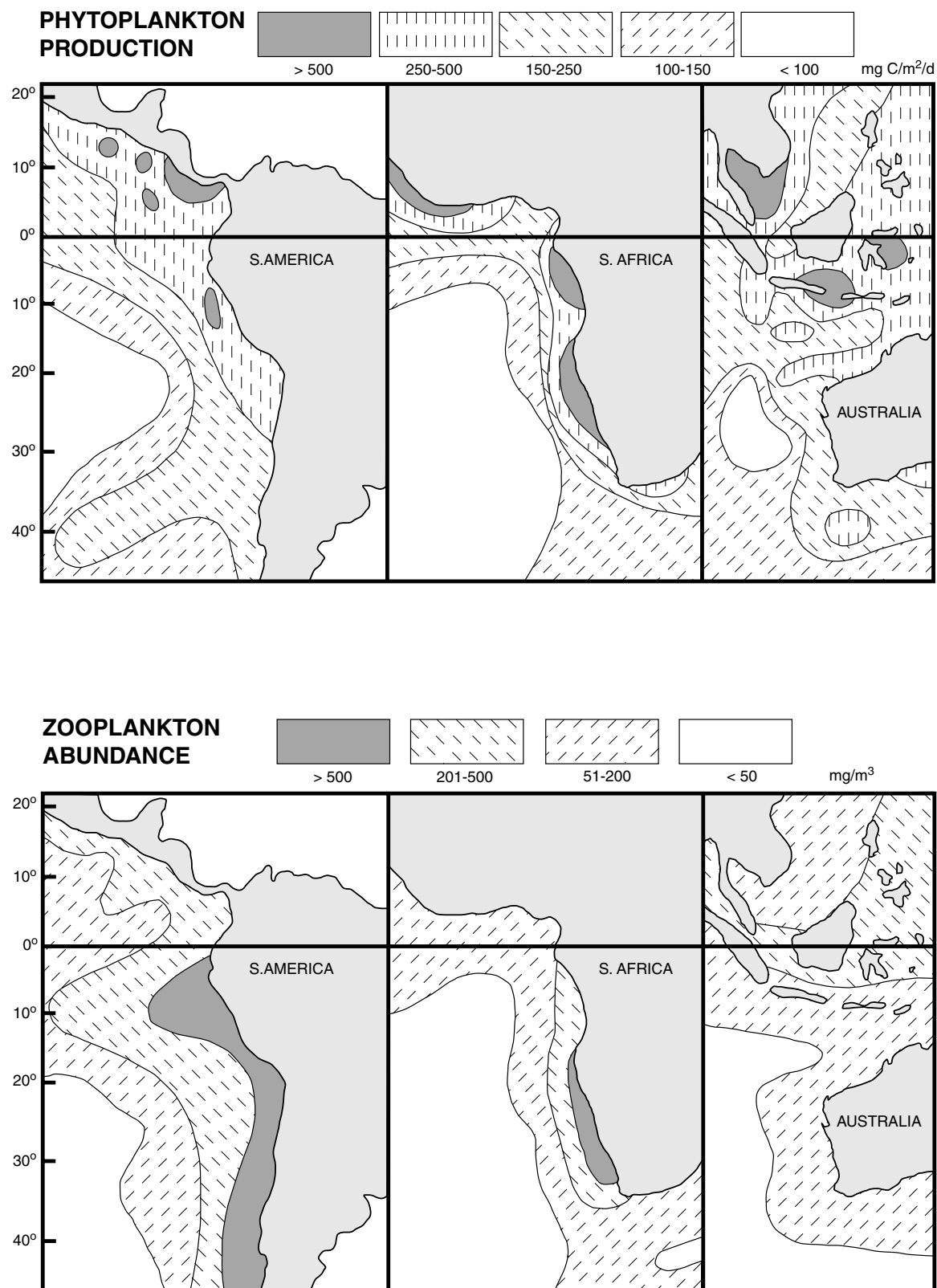
Figure 2 Phytoplankton production ( \text{mg C/m}^2/\text{day} ) (upper panel) and zooplankton abundance ( \mu\text{g/L} ) (lower panel) off the west coasts of South America, South Africa and Western Australia. After Pearce (1991), adapted from FAO (1981).
