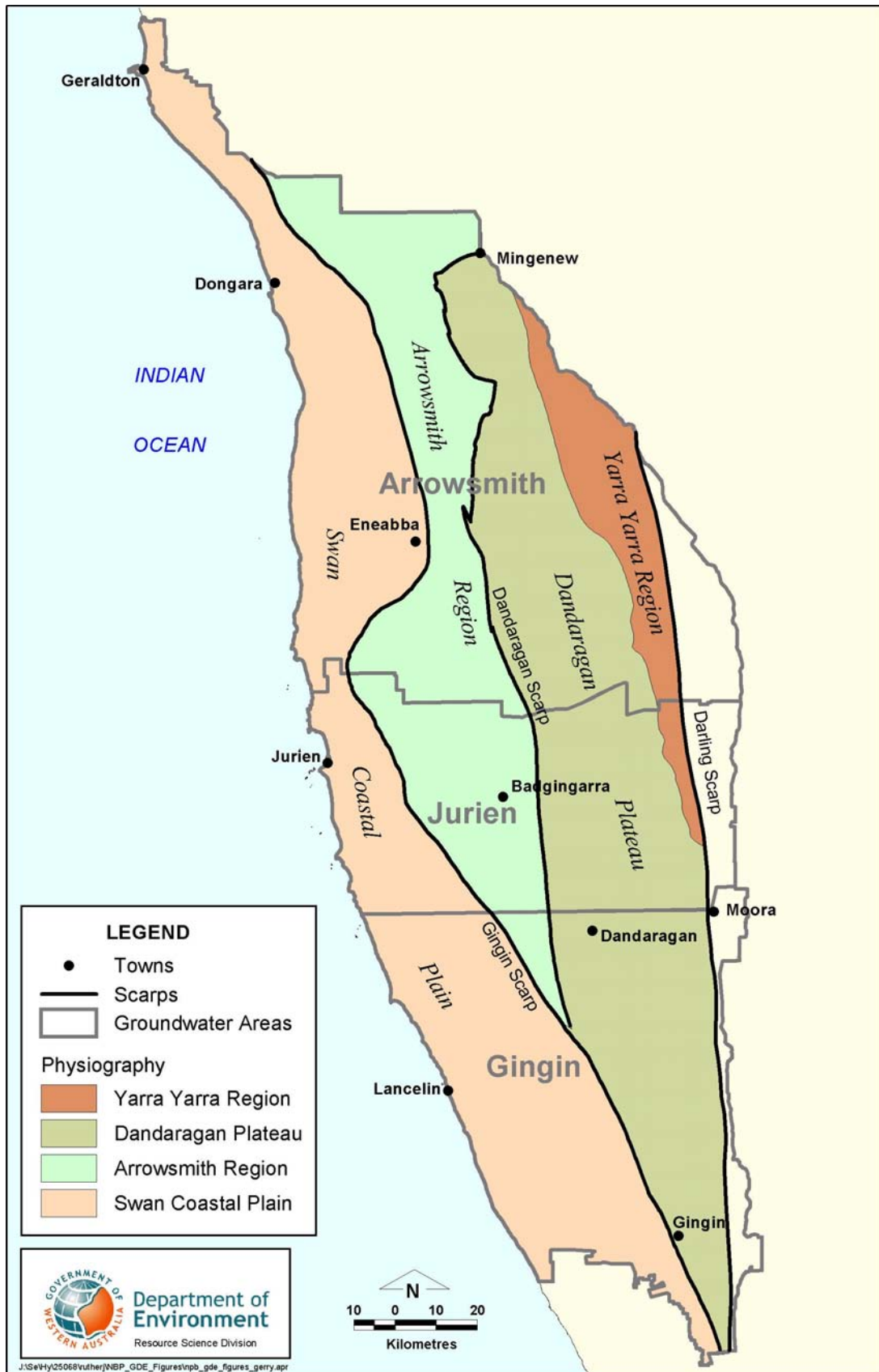
Figure 2: Physiography; major perennial and ephemeral watercourses
