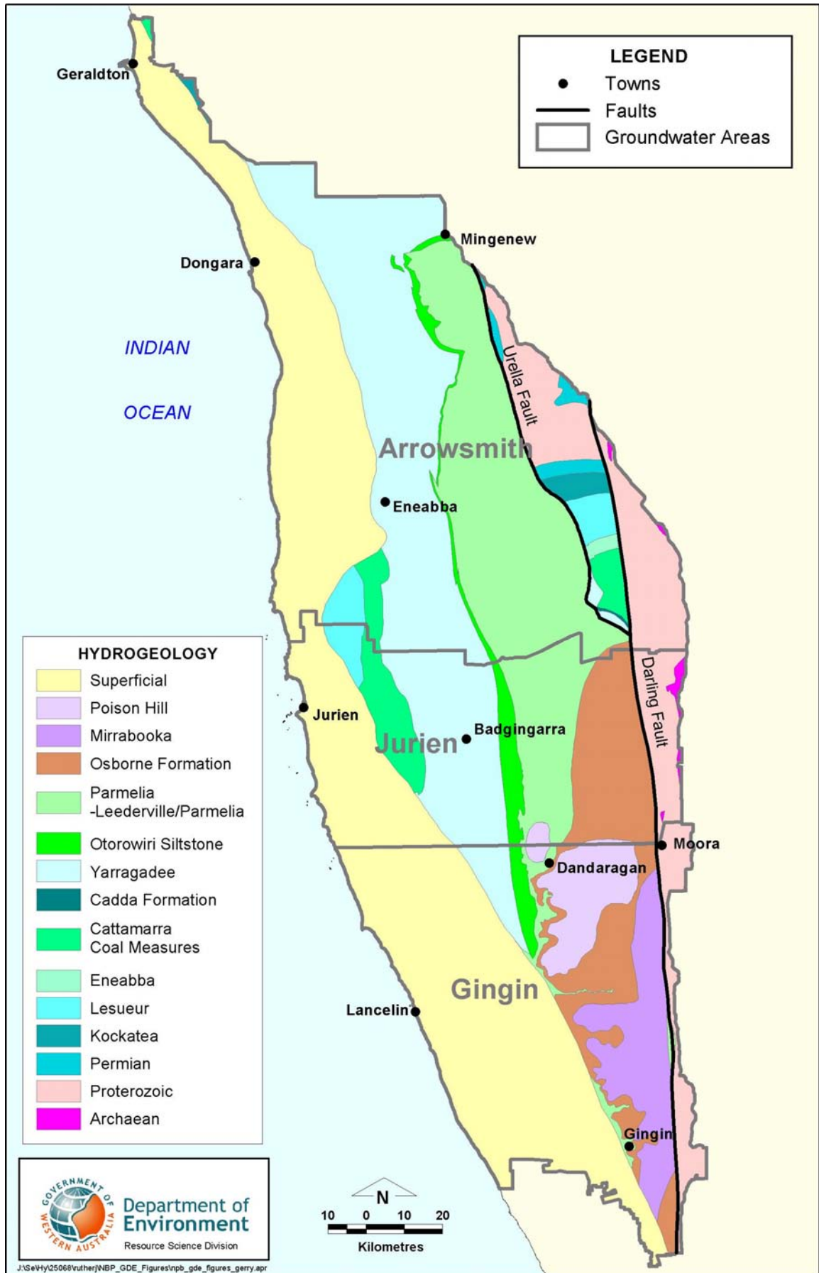
Figure 3: Hydrogeology of the Northern Perth Basin
