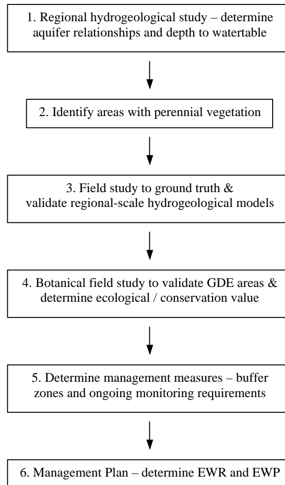
Figure 5: A technical approach for identifying GDEs
