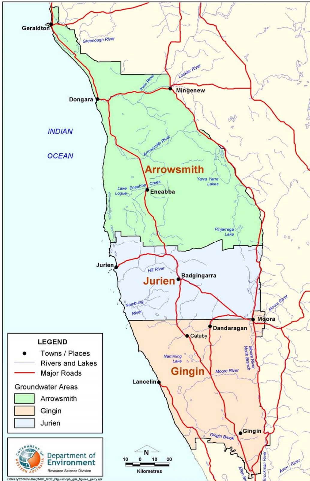
Figure 1: Study area; major groundwater management areas
