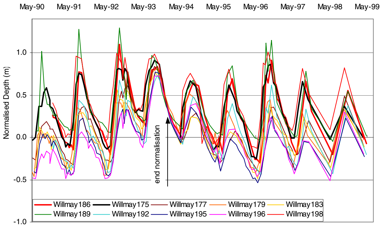
Figure A3.5 Normalised piezometer records from Willmay
