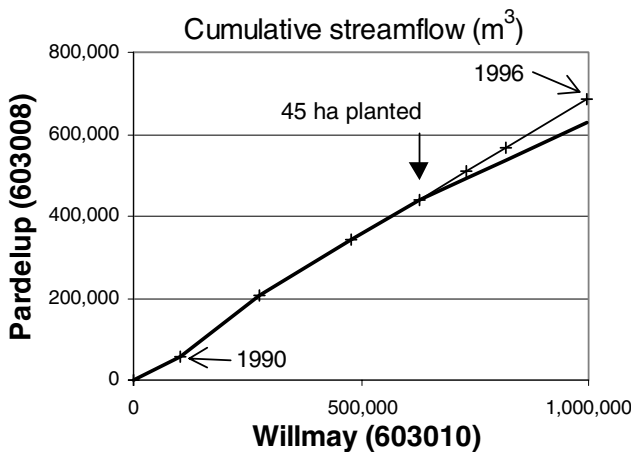
Figure 16. Double mass curves — Pardelup compared with Willmay
