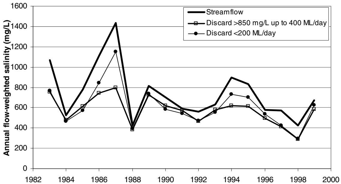
Figure 30. Effect on salinity of using the criteria for diversion to achieve 1983–99 mean of 500 mg/L
