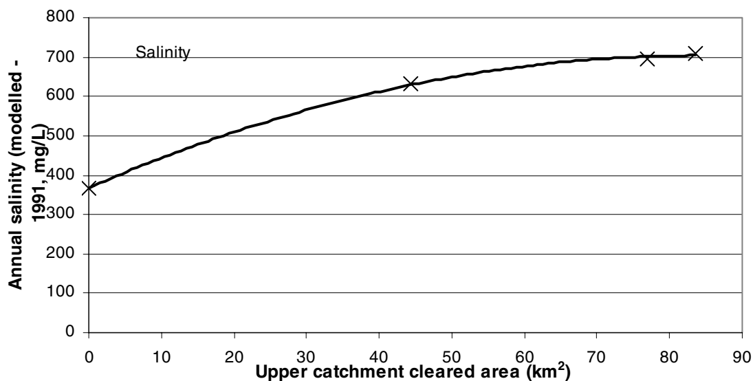
Figure 27. Modelled stream salinity for Denmark River at Mt Lindesay
