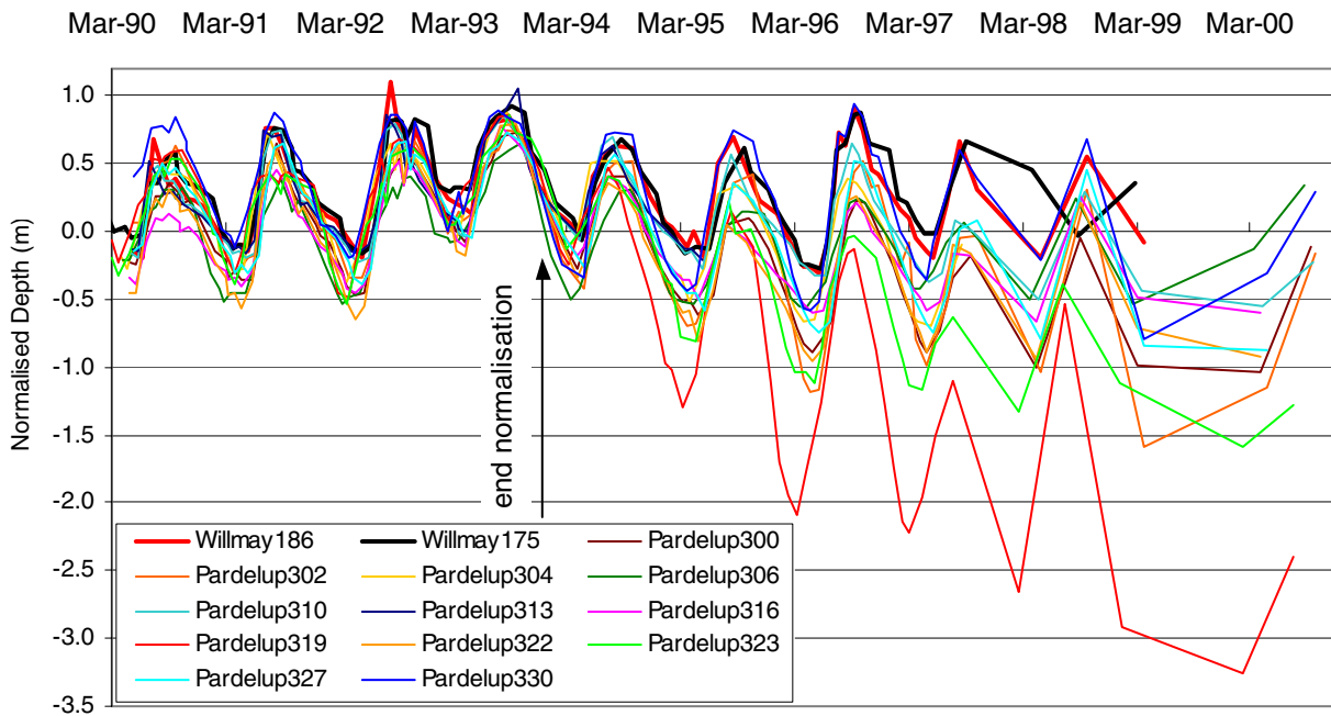
Figure A3.1 Normalised piezometer records from Pardelup compared with selected Willmay piezometers
