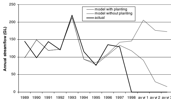
Figure A4.7 Barrama actual and modelled annual flows (Sept–Aug)
