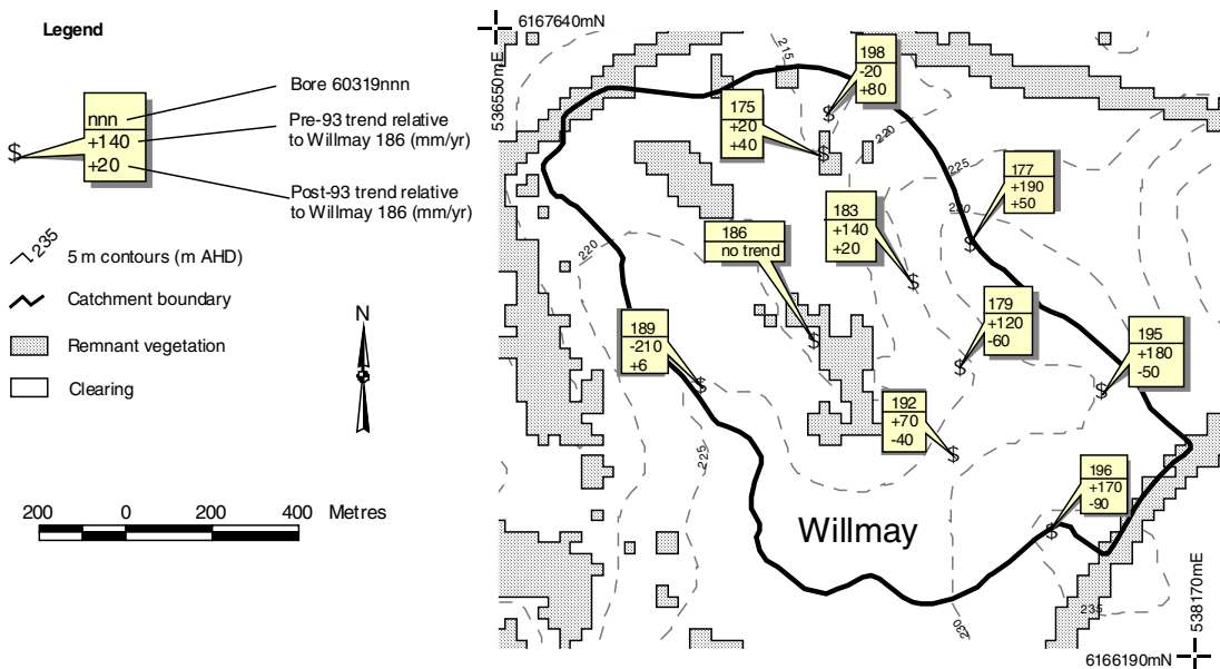
Figure 18. Willmay piezometer trend
