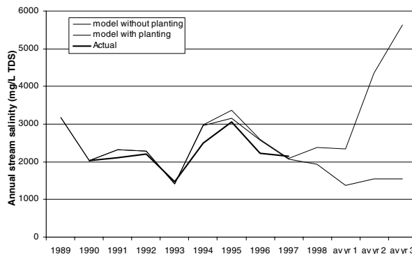
Figure A4.9 Barrama actual and modelled flow-weighted salinity (Sept–Aug)
