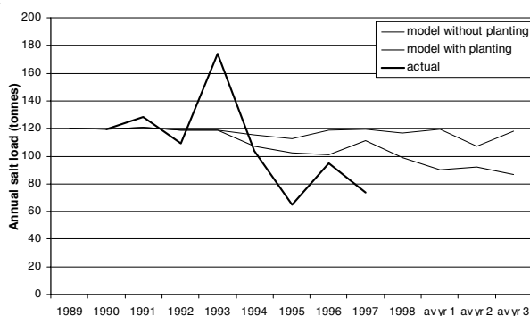
Figure A4.3 Pardelup actual and modelled annual salt load (Sept–Aug)
