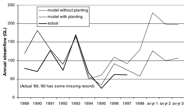
Figure A4.2 Pardelup actual and modelled annual flows (Sept–Aug)
