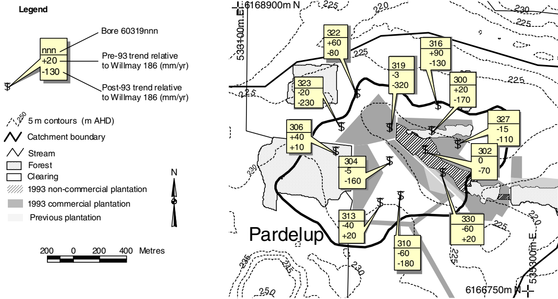
Figure 19. Pardelup piezometer trend
