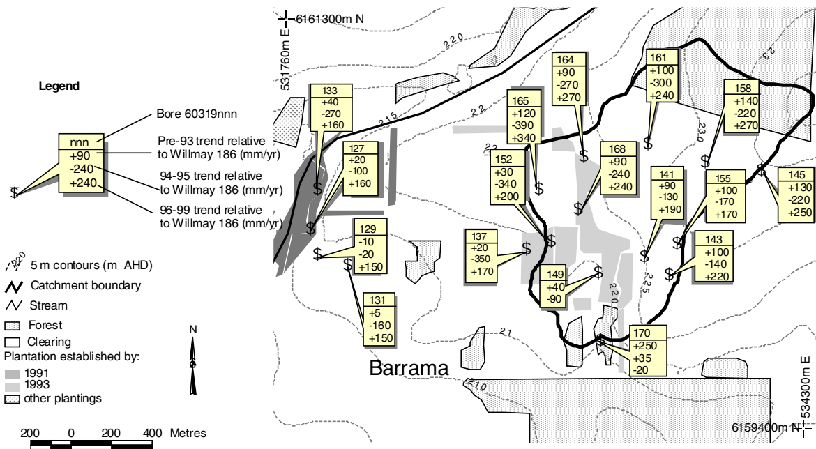
Figure 20 Barrama piezometer trend
