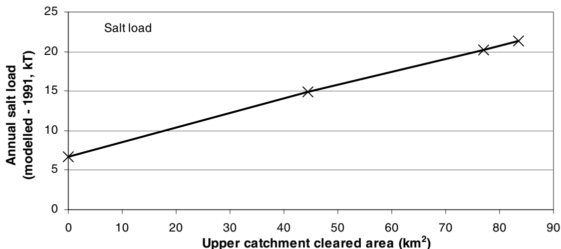
Figure 28. Modelled salt load for Denmark River at Mt Lindesay
