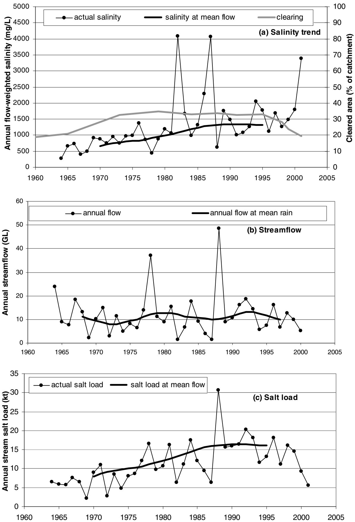
Figure 13b. Stream salinity trend of the Denmark River at the Kompup gauging station
