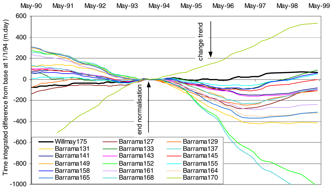
Figure A3.4 Accumulated differences of normalised piezometer records from Willmay 186 (Barrama)
