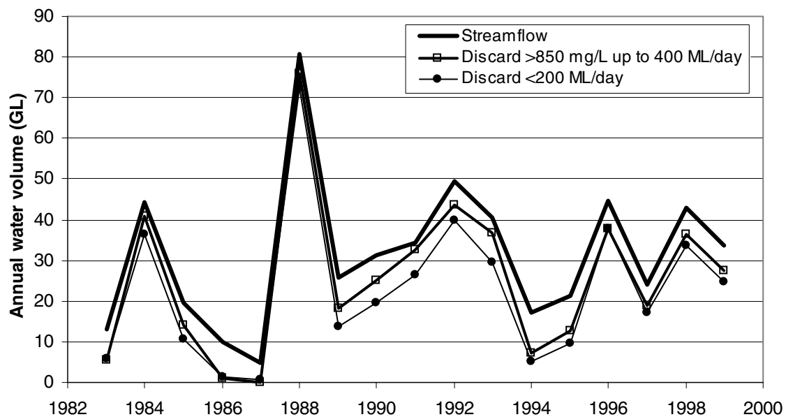
Figure 31. Effect on water volume of using the criteria for diversion to achieve 1983–99 mean of 500 mg/L
