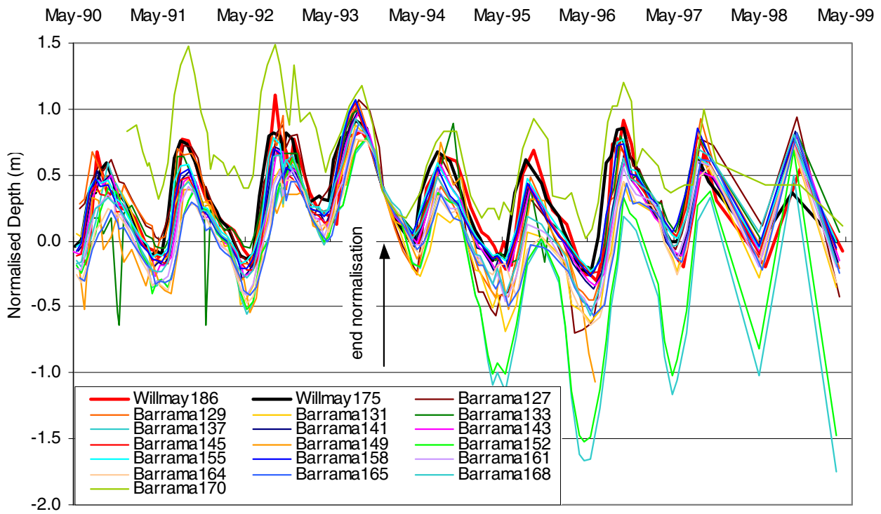
Figure A3.3 Accumulated differences of normalised piezometer records from Willmay 186 (Barrama)
