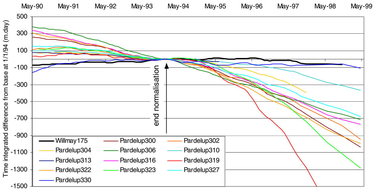
Figure A3.2 Accumulated differences of normalised piezometer records from Willmay 186 (Pardelup)
