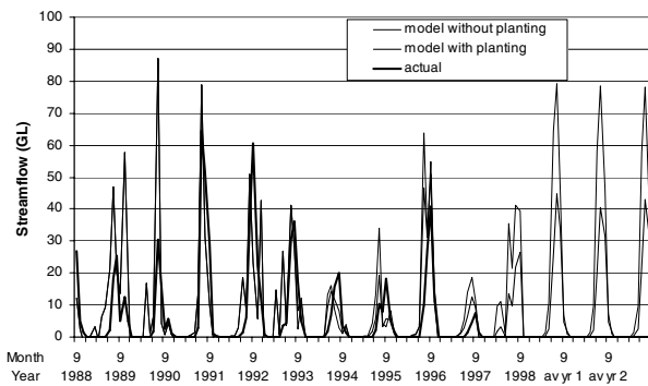
Figure A4.1 Pardelup actual and modelled monthly streamflows
