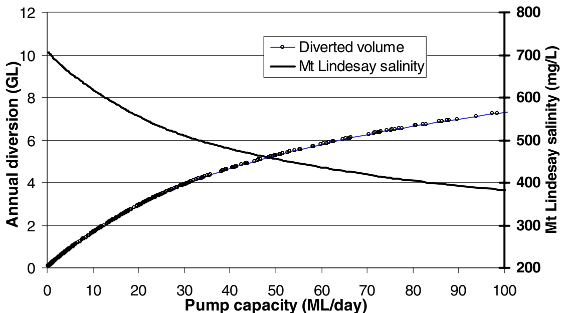
Figure 32. Effect of diverting water at the Kompup gauging station on mean salinity at the Mt Lindesay gauging station
