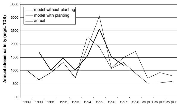
Figure A4.4 Pardelup actual and modelled flow-weighted salinity (Sept–Aug)
