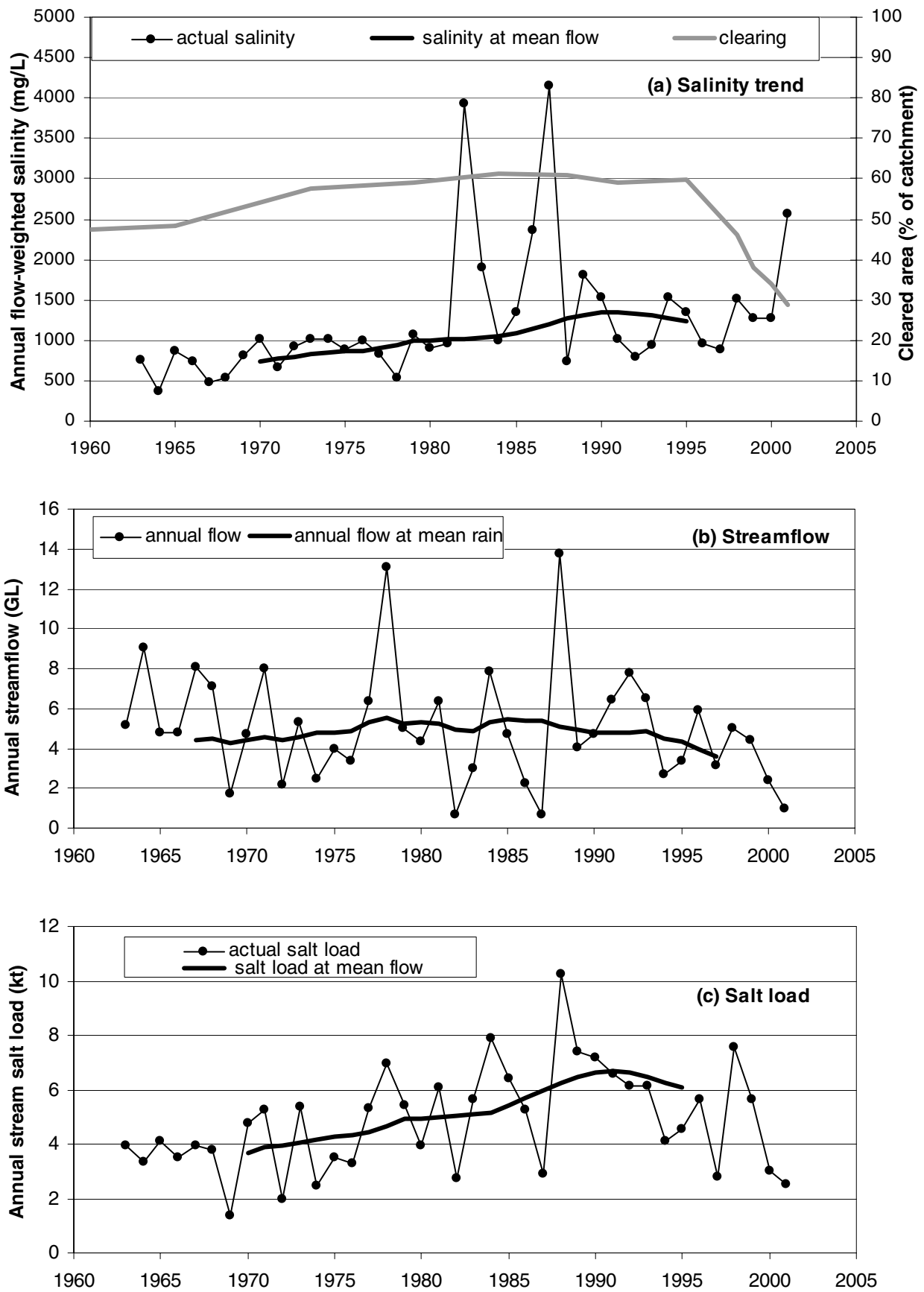
Figure 13c. Stream salinity trend of the Denmark River at the Yate Flat Creek gauging station
