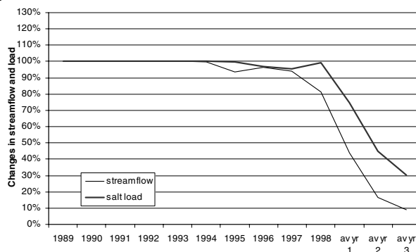
Figure A4.10 Barrama change in modelled flow and salt load with planting
