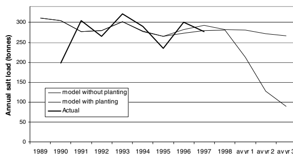
Figure A4.8 Barrama actual and modelled annual salt loads (Sept–Aug)
