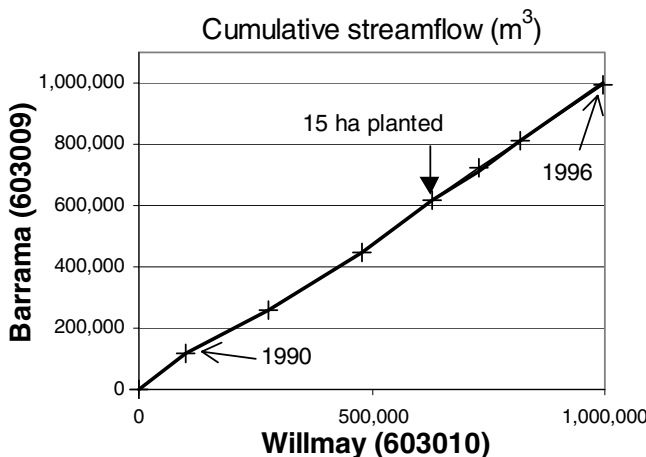
Figure 17. Double mass curves — Barrama compared with Willmay
