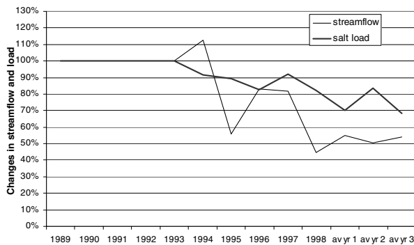
Figure A4.5 Pardelup change in modelling flow and salt load with planting
