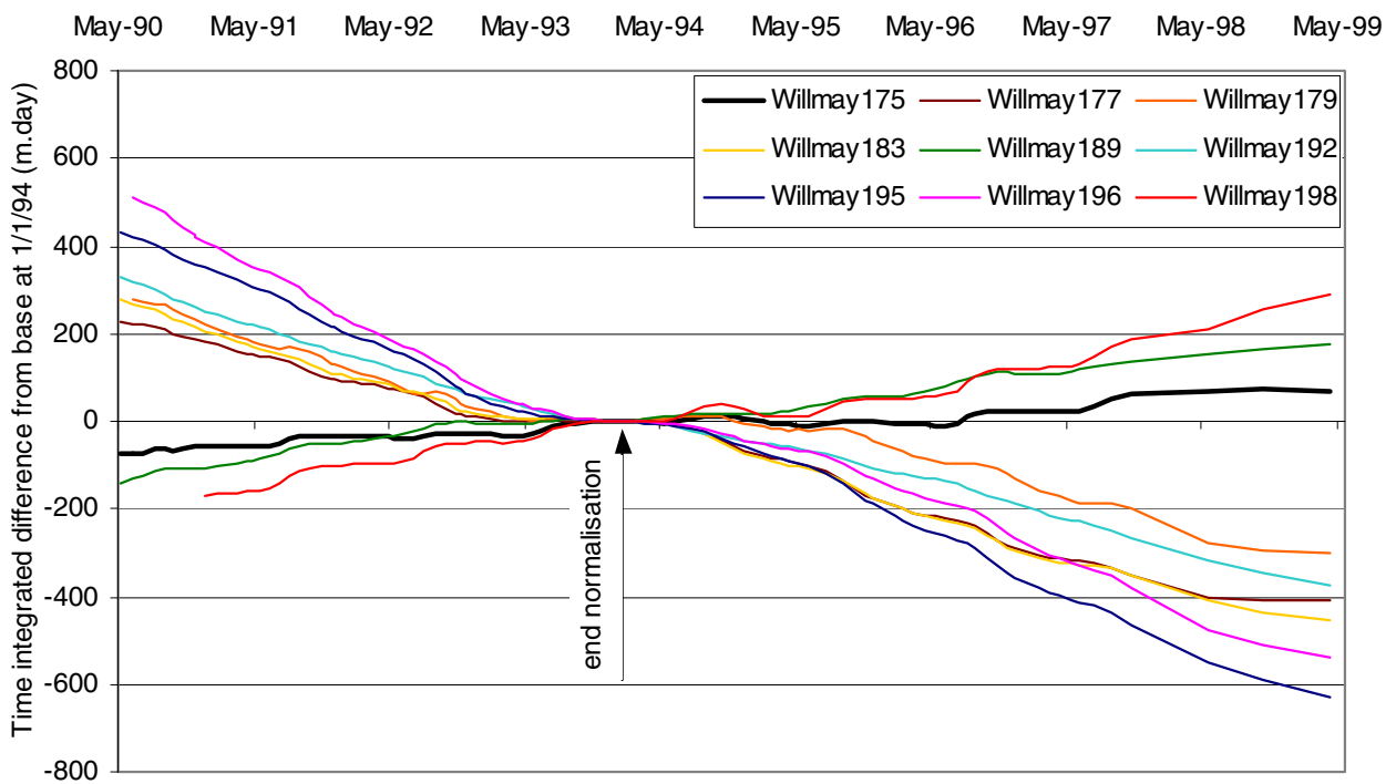
Figure A3.6 Accumulated differences of normalised piezometer records from Willmay 186 (Willmay)
