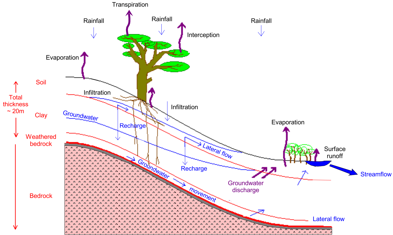
Figure 21 Representation of hydrological processes used in MAGIC model
