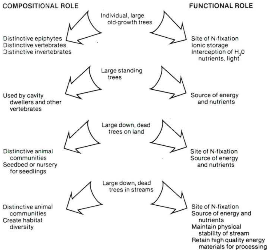
Figure 9. Most of the special habitat and ecosystem functions of old-growth conifer forests can be related to four structural components.
