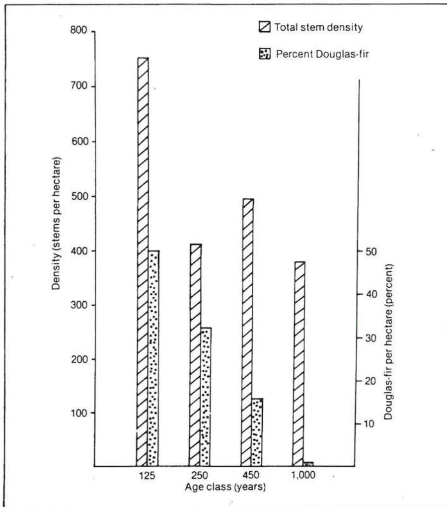
Figure 7. Densities of all trees and Douglas-fir for stands illustrated in figure 6, showing the relatively constant level of density of all trees greater than 2-inch (5-cm) d.b.h. and declining densities of Douglas-fir.
