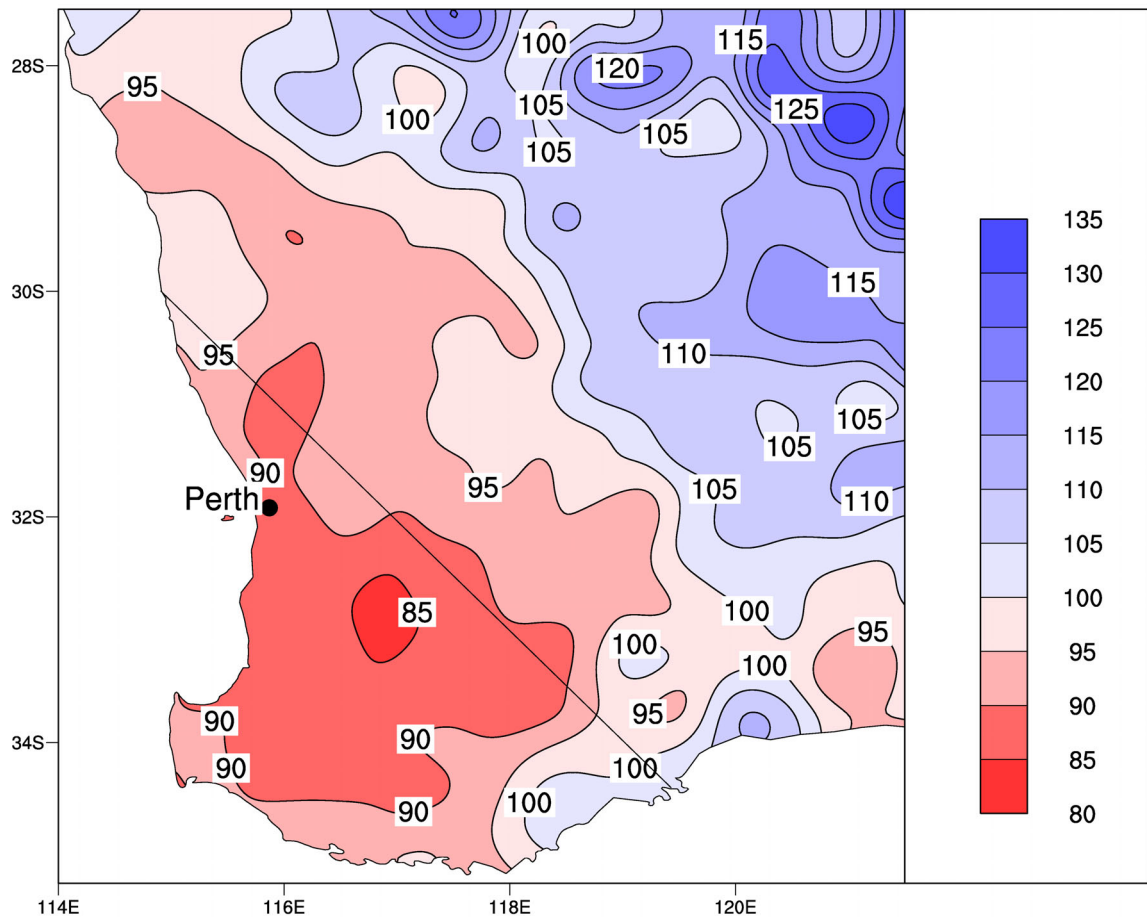
Figure 3. Average May–October rainfall over the 1976–2001 period as a percentage of the average May–October over the 1925–75 period (After IOCI, 2002)
