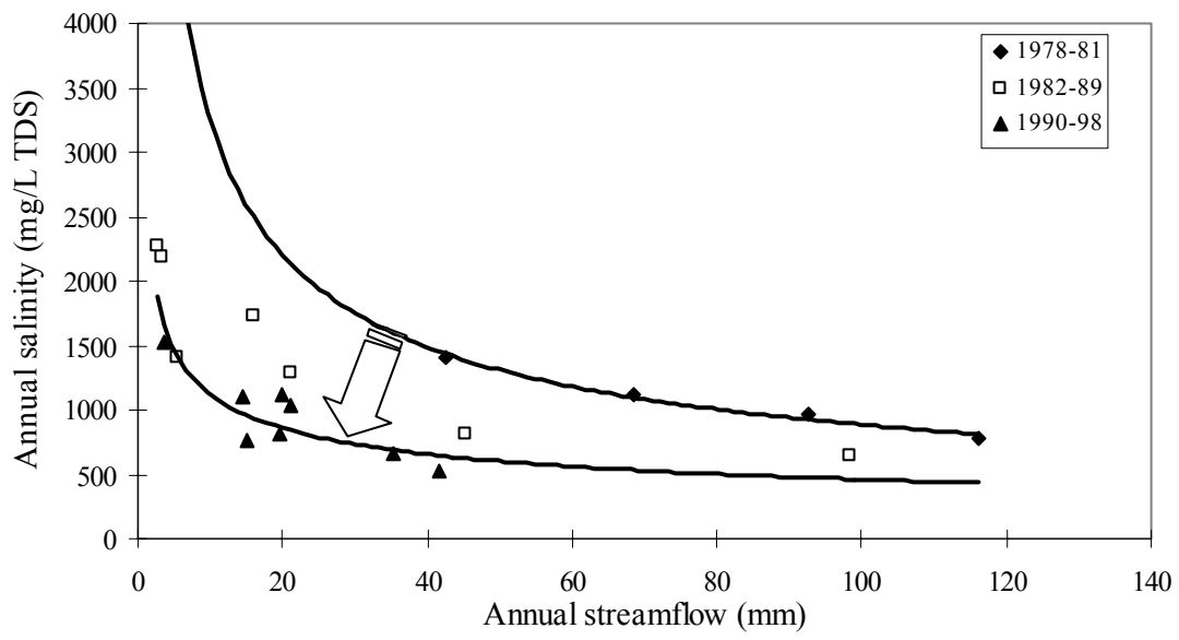
Figure 18. Relationship between annual streamflow and salinity in the Padbury Road catchment
