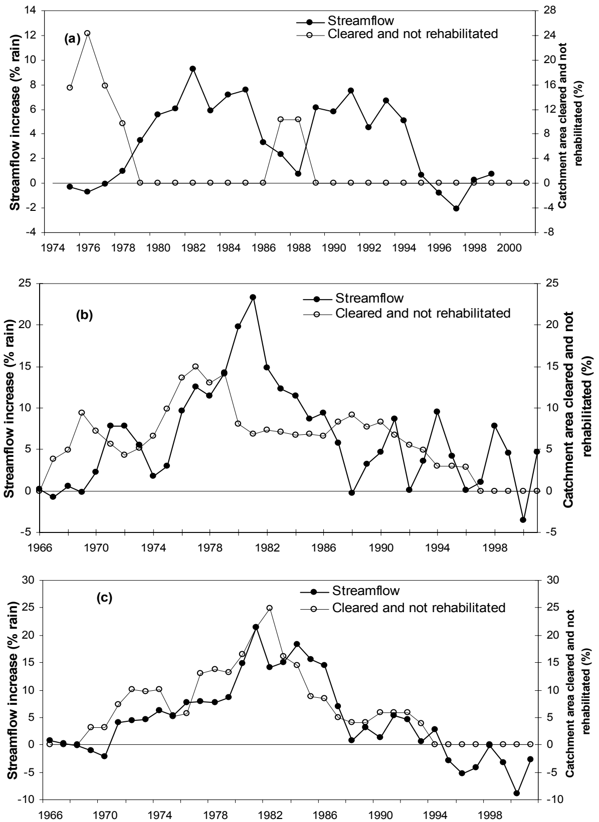
Figure 16. Changes in streamflow following bauxite mining and rehabilitation at (a) Del Park, (b) Seldom Seen and (c) More Seldom Seen catchments
