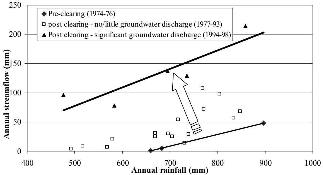
Figure 7. Annual streamflow relationship with rainfall changing with time
