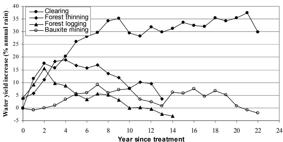
Figure 19. Comparison of water yield responses to land use practices in the High Rainfall Zone
