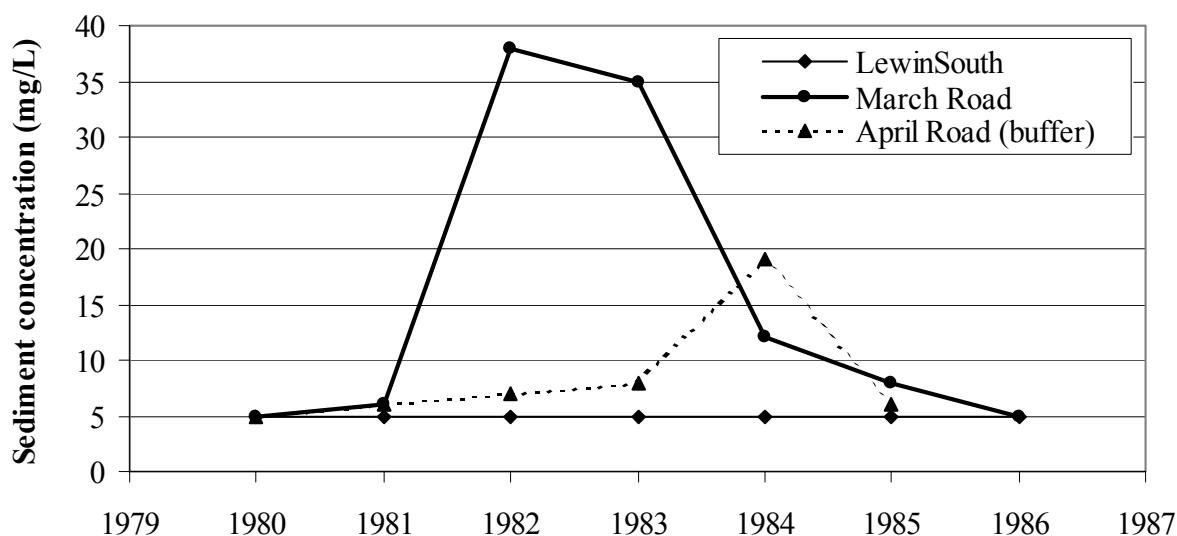
Figure 13. Changes in stream sediment concentration following logging in the Southern Forest
