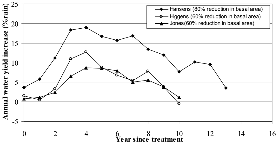
Figure 14. Water yield increases after forest thinning in high rainfall catchments
