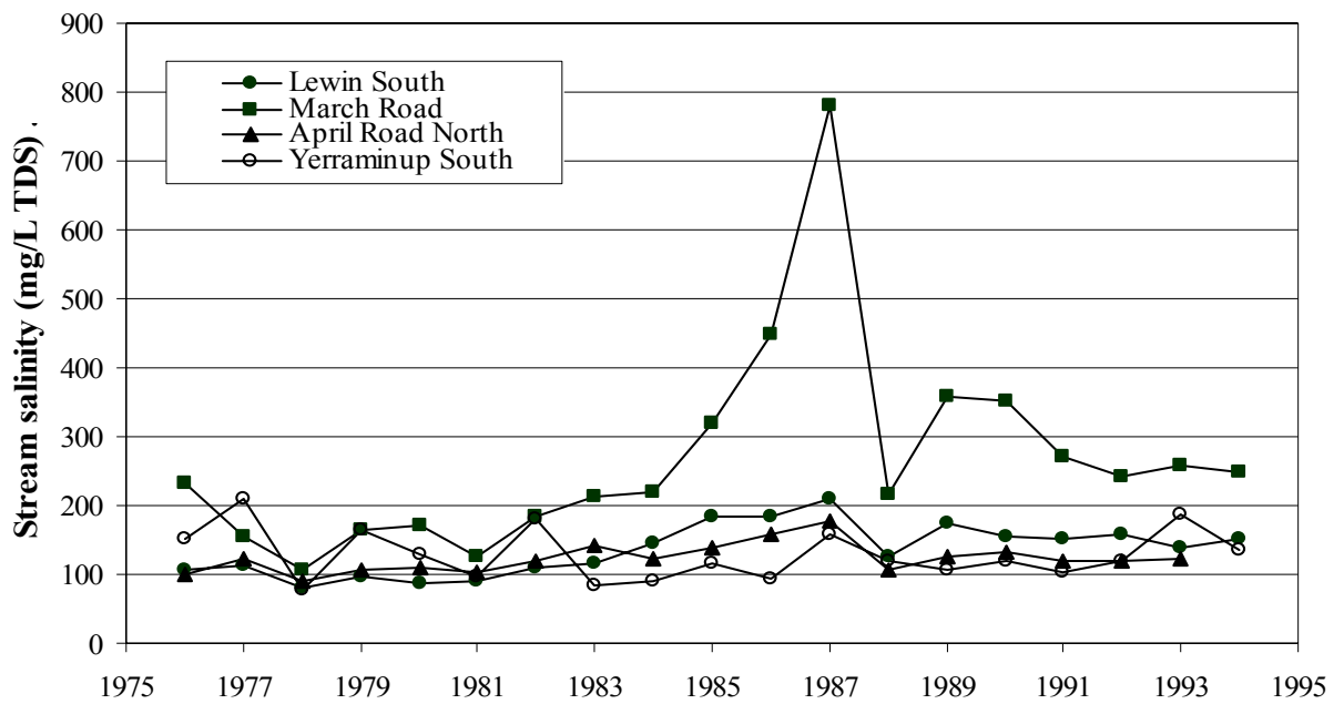
Figure 11. Annual stream salinity of four treated catchments
