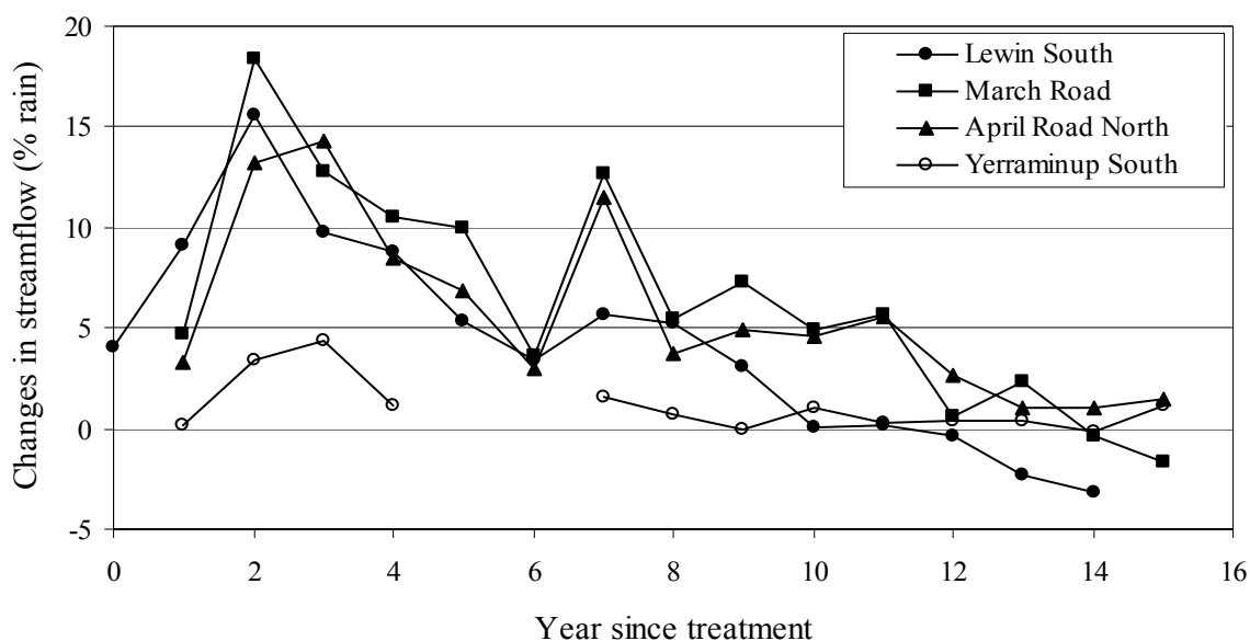
Figure 10. Streamflow response to logging experimental catchments in the Southern Forest
