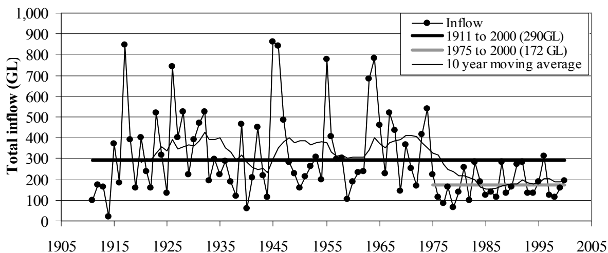
Figure 5. Yearly inflow into Perth water supply reservoirs
