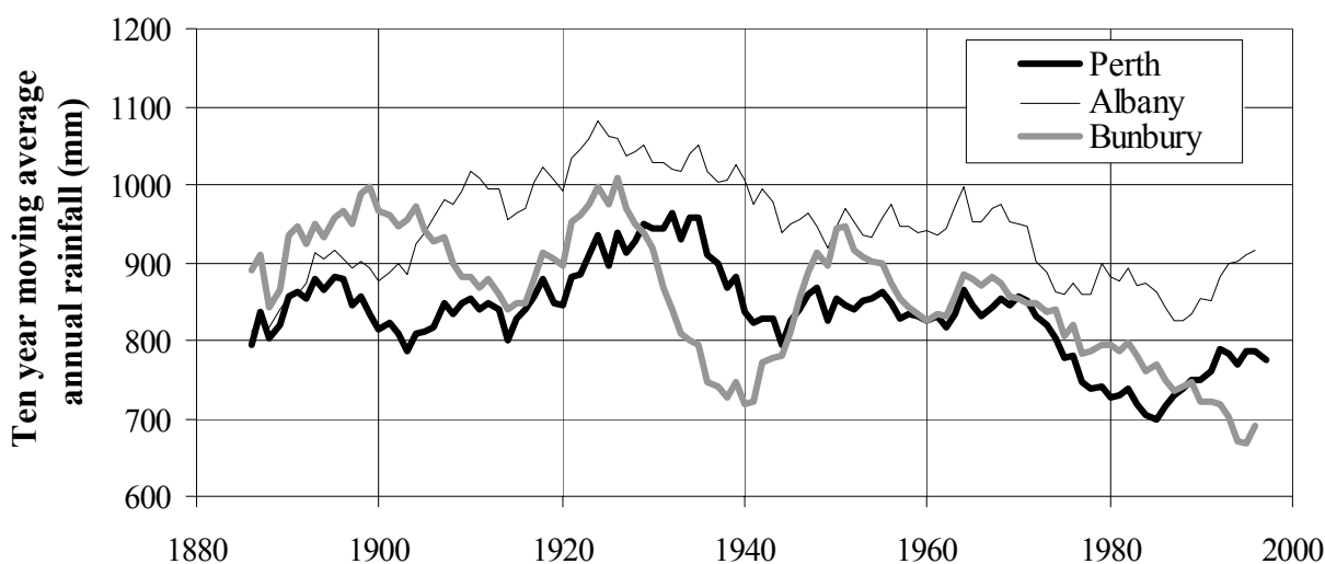
Figure 2. Annual rainfall variability over the last 100 years
