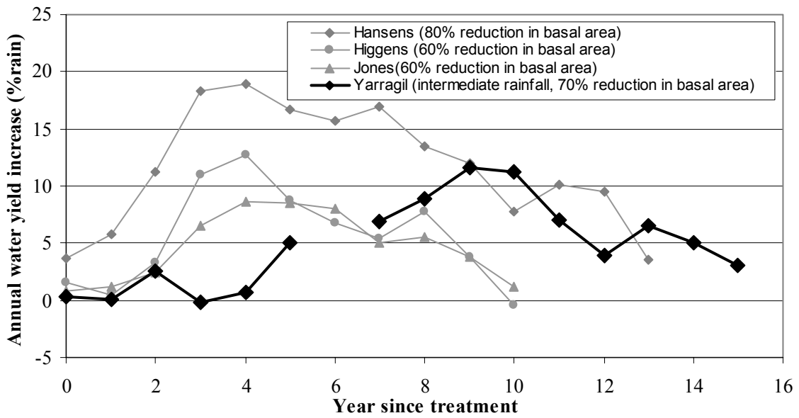
Figure 15. Water yield increases after forest thinning in low rainfall catchments
