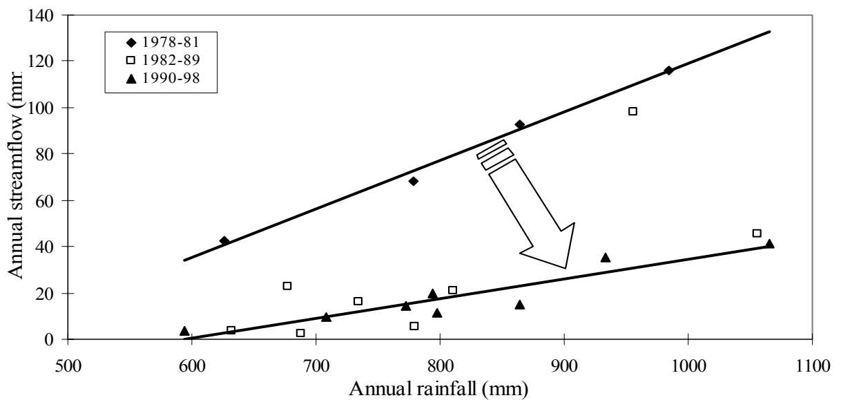
Figure 17. Relationship between annual rainfall and streamflow in the Padbury Road catchment
