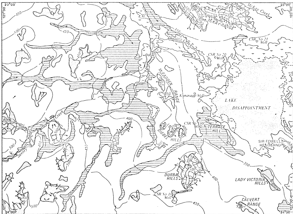
FIGURE 1 PHYSIOGRAPHY AND DRAINAGE GUNANYA SHEET SF 51-14
