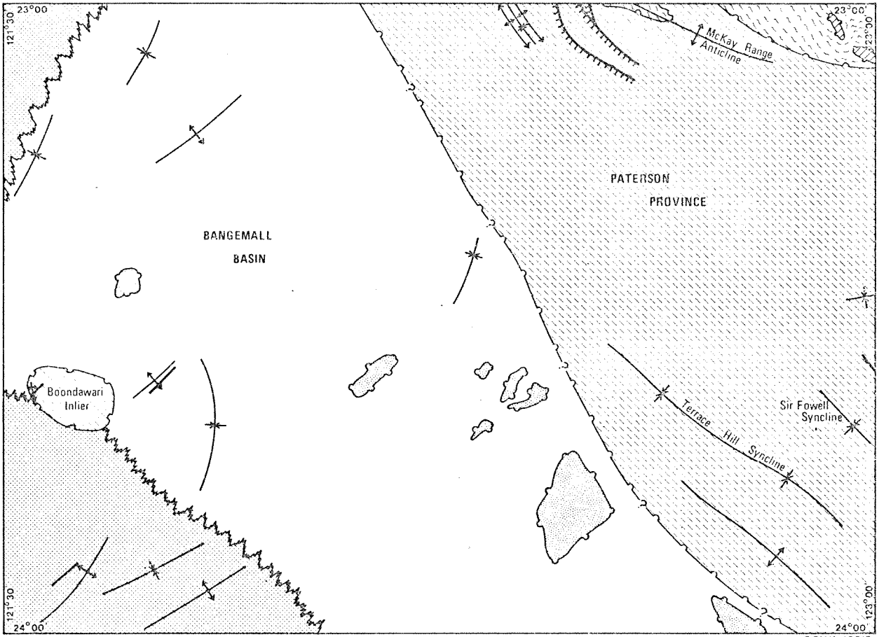
FIGURE 2 STRUCTURAL SKETCH GUNANYA SHEET SF 51-14
