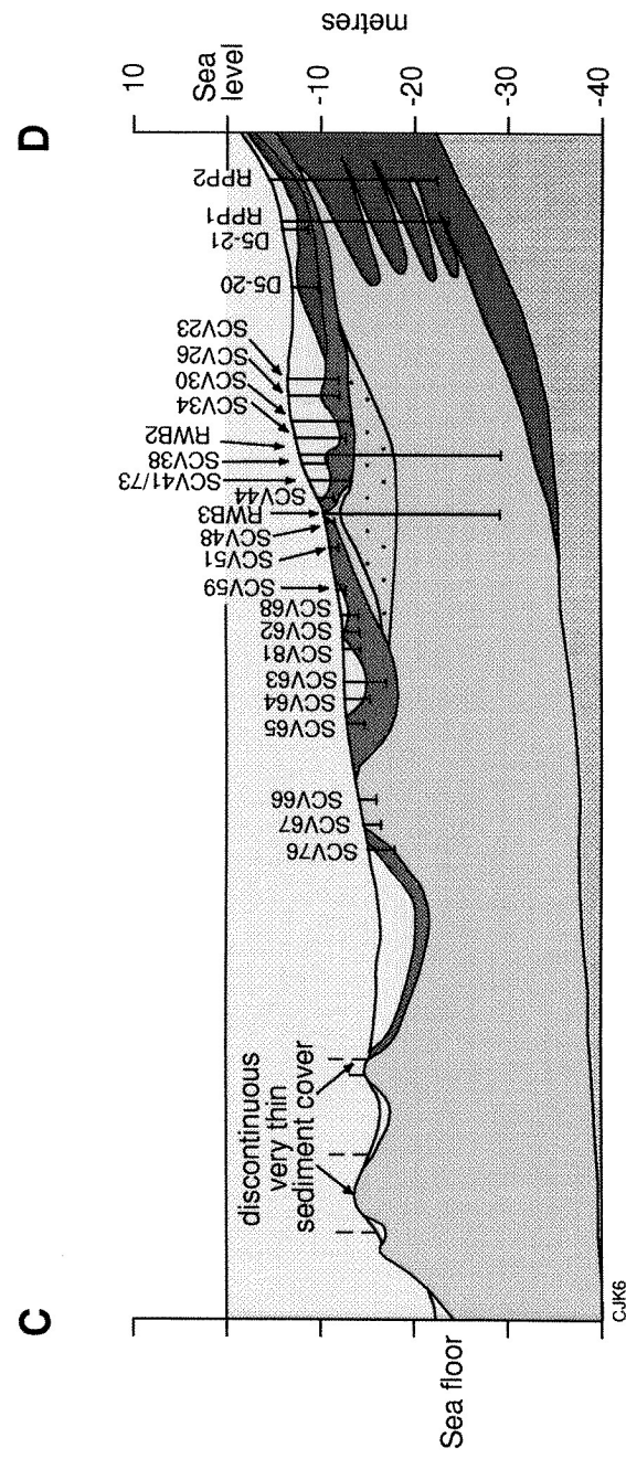
Figure 5. Geological cross sections A–B and C–D Cainozoic geology Mermaid Sound
