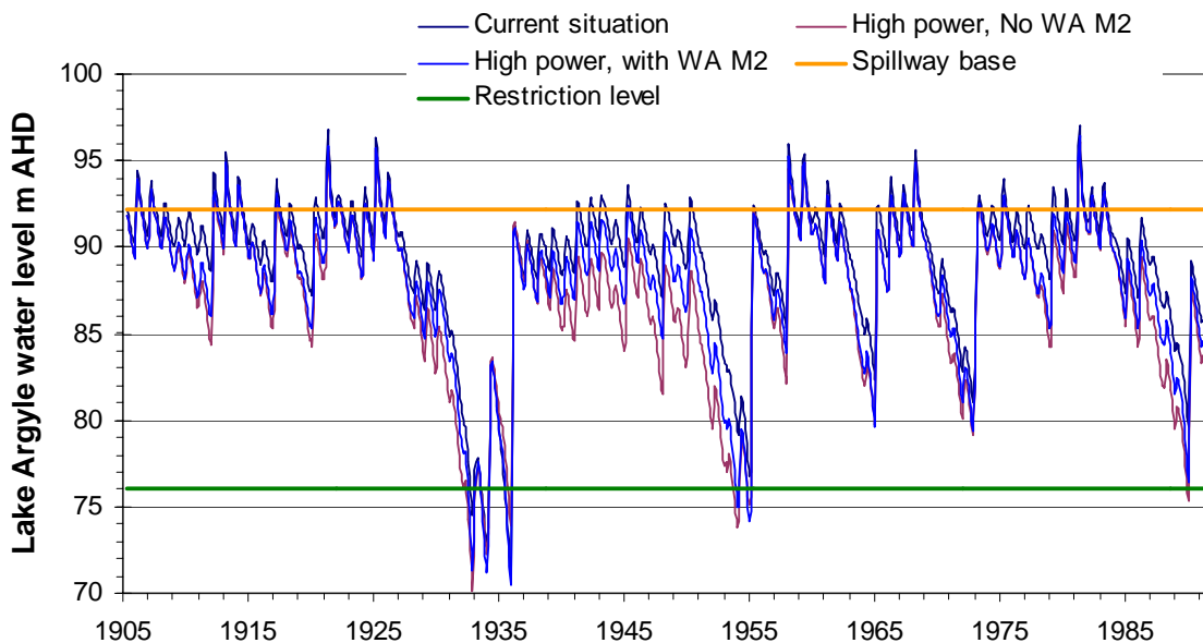
Figure 29 Simulated monthly levels in Lake Argyle under current and proposed allocations
