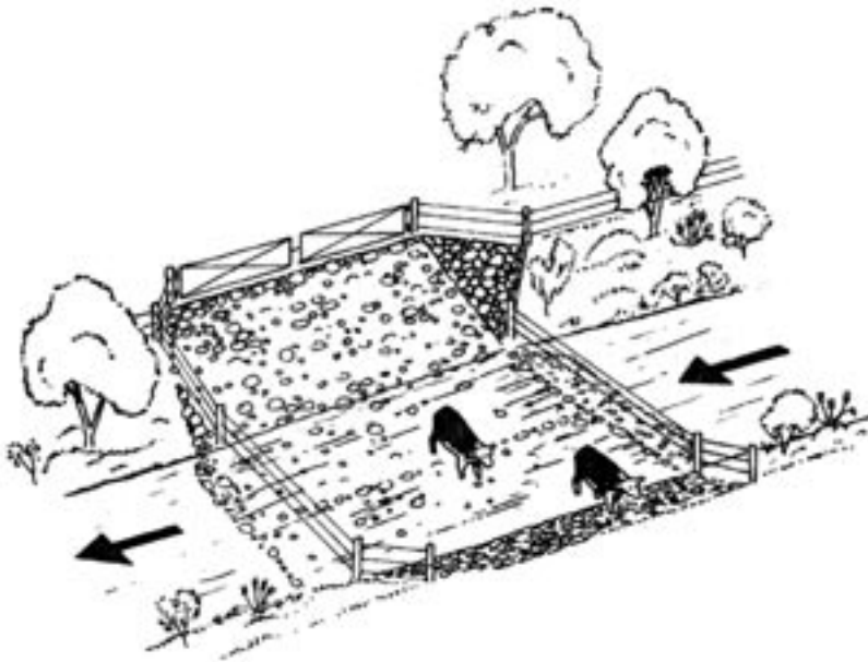
Figure 3 Basic geometry of a livestock crossing (Source: Water and Rivers Commission, 2000b)
