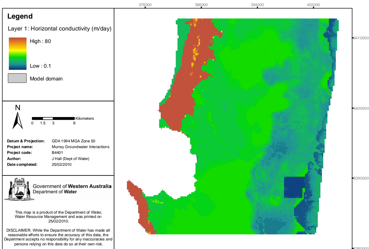
Figure 4-7: Computational layer 1 - horizontal hydraulic conductivity (m/day)
