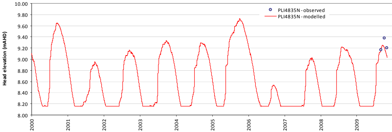
Modelled vs observed time-series plot - PLI4835N
