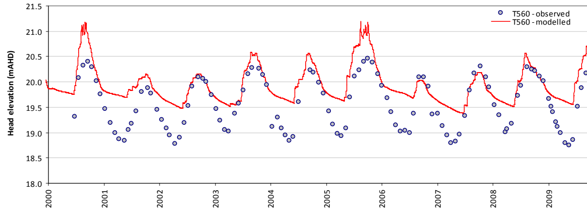
Modelled vs observed time-series plot - T560
