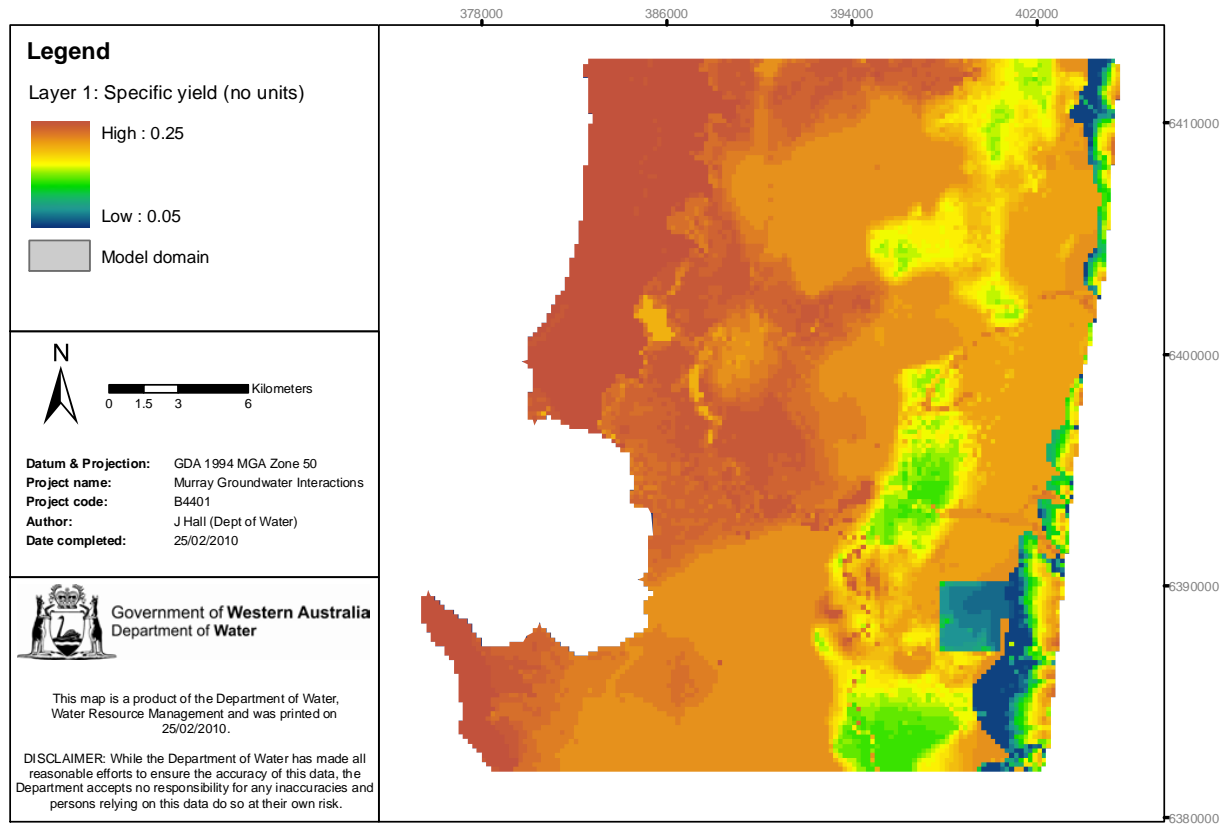
Figure 4-11: Computational layer 1 - specific yield
