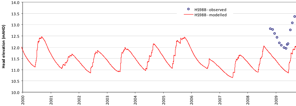
Modelled vs observed time-series plot - HS98B
