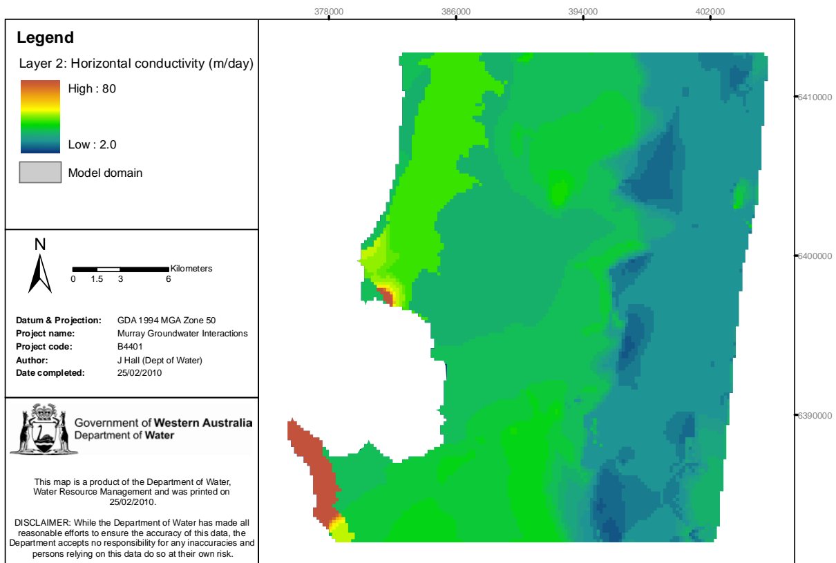
Figure 4-8: Computational layer 2 - horizontal hydraulic conductivity (m/day)
