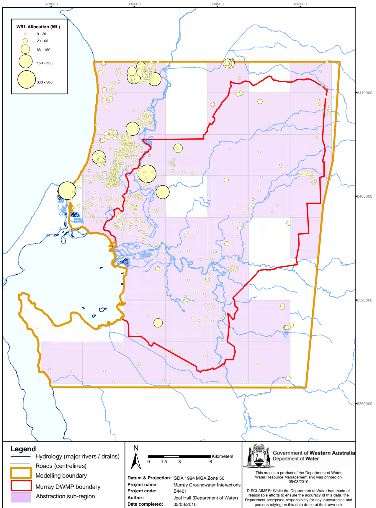
Figure 3-32: Superficial Aquifer abstraction bores and sub-regions
