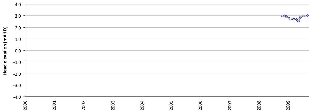
Residual time-series plot - HS105A
