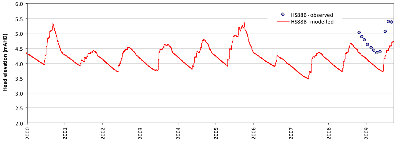
Modelled vs observed time-series plot - HS88B
