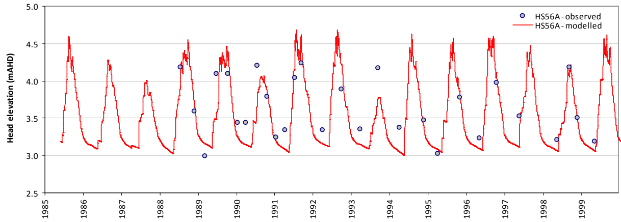
Modelled vs observed time-series plot - HS56A
