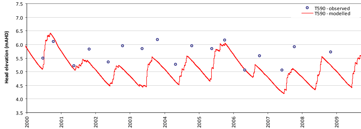
Modelled vs observed time-series plot - T590
