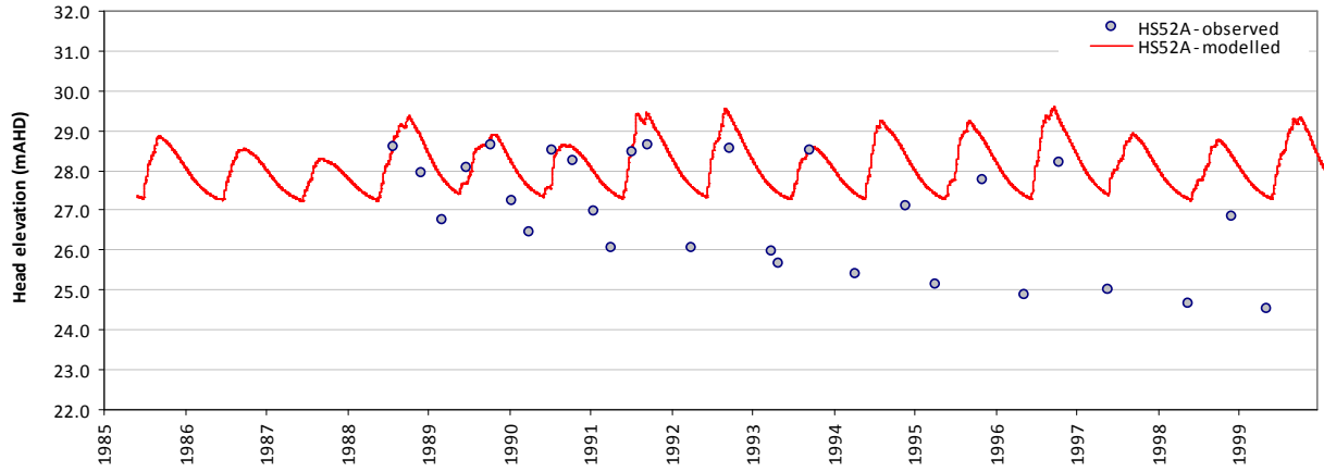
Modelled vs observed time-series plot - HS52A
