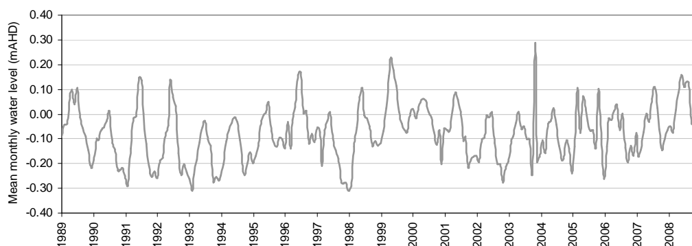
Figure 3-35: Time-varying fixed-head boundary condition on the western boundary of the model
