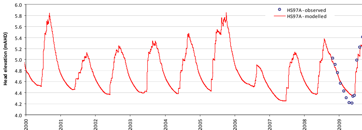
Modelled vs observed time-series plot - HS97A
