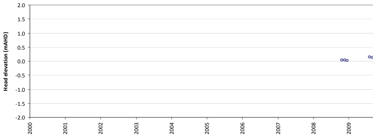
Residual time-series plot - HS101B
