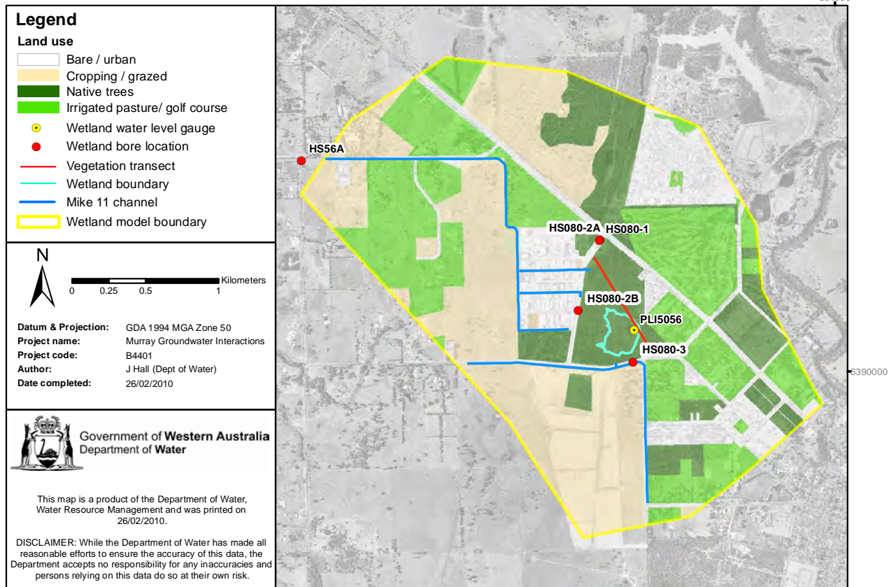
Figure 7-6: Phillips Road model: land use, monitoring and Mike 11 channel locations
