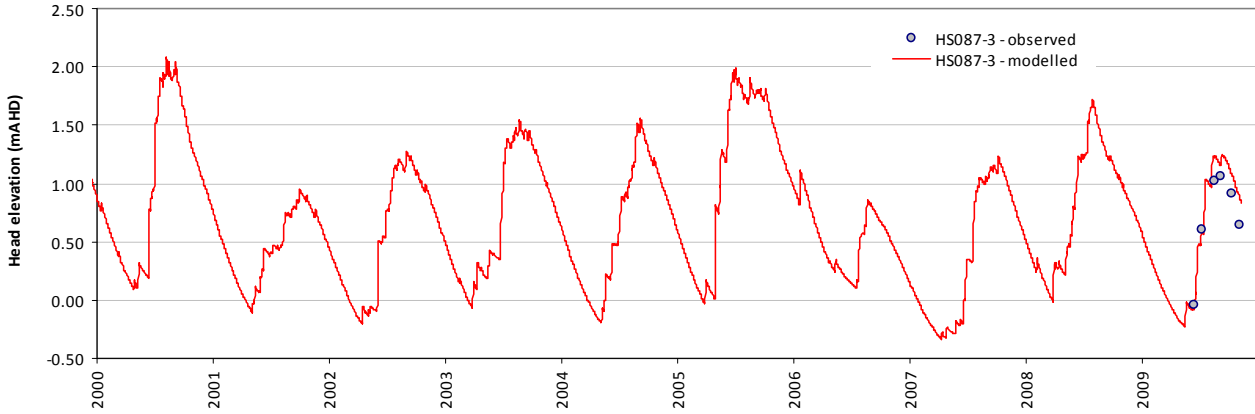
Modelled vs observed time-series plot - HS087-3
