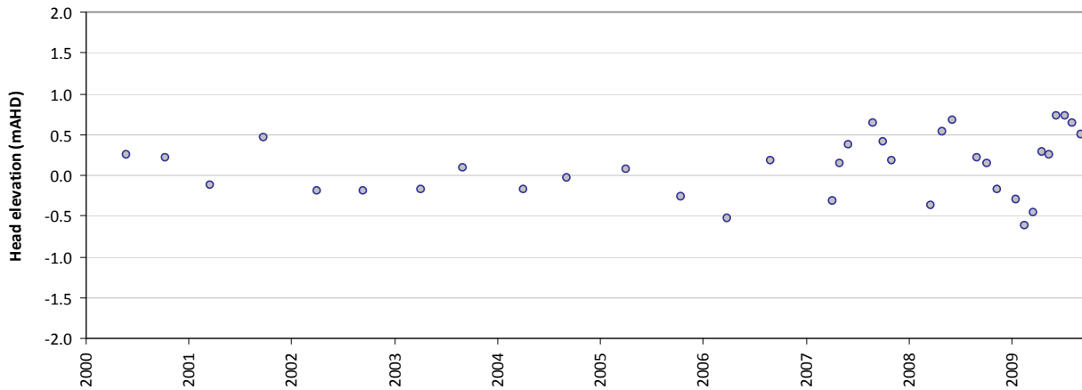
Residual time-series plot - HS56A
