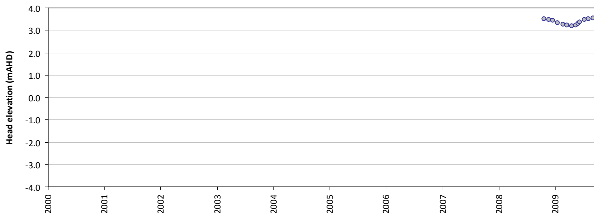
Residual time-series plot - HS105B
