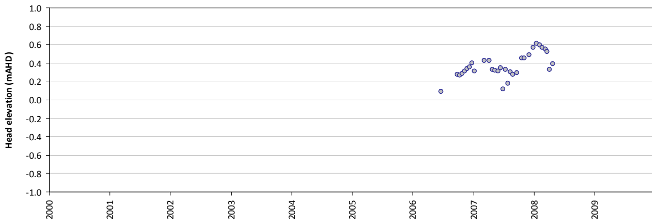
Residual time-series plot - LP17
