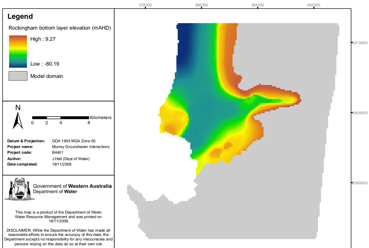
Figure 3-15: Rockingham Sand: base of geological formation (mAHd)
