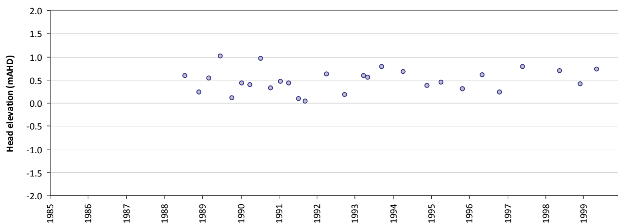
Residual time-series plot - HS55A
