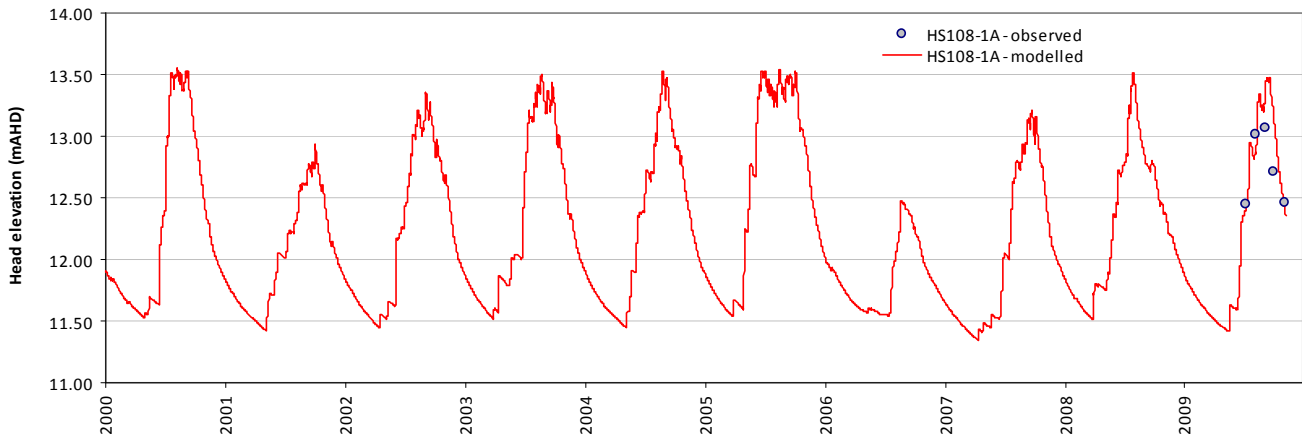
Modelled vs observed time-series plot - HS108-1A
