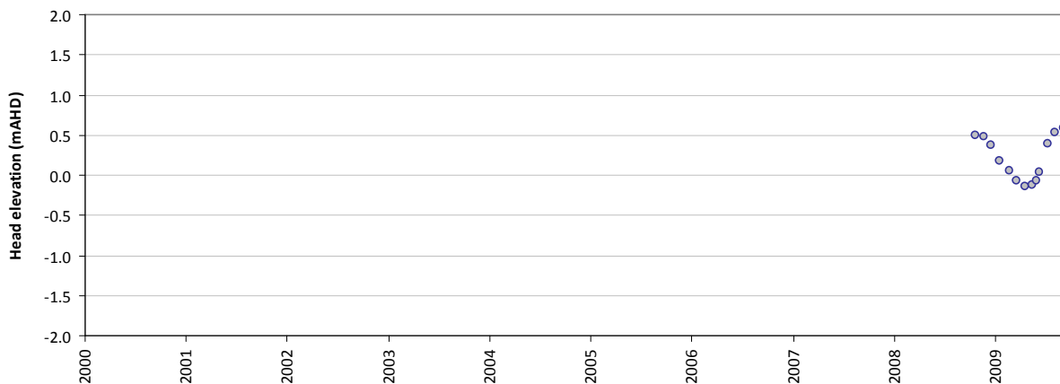
Residual time-series plot - HS106A
