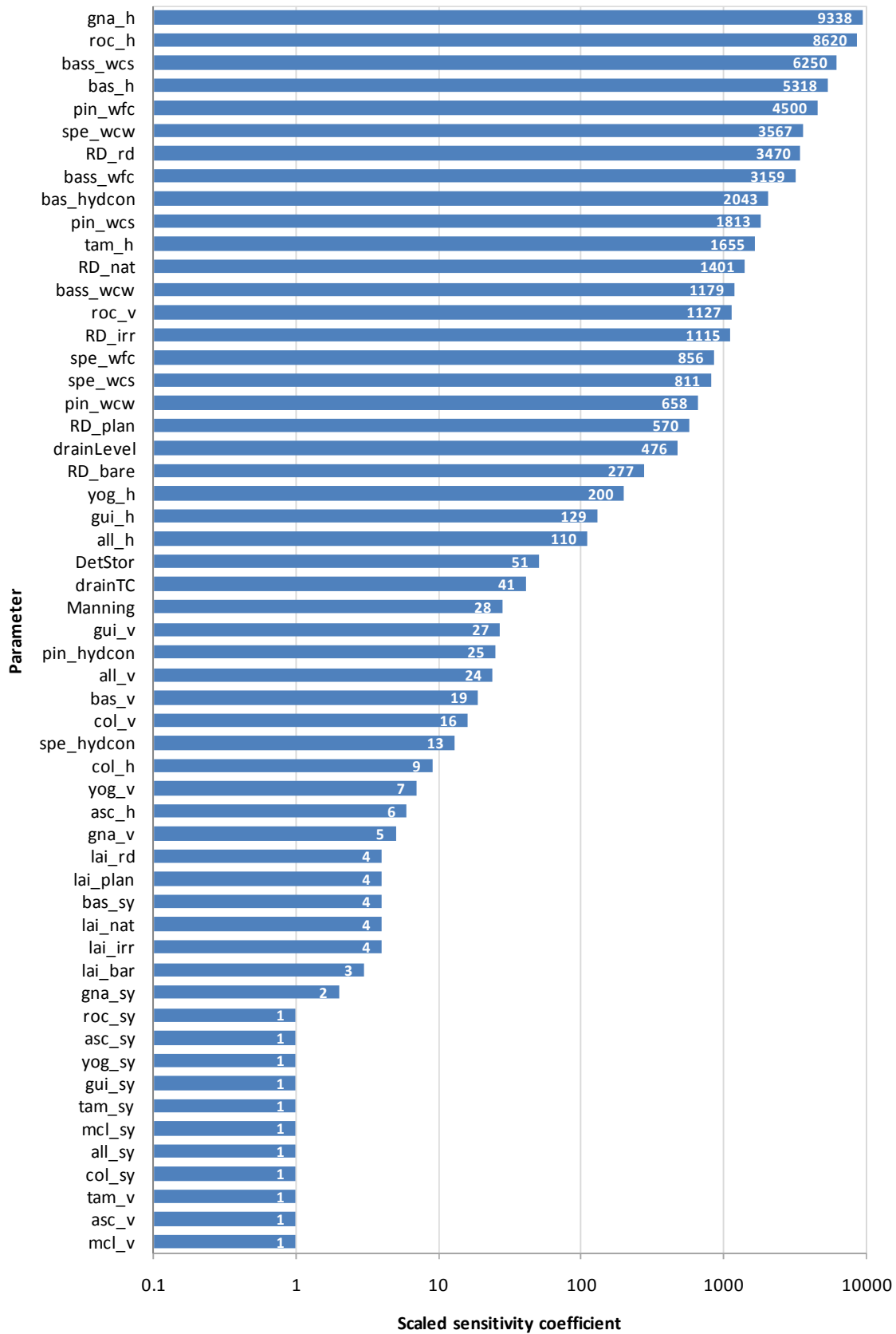
Figure 6-1: Scale sensitivity values resulting from the sensitivity analysis
