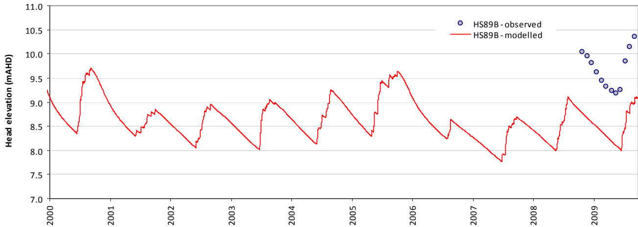
Modelled vs observed time-series plot - HS89B
