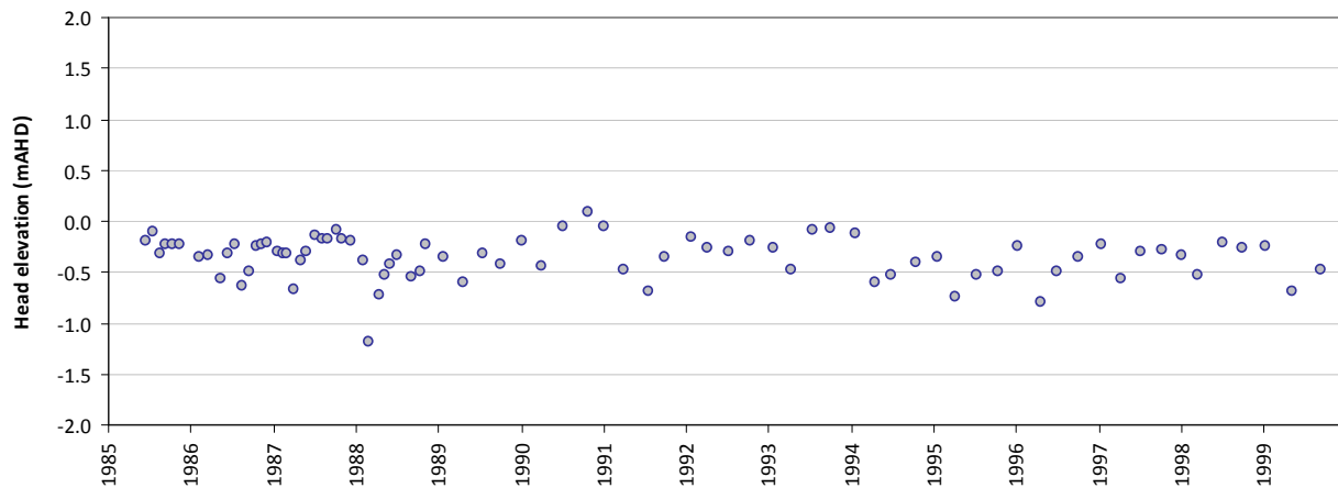
Residual time-series plot - T560
