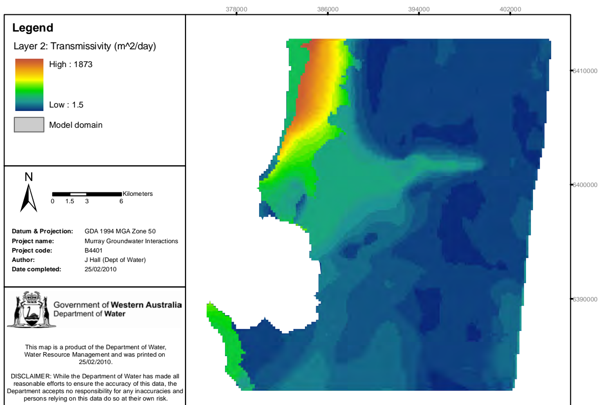
Figure 4-14: Computational layer 2 - transmissivity (m 2 /day)
