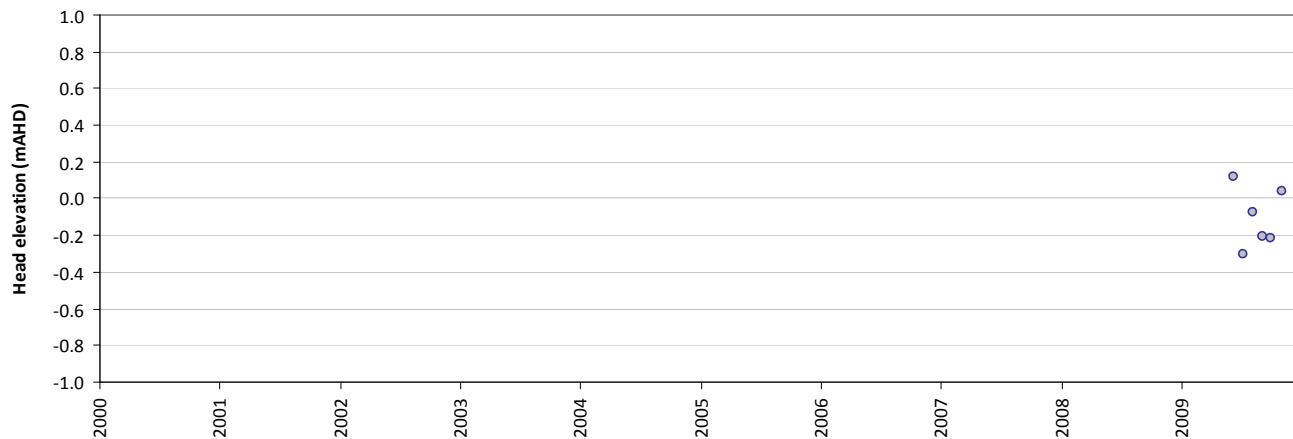
Residual time-series plot - HS109-2
