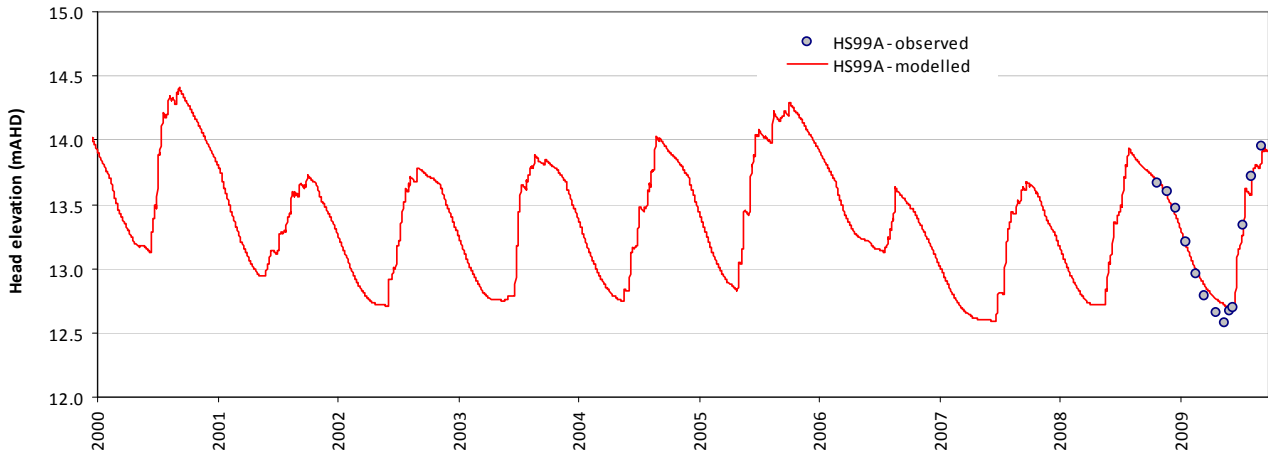
Modelled vs observed time-series plot - HS99A
