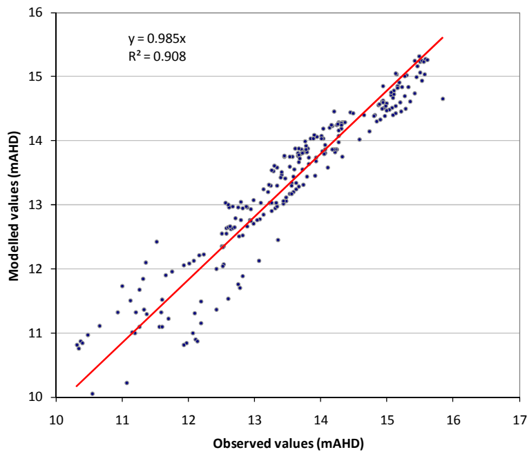
Figure D-1: Scott Road wetland system scatterplot for observed vs modelled groundwater levels
