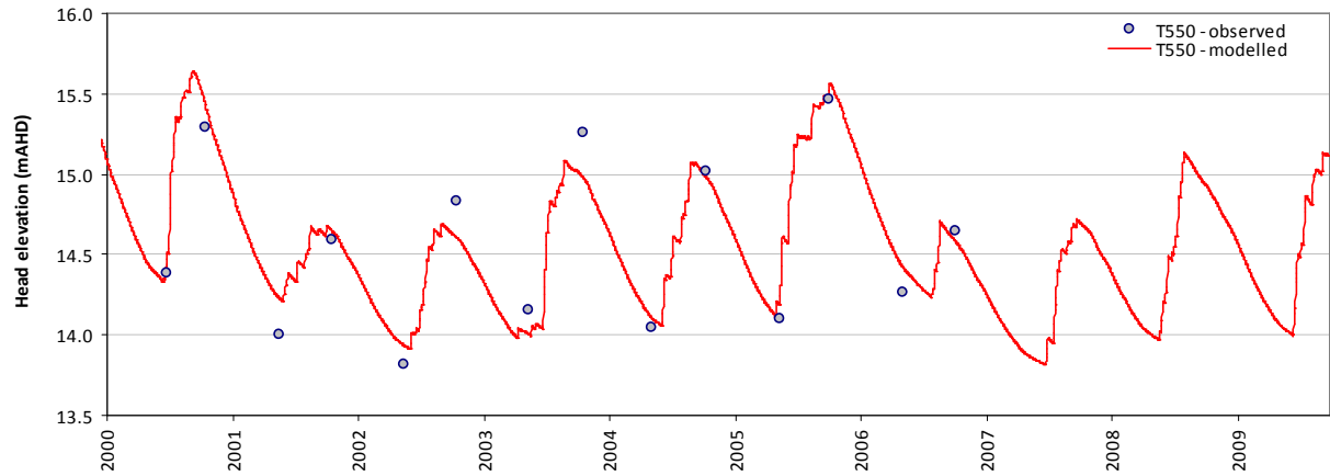
Modelled vs observed time-series plot - T550
