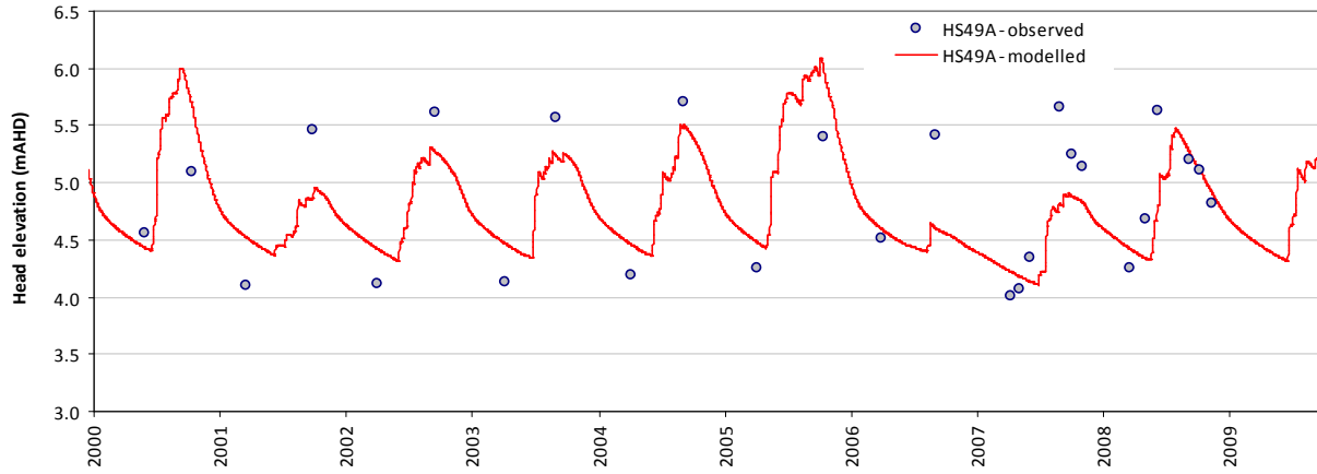
Modelled vs observed time-series plot - HS49A
