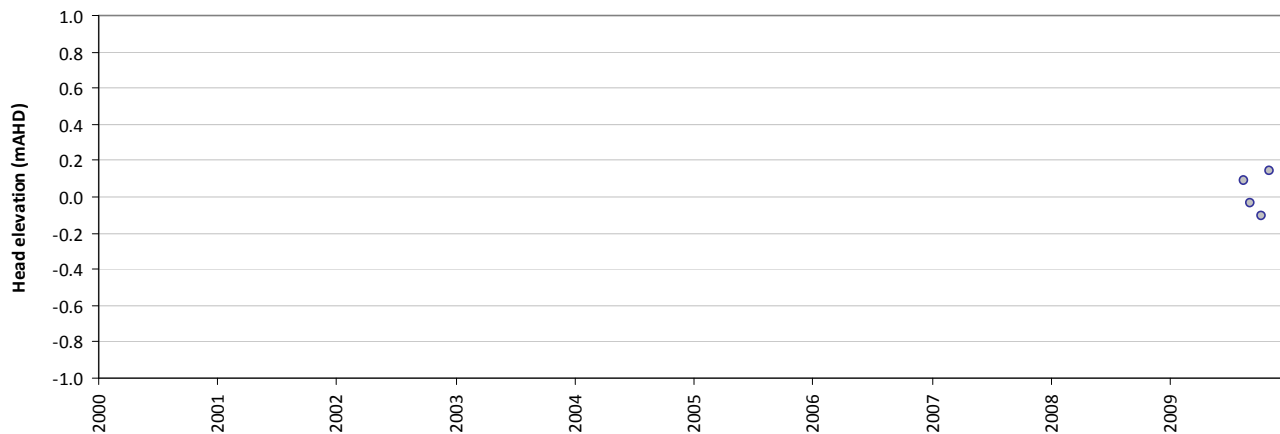
Residual time-series plot - PLI5180
