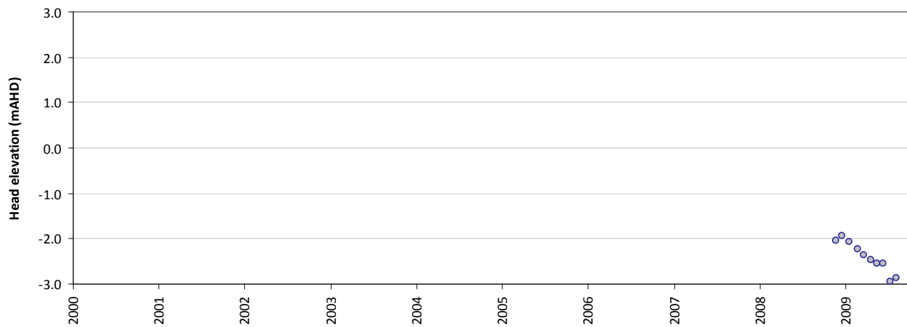
Residual time-series plot - HS76B
