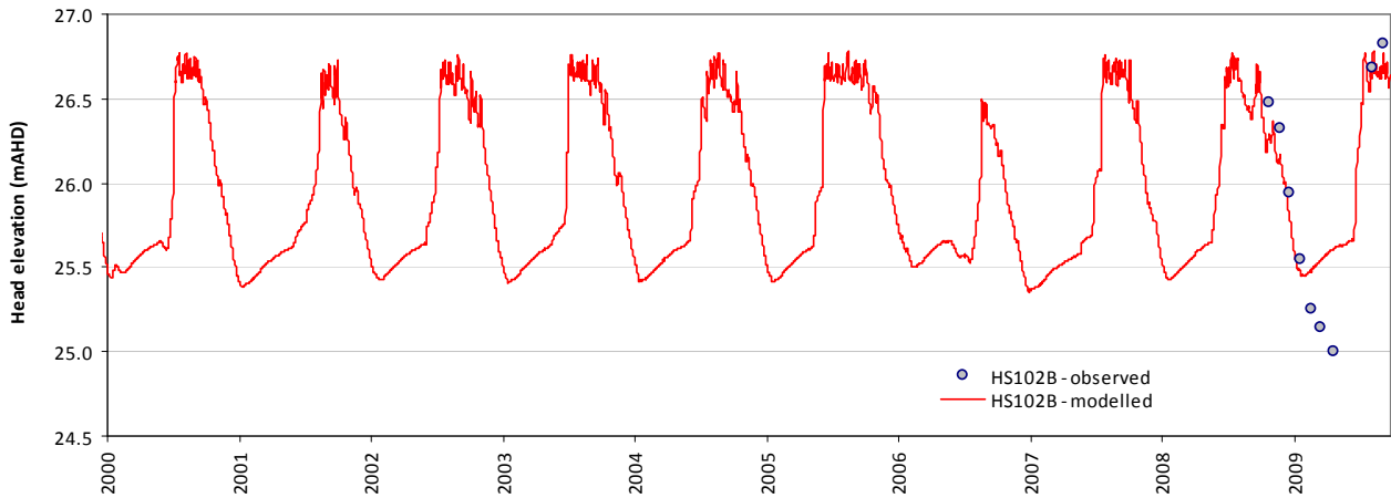
Modelled vs observed time-series plot - HS102B
