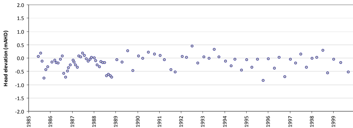
Residual time-series plot - T610
