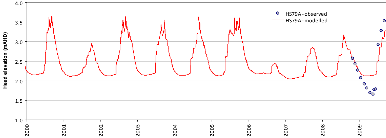
Modelled vs observed time-series plot - HS79A
