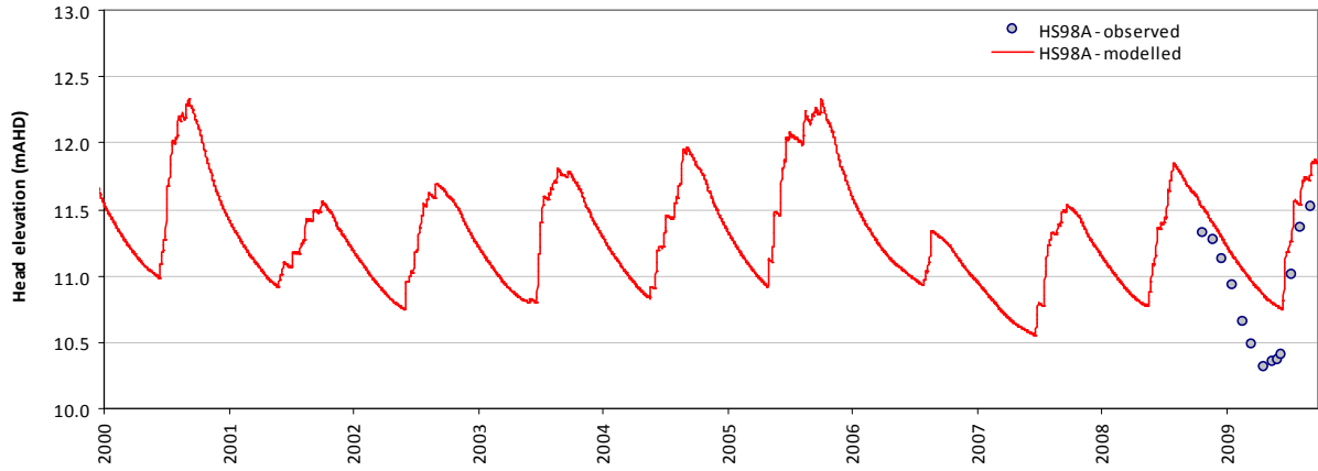
Modelled vs observed time-series plot - HS98A
