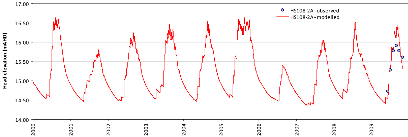
Modelled vs observed time-series plot - HS108-2A
