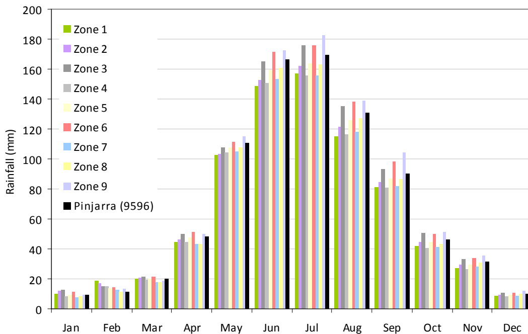
Figure 3-7: Monthly rainfall (1985 - 2009) for the nine climate zones in the Murray study area and for the Pinjarra rainfall gauging station (9596)
