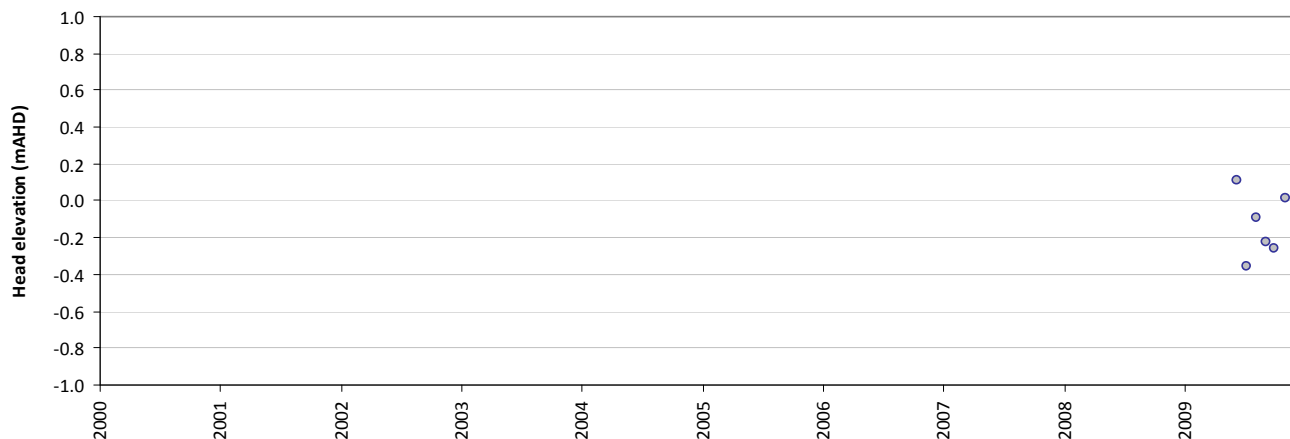
Residual time-series plot - HS109-1
