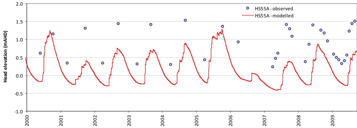
Modelled vs observed time-series plot - HS55A
