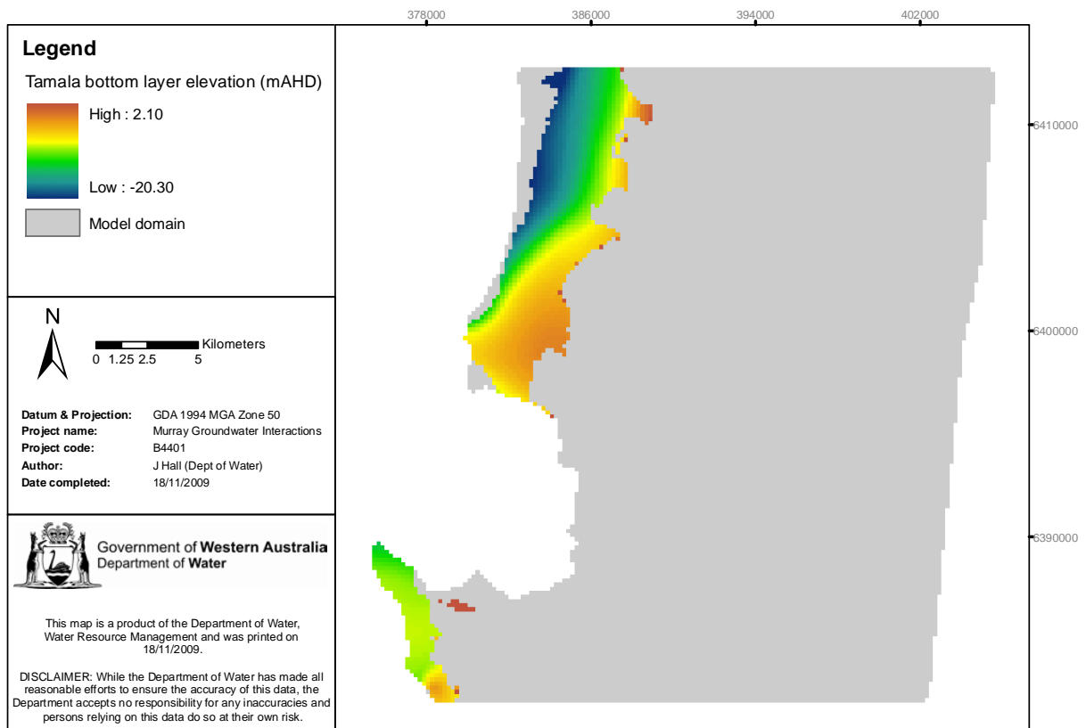
Figure 3-25: Tamala Limestone: base of geological formation (mAHD)
