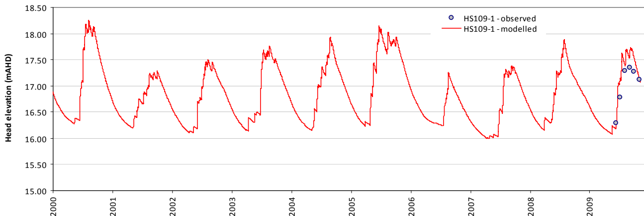
Modelled vs observed time-series plot - HS109-1
