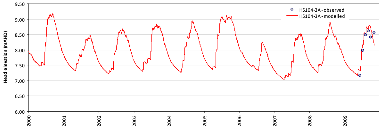
Modelled vs observed time-series plot - HS104-3A
