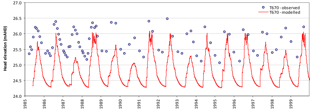
Modelled vs observed time-series plot - T670
