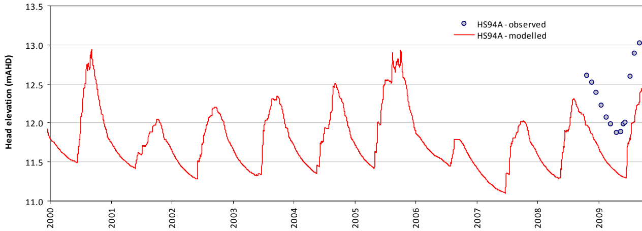
Modelled vs observed time-series plot - HS94A
