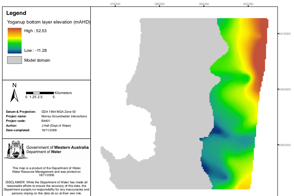
Figure 3-19: Yoganup Formation: base of geological formation (mAHd)
