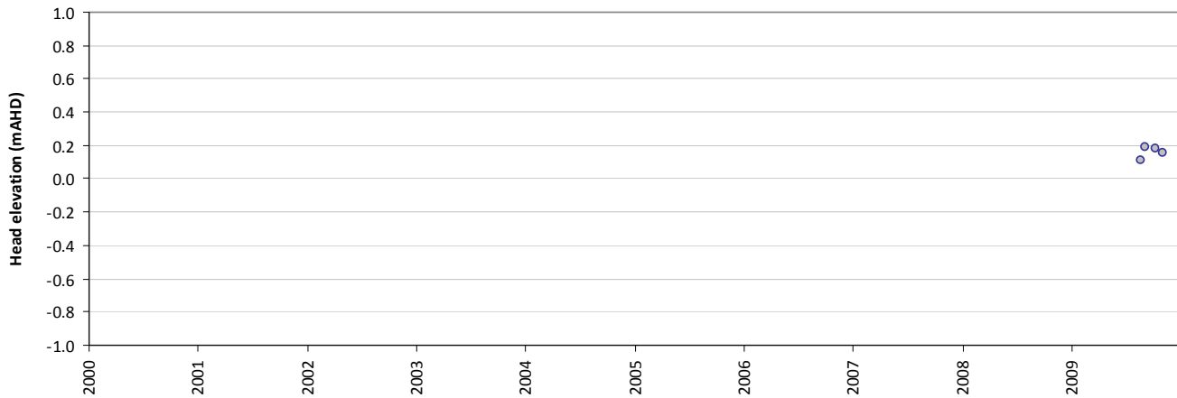
Residual time-series plot - PLI4835S
