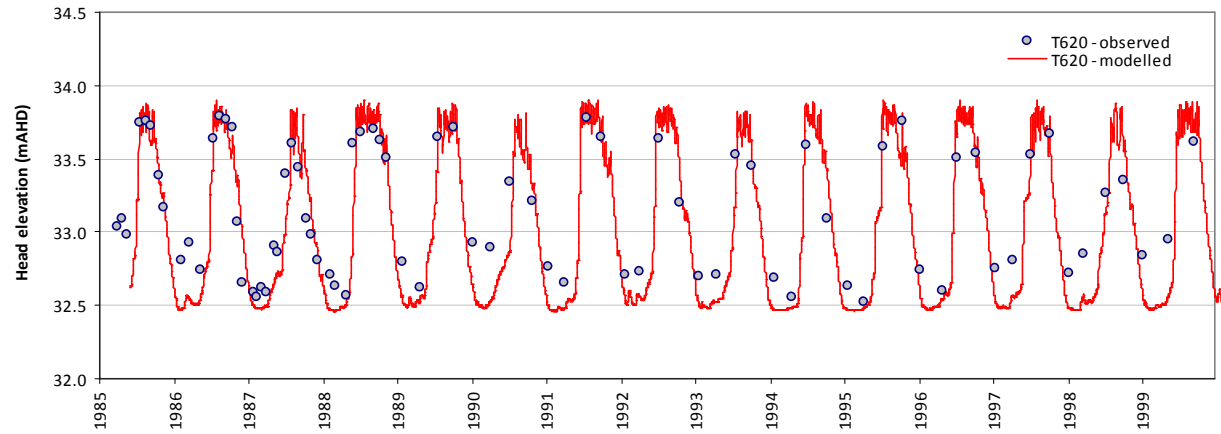
Modelled vs observed time-series plot - T620
