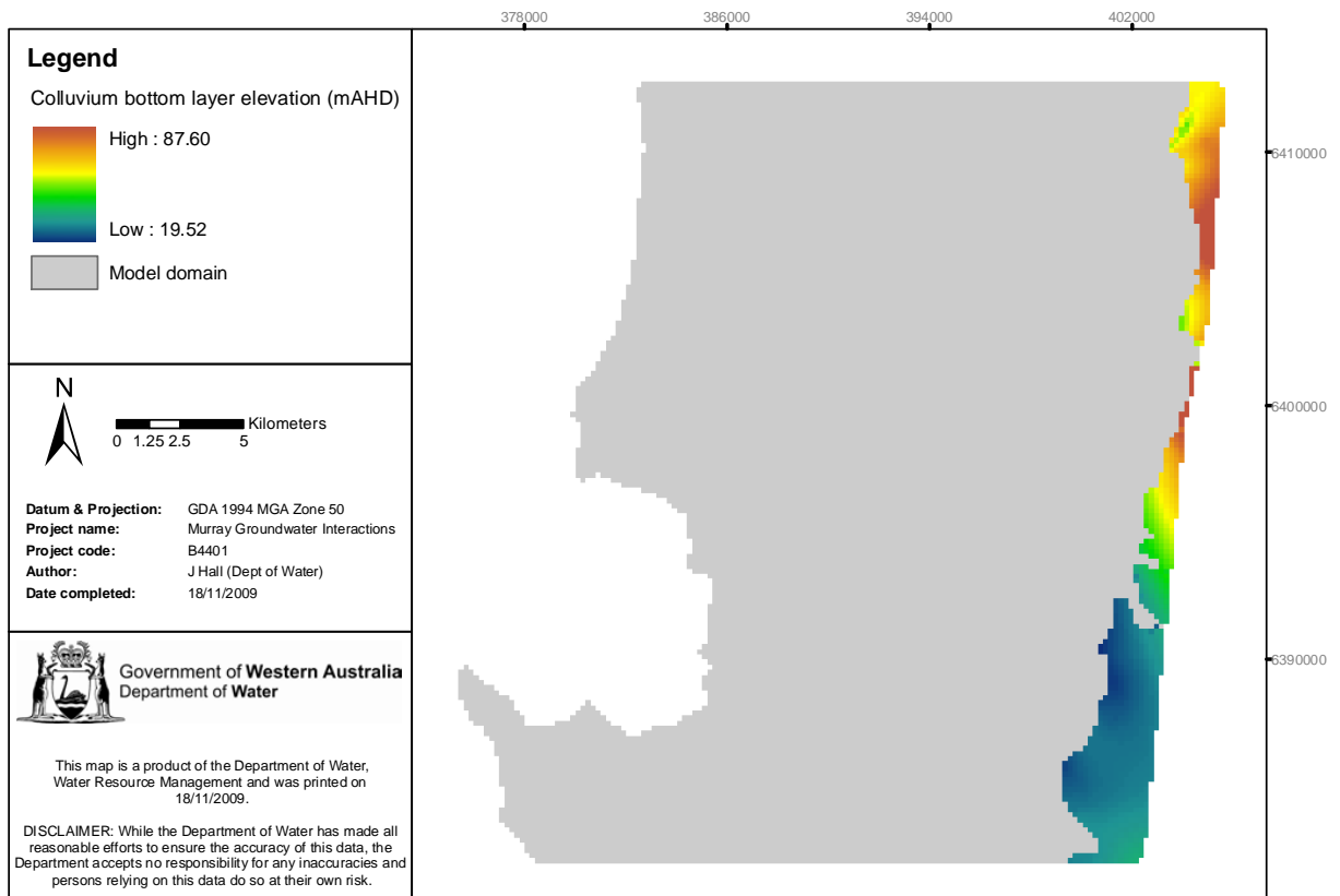
Figure 3-29: Colluvium: base of geological formation (mAHD)
