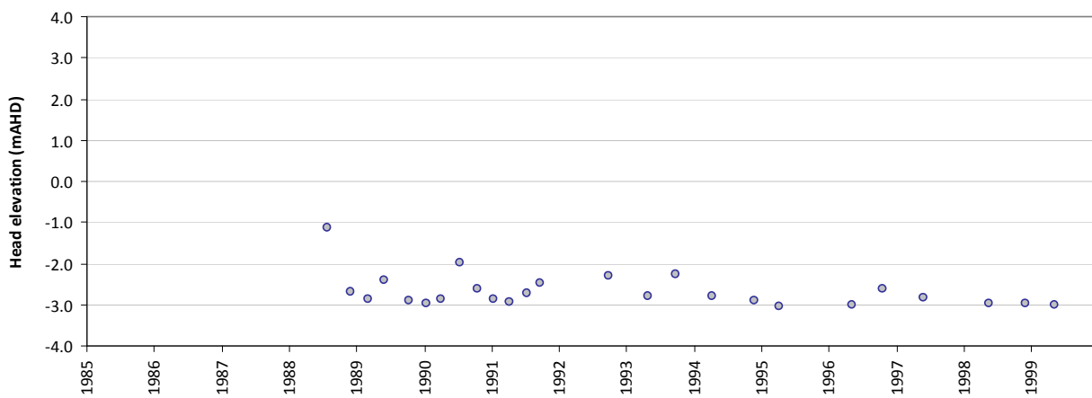
Residual time-series plot - HS51A
