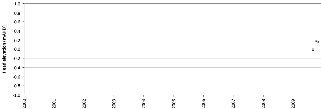
Residual time-series plot - PLI4835N
