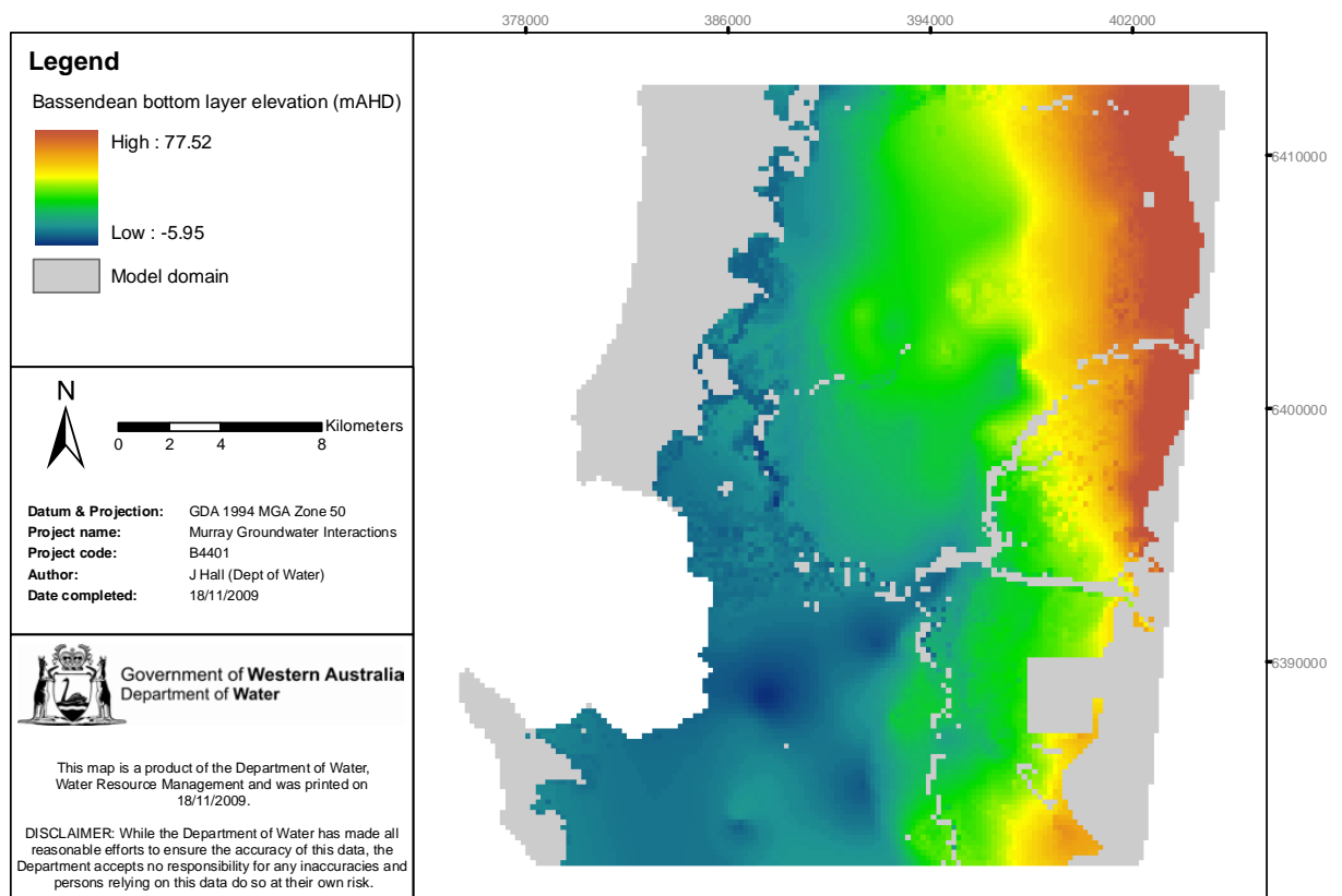
Figure 3-23: Bassendean Sand: base of geological formation (mAHD)
