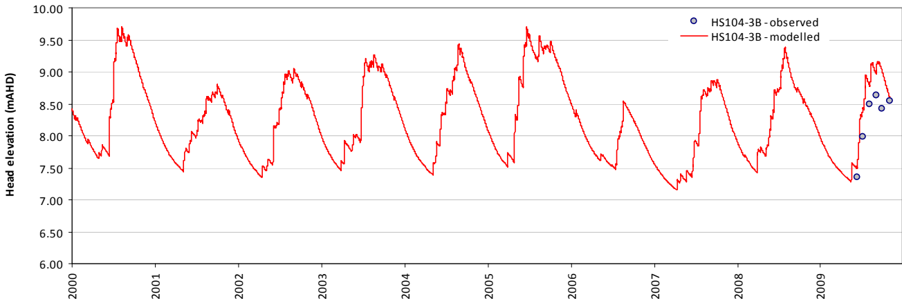
Modelled vs observed time-series plot - HS104-3B
