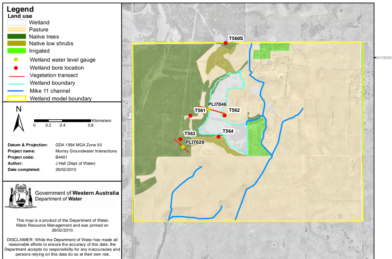
Figure 7-4: Elliot Road model: land use and monitoring locations
