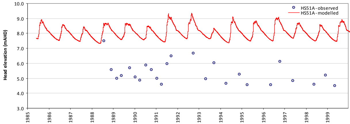
Modelled vs observed time-series plot - HS51A
