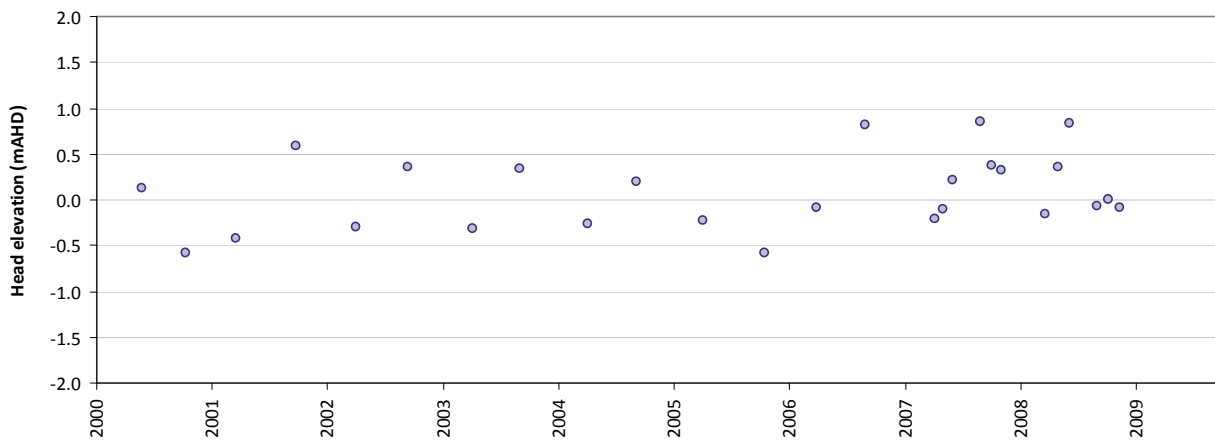
Residual time-series plot - HS49A
