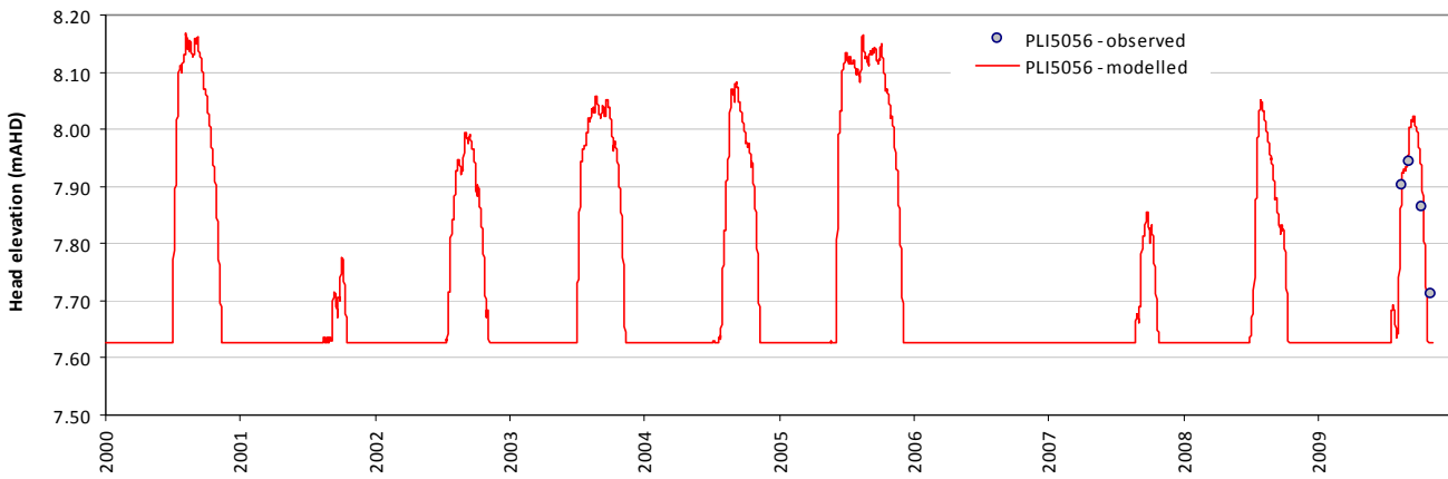
Modelled vs observed time-series plot - PLI5056
