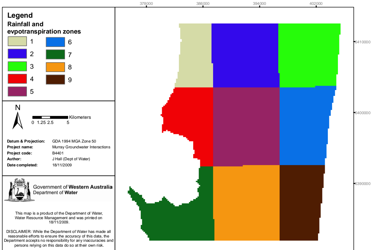
Figure 3-4: Climate zones (evapotranspiration and rainfall) for the Murray regional model
