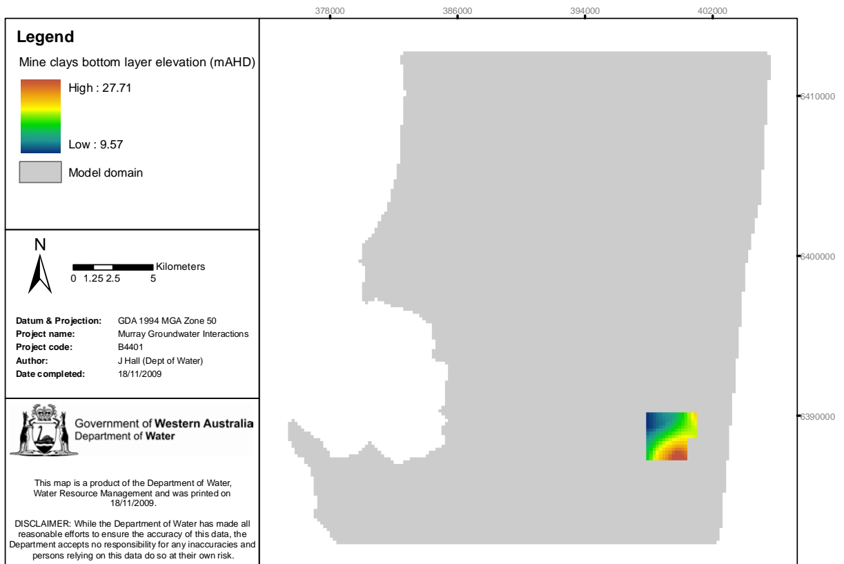
Figure 3-31: Mine clays: base of geological formation (mAHD)
