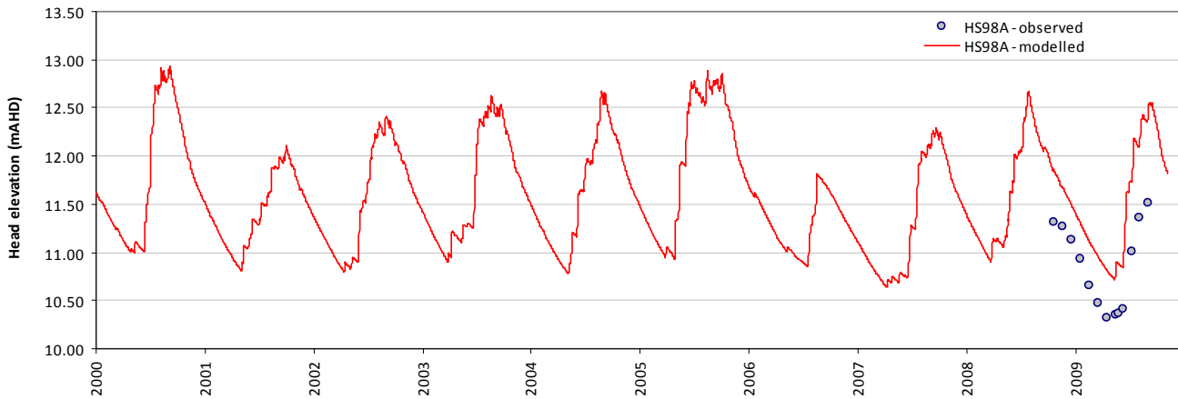
Modelled vs observed time-series plot - HS98A
