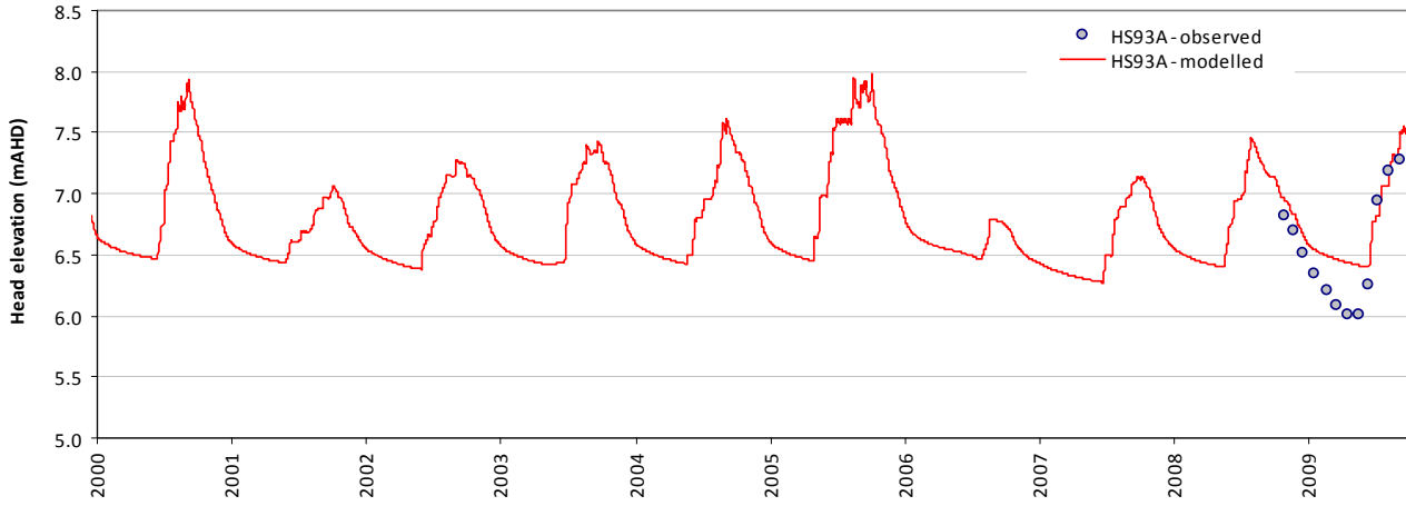
Modelled vs observed time-series plot - HS93A
