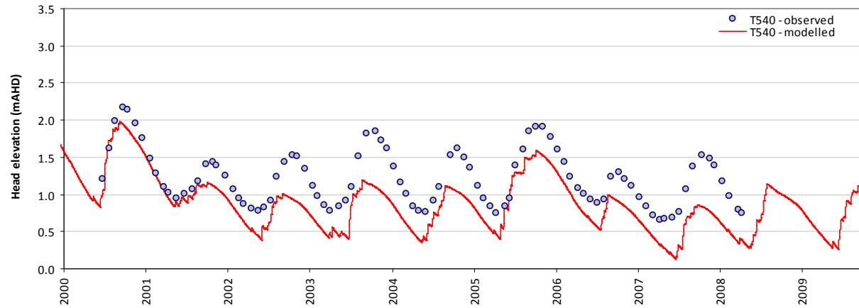
Modelled vs observed time-series plot - T540
