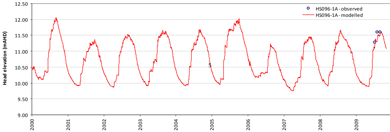
Modelled vs observed time-series plot - HS096-1A
