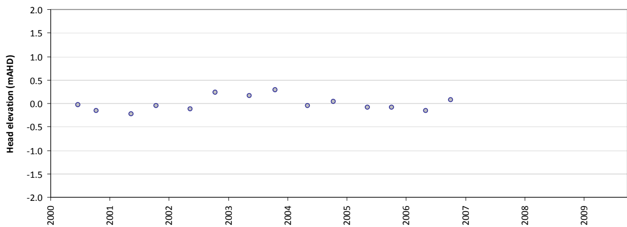
Residual time-series plot - T550
