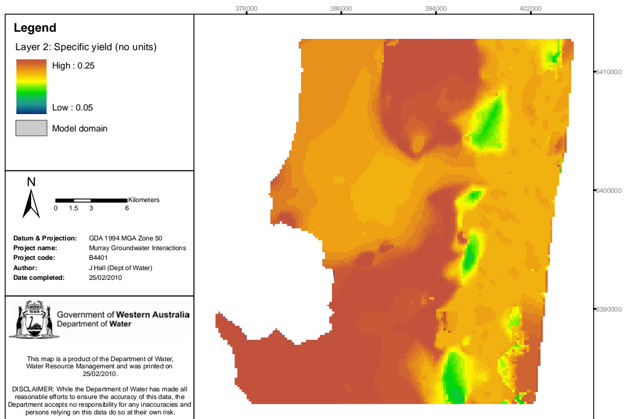
Figure 4-12: Computational layer 2 - specific yield
