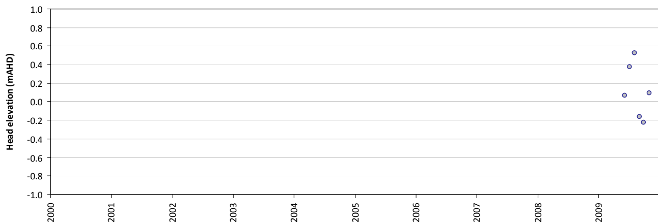
Residual time-series plot - HS104-2A
