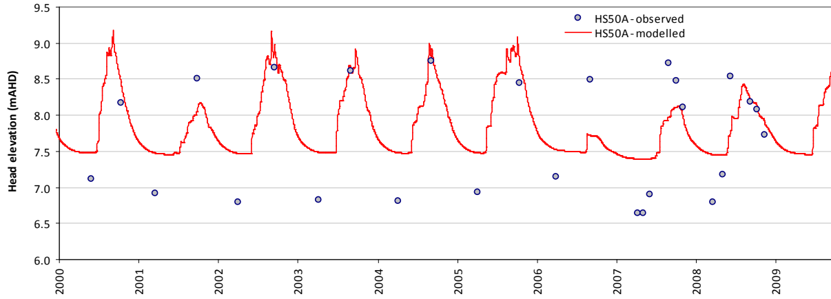
Modelled vs observed time-series plot - HS50A
