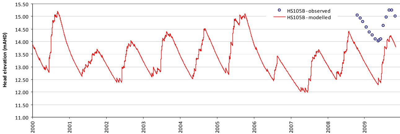
Modelled vs observed time-series plot - HS105B
