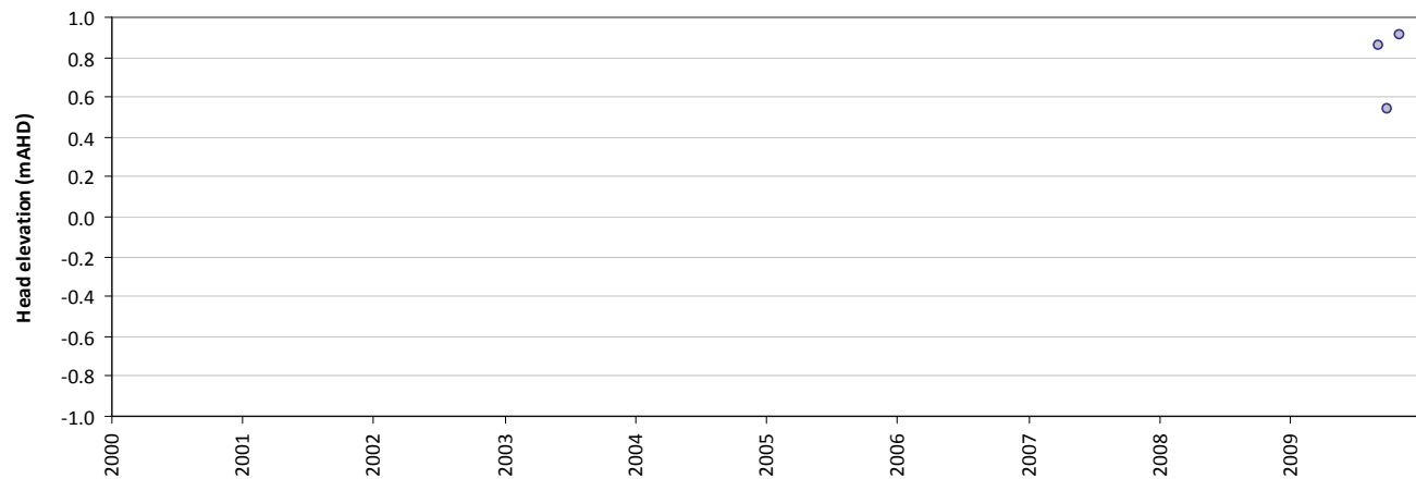
Residual time-series plot - HS80-1
