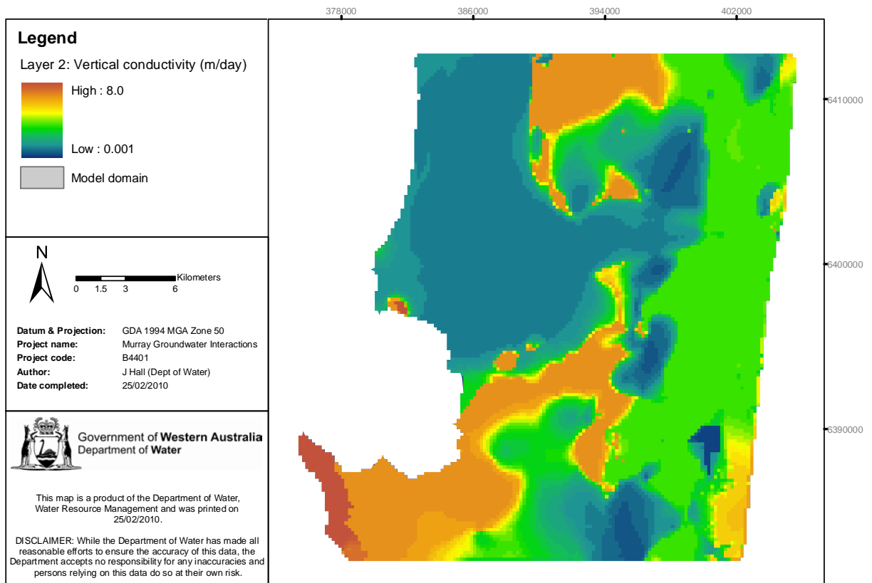
Figure 4-10: Computational layer 2 - vertical hydraulic conductivity (m/day)
