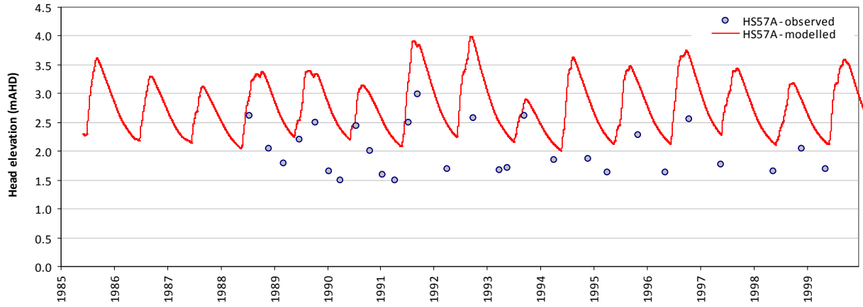
Modelled vs observed time-series plot - HS57A
