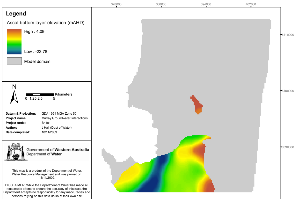
Figure 3-17: Ascot Formation: base of geological formation (mAHD)
