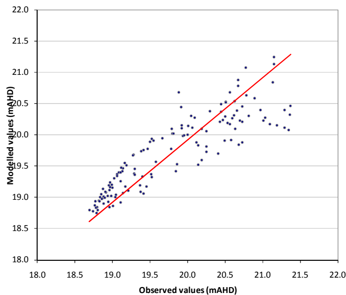
Figure E-1: Elliot Road wetland system scatterplot for observed vs modelled groundwater levels
