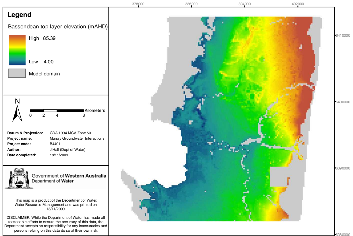
Figure 3-22: Bassendean Sand: top of geological formation (mAHD)
