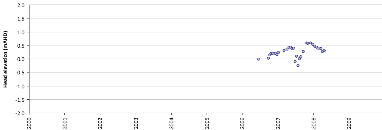
Residual time-series plot - LP15
