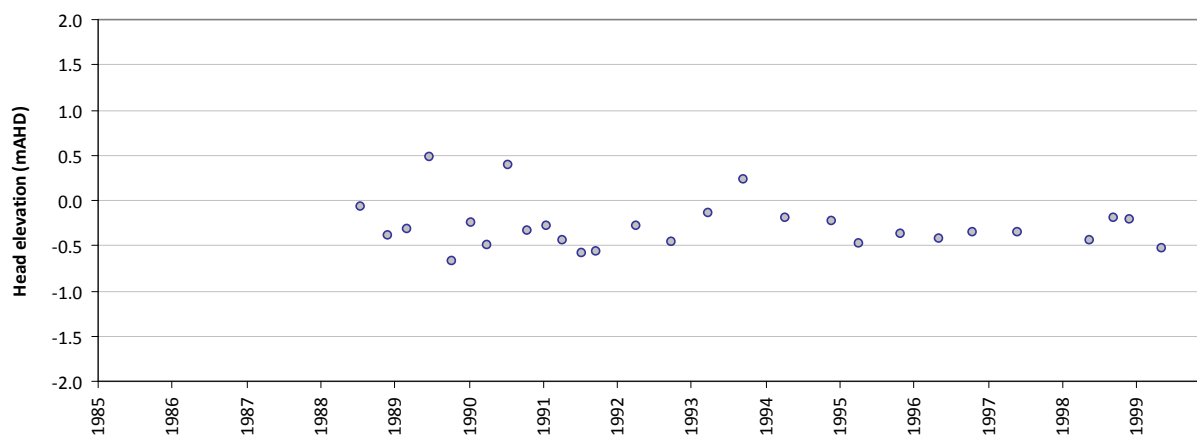
Residual time-series plot - HS54A
