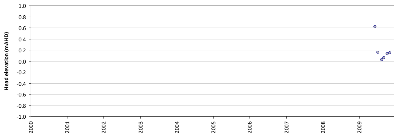
Residual time-series plot - HS087-1
