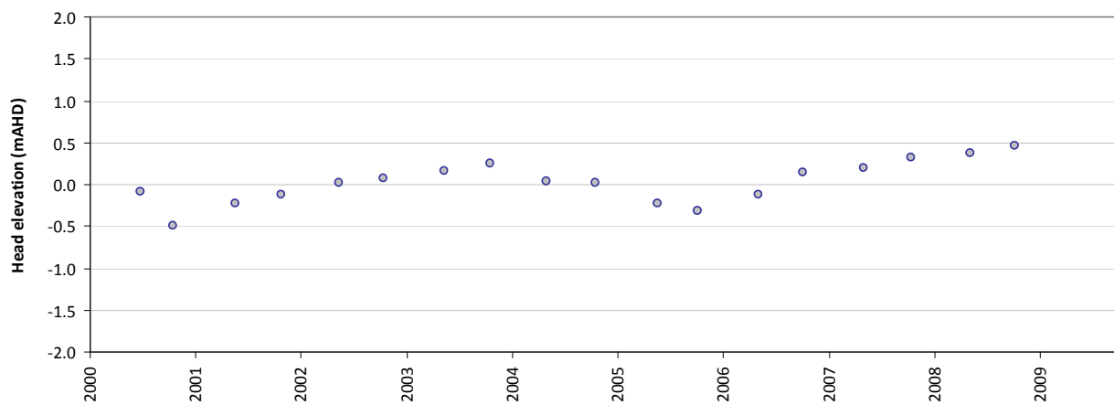
Residual time-series plot - T530
