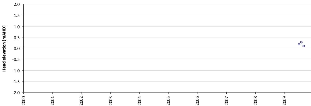
Residual time-series plot - HS096-1A
