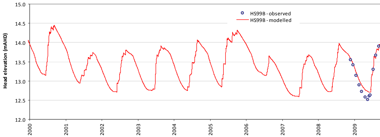
Modelled vs observed time-series plot - HS99B
