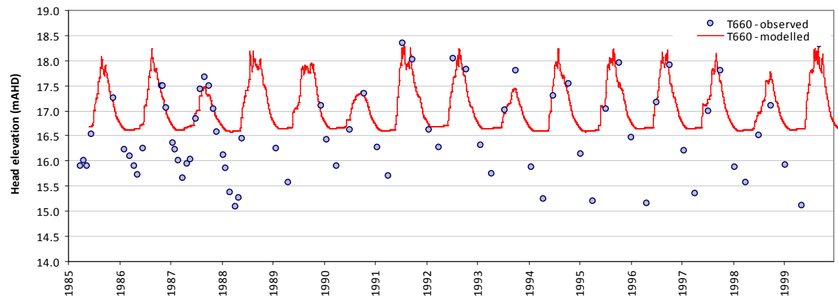
Modelled vs observed time-series plot - T660
