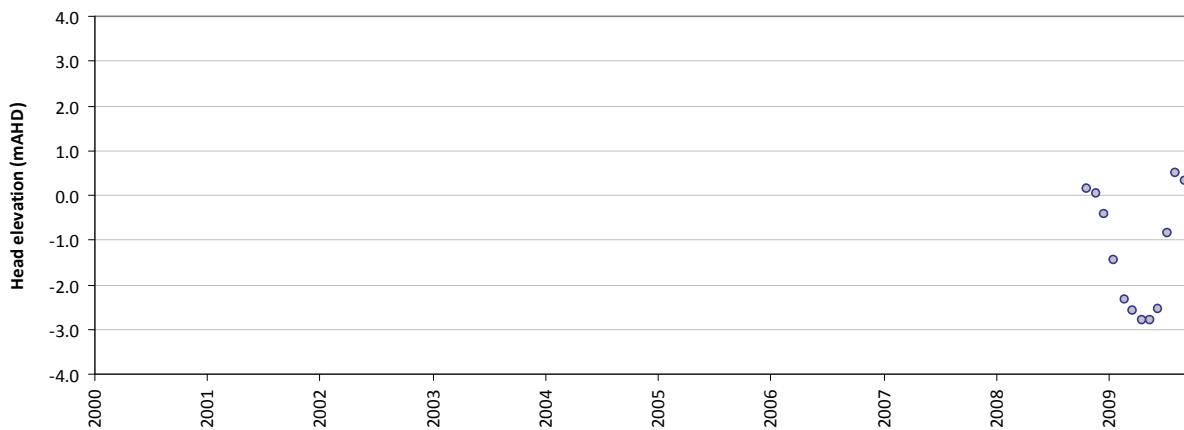
Residual time-series plot - HS103A
