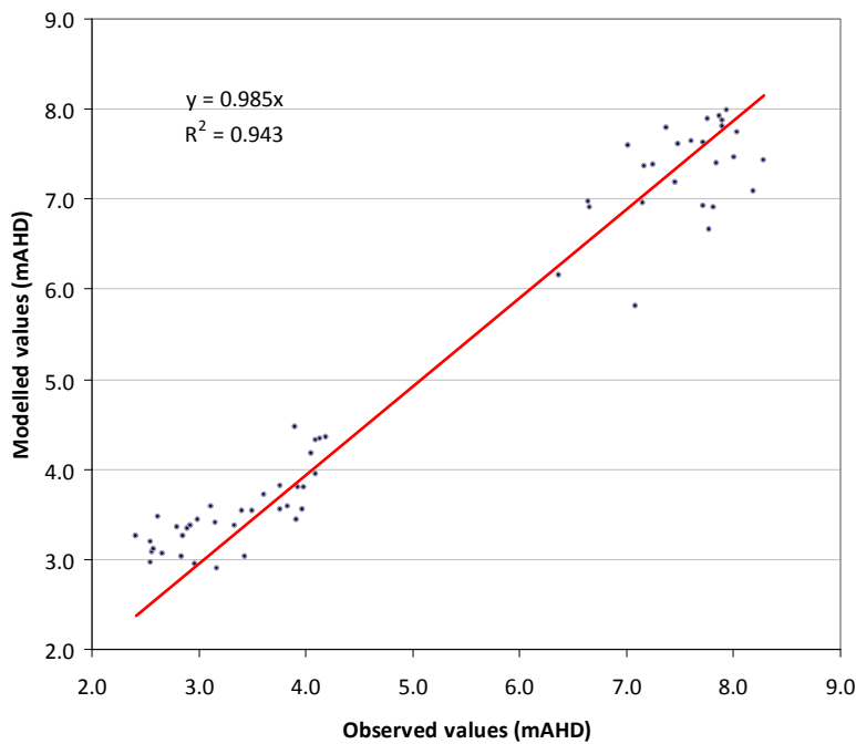
Figure G-1: Phillips Road wetland system scatterplot for observed vs modelled groundwater levels
