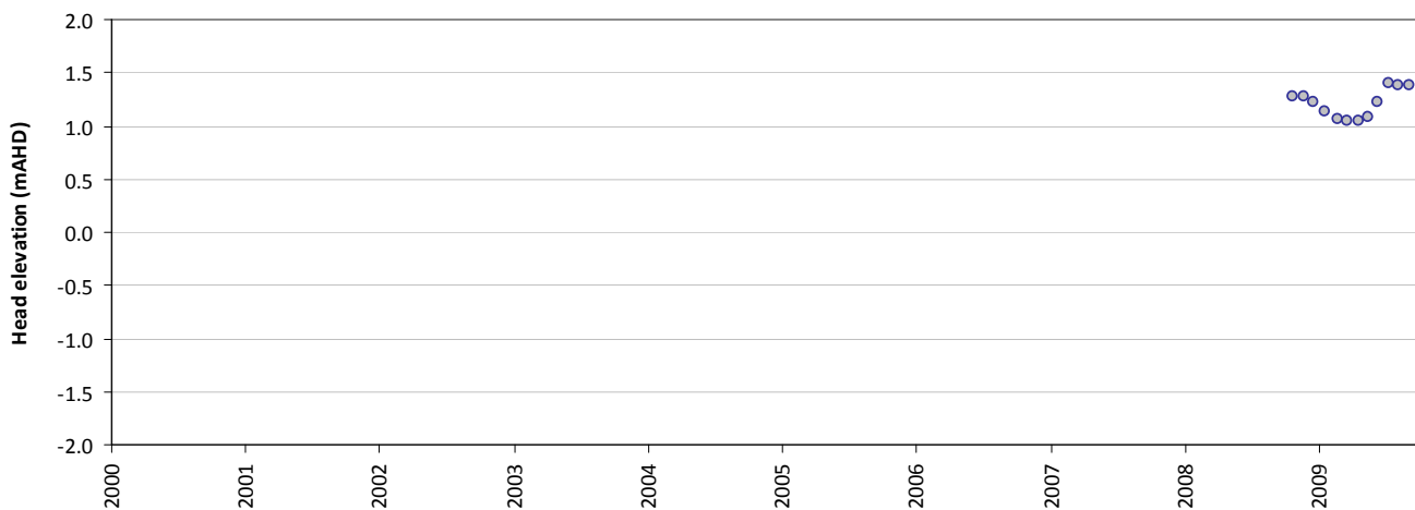
Residual time-series plot - HS89B
