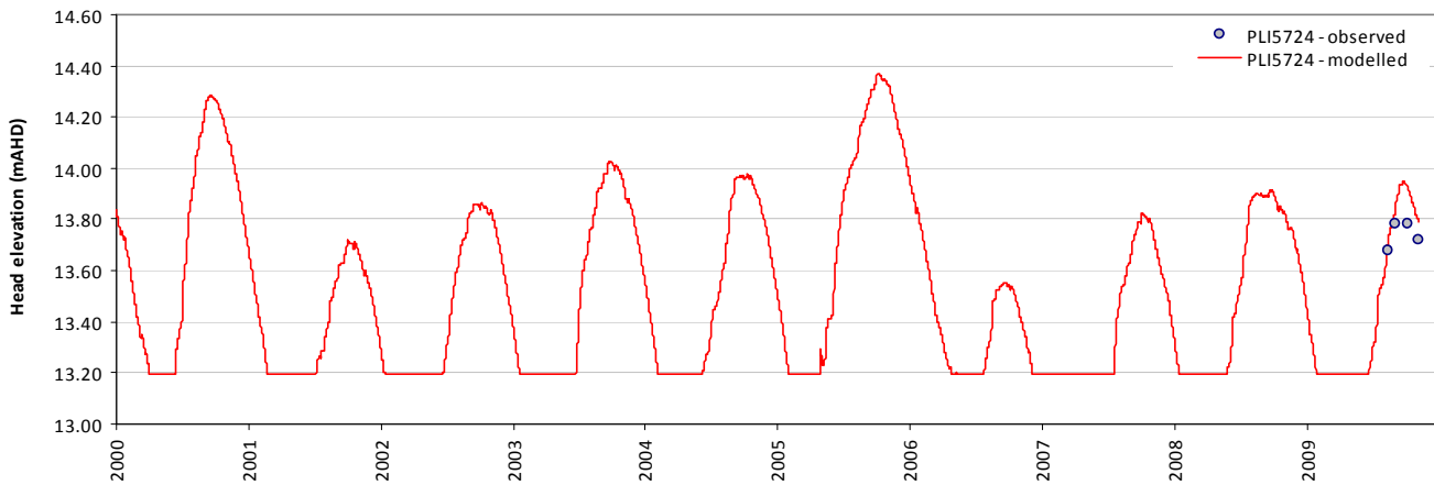
Modelled vs observed time-series plot - PLI5724
