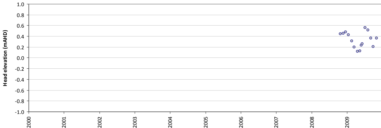
Residual time-series plot - HS97A
