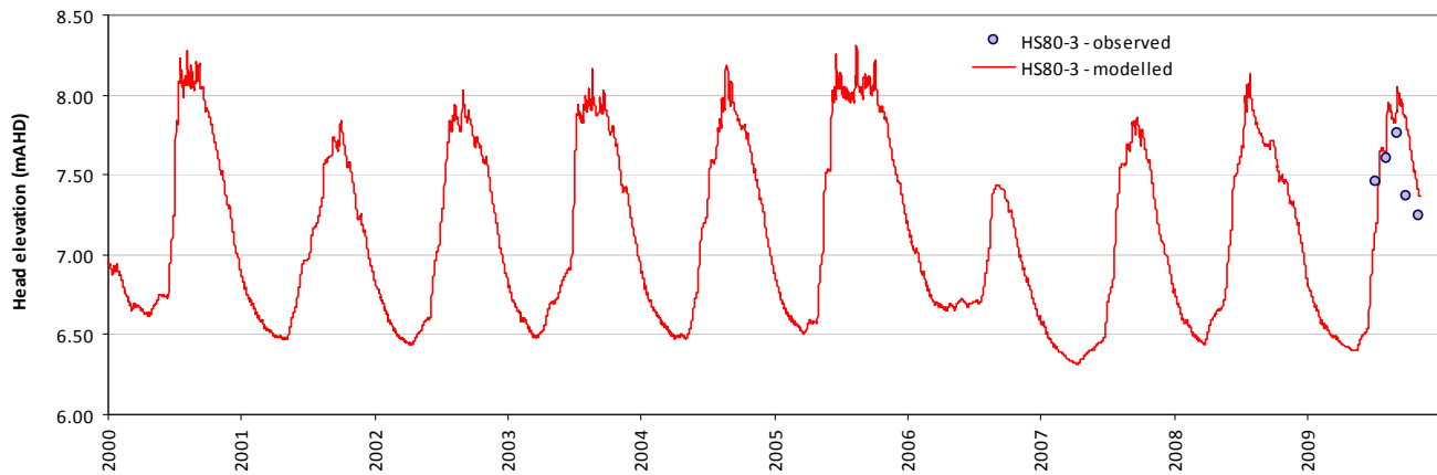
Modelled vs observed time-series plot - HS80-3
