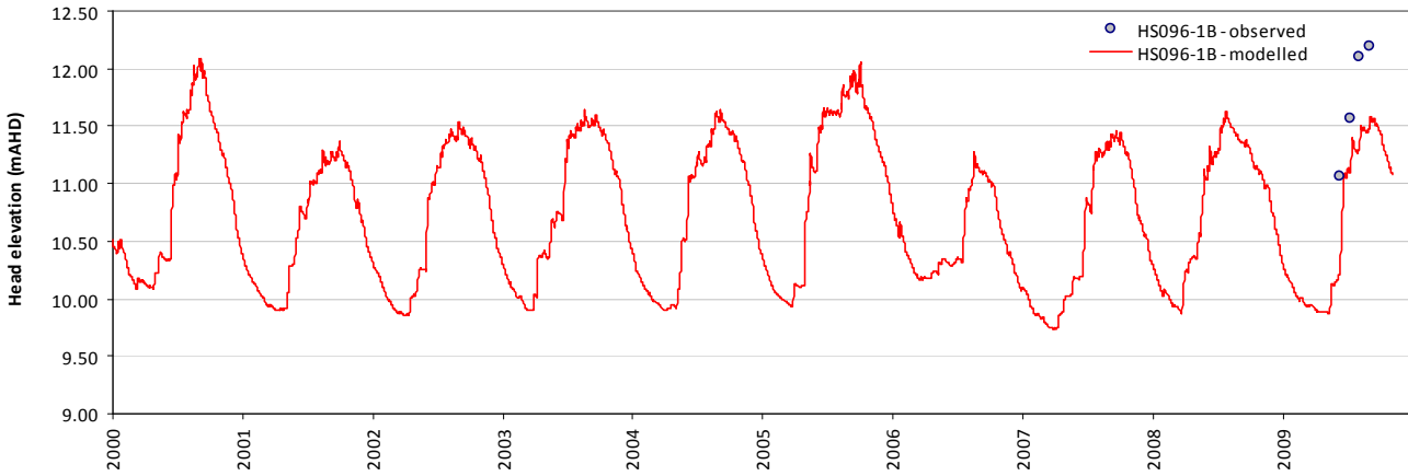
Modelled vs observed time-series plot - HS096-1B
