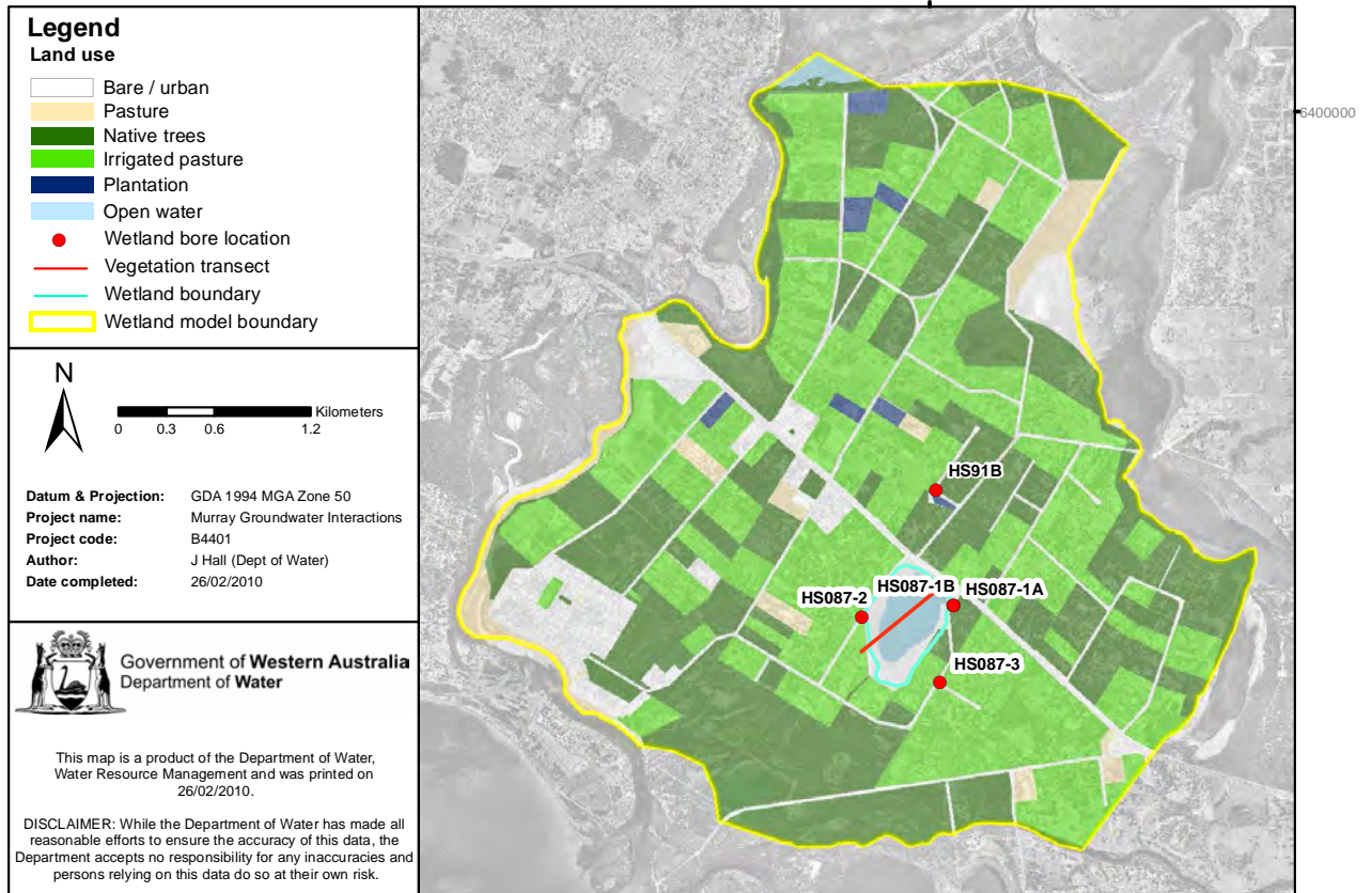
Figure 7-2: Barragup wetland model: land use and monitoring locations
