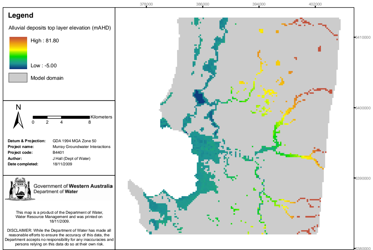
Figure 3-26: Alluvium, estuarine deposits and swamp deposits: top of formation (mAHD)
