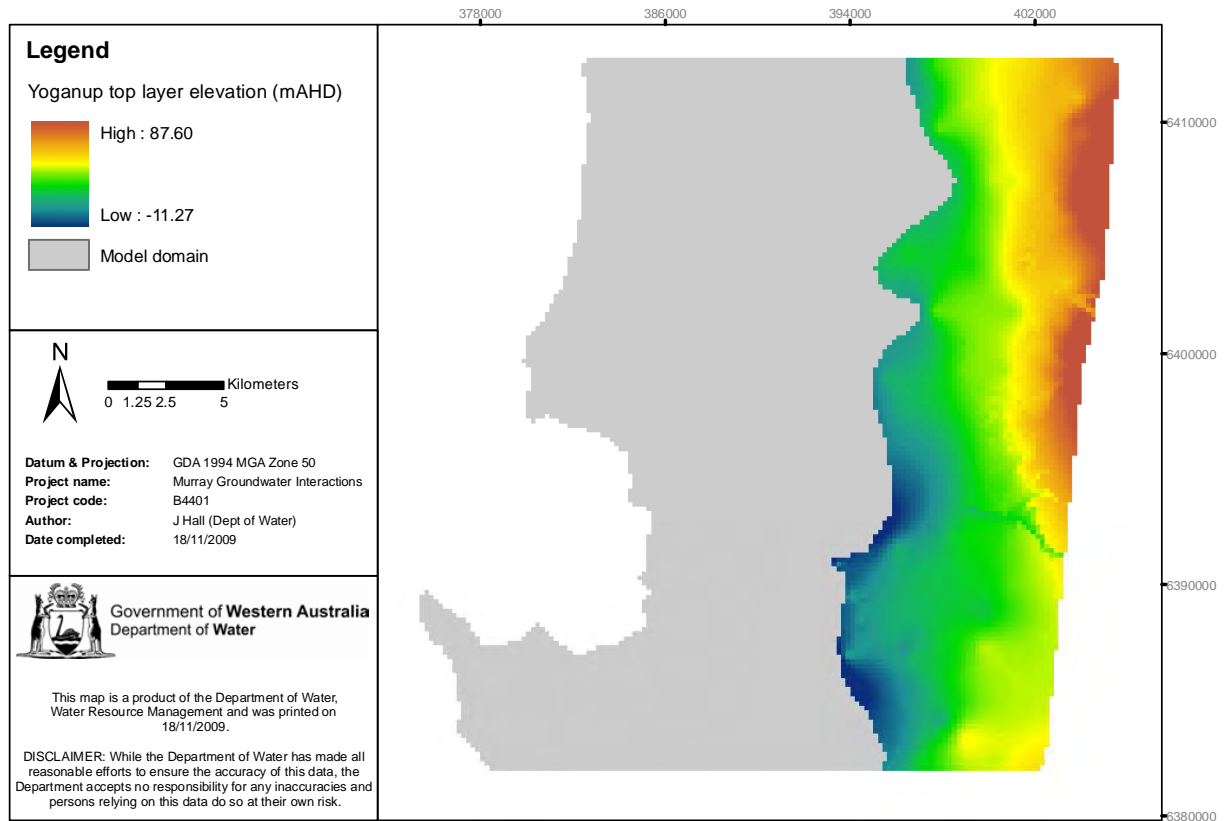
Figure 3-18: Yoganup Formation: top of geological formation (mAHd)
