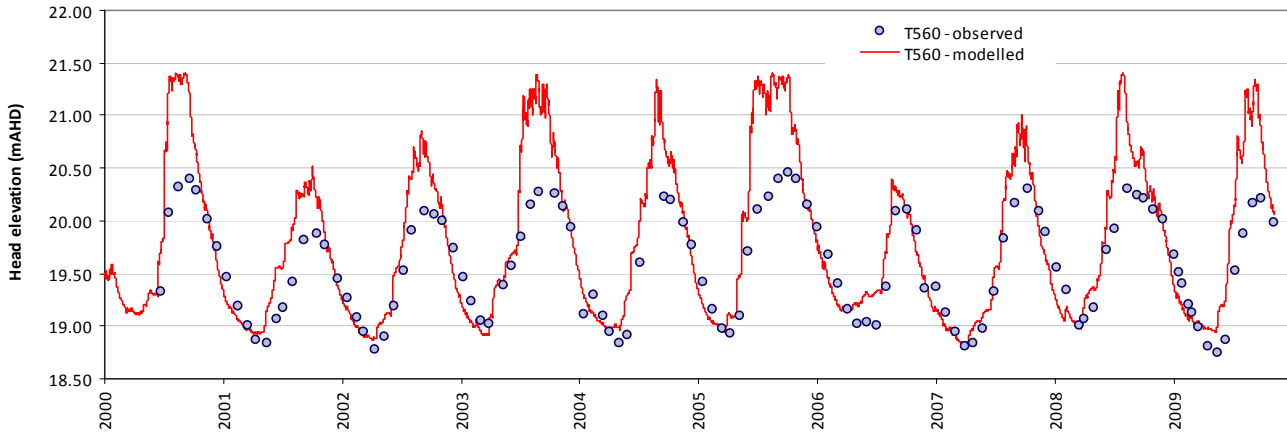
Modelled vs observed time-series plot - T560
