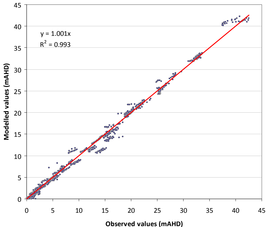
Figure 4-4: Validation scatter plot for the observed versus modelled heads in the Murray regional model
