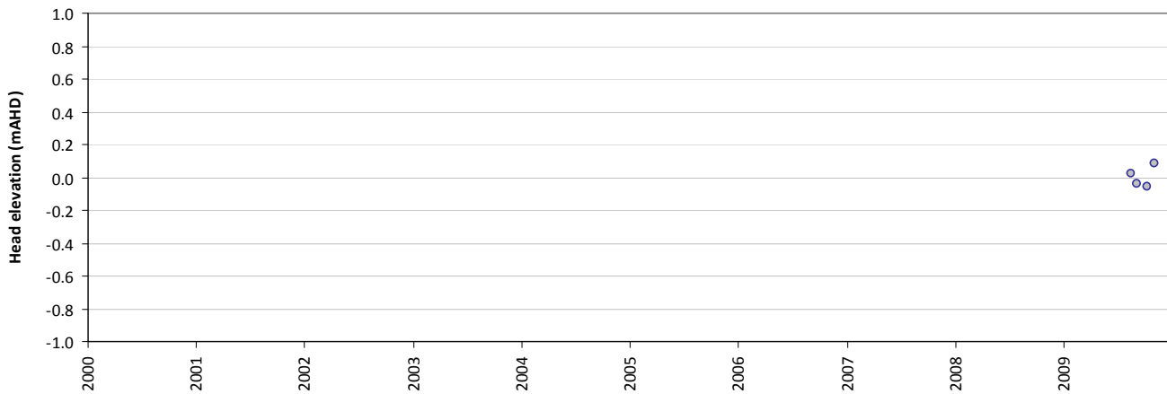
Residual time-series plot - PLI5056
