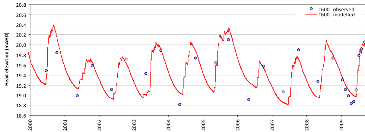
Modelled vs observed time-series plot - T600
