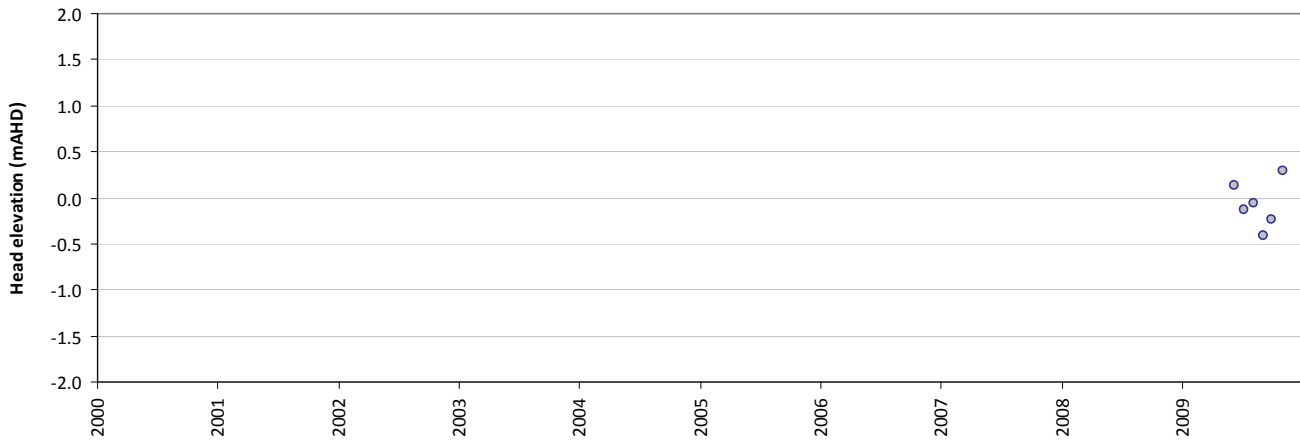
Residual time-series plot - HS108-2B
