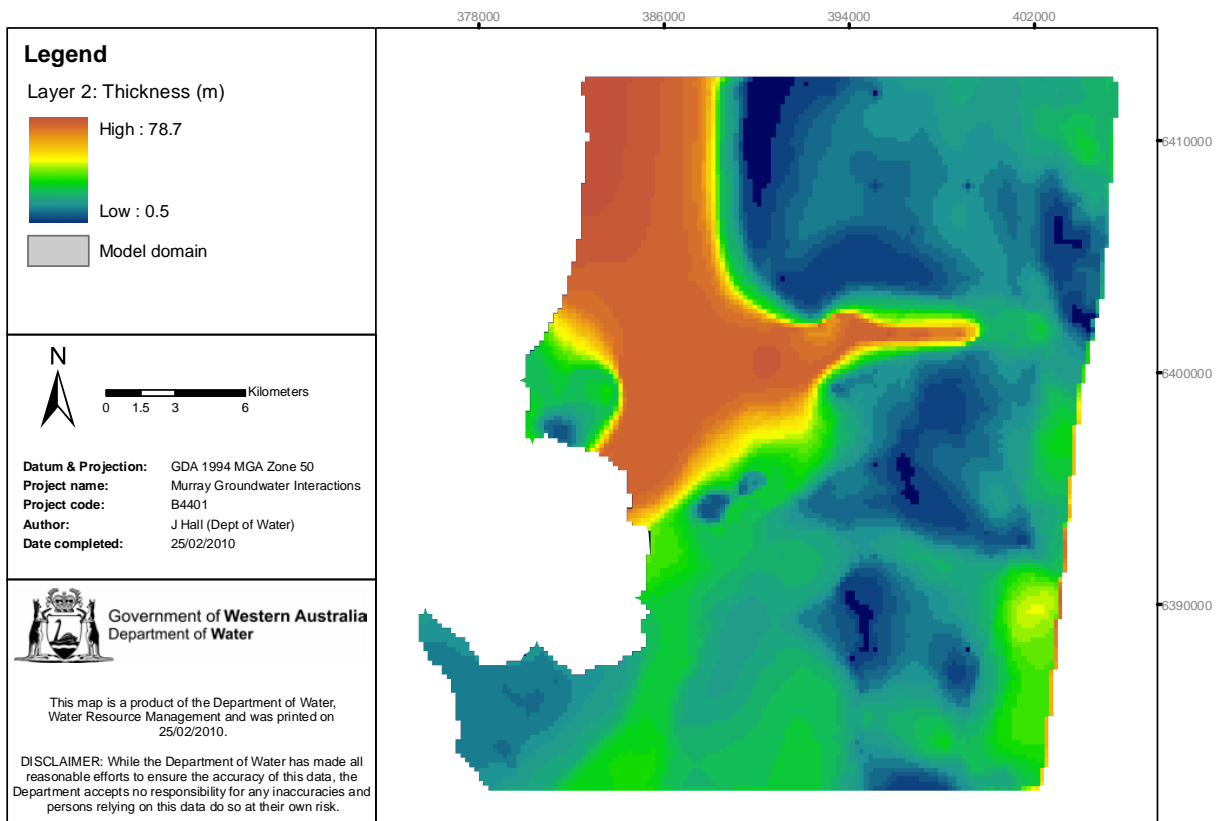
Figure 4-6: Computational layer 2 - thickness (m)
