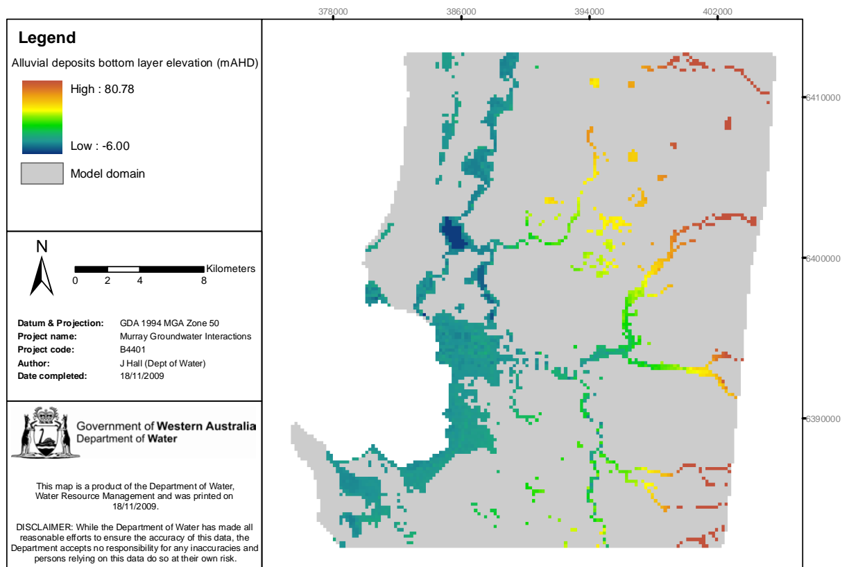
Figure 3-27 Alluvium, estuarine deposits and swamp deposits: base of formation (mAHD)
