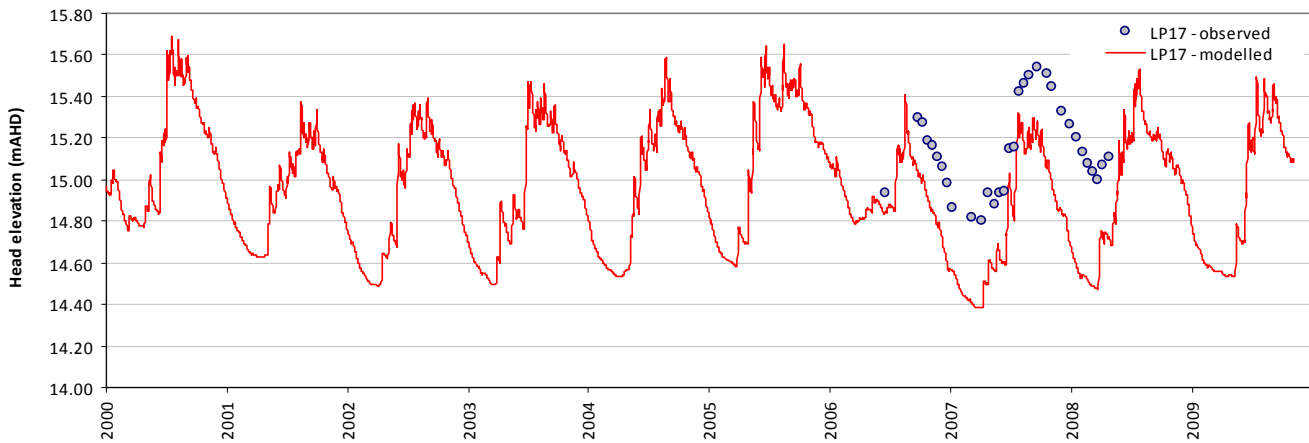
Modelled vs observed time-series plot - LP17
