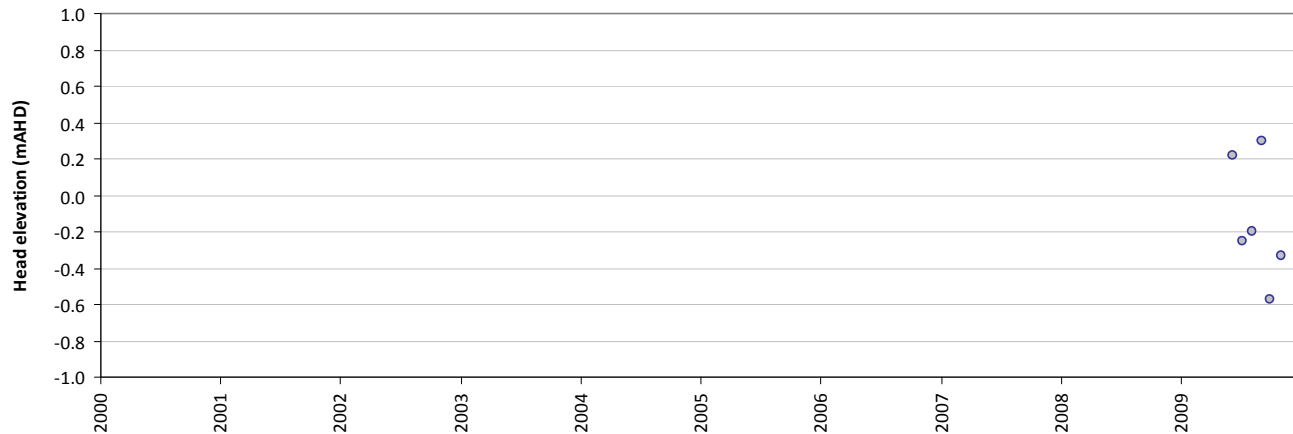
Residual time-series plot - HS80-2B
