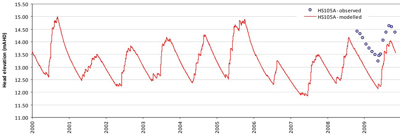
Modelled vs observed time-series plot - HS105A
