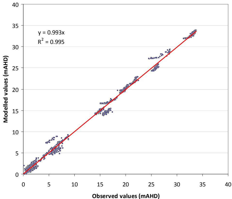
Figure 4-2: Calibration scatter plot for the observed versus modelled heads in the Murray Mike SHE model
