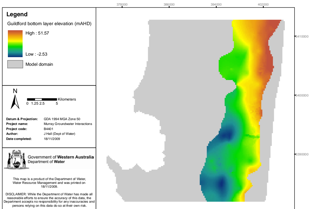
Figure 3-21: Guildford Clay: base of geological formation (mAHD)
