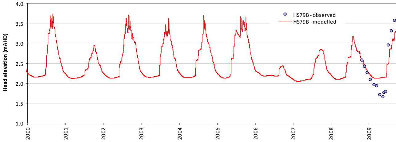
Modelled vs observed time-series plot - HS79B
