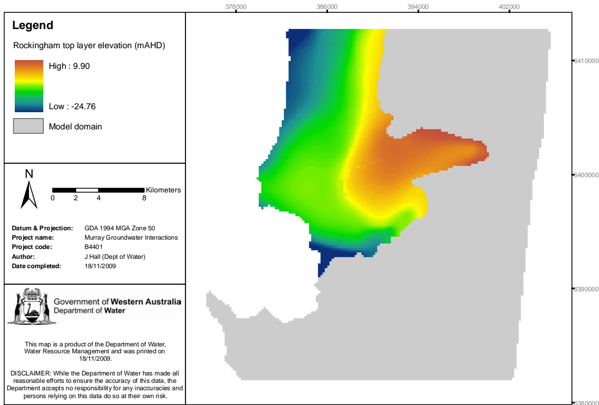
Figure 3-14: Rockingham Sand: top of geological formation (mAHd)
