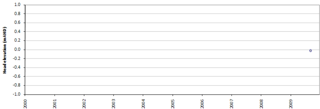
Residual time-series plot - PLI7029
