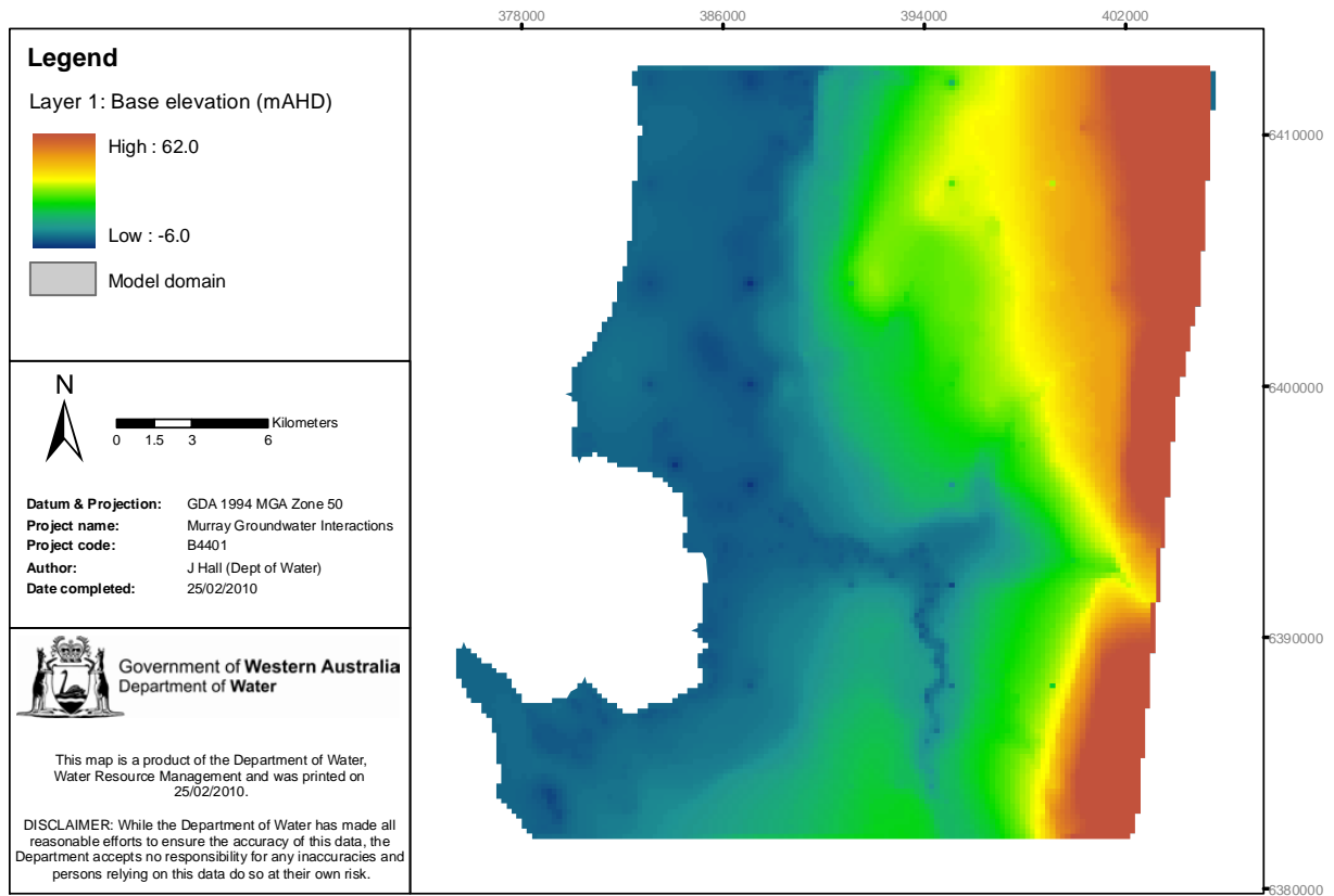
Figure 3-33: Base of computational layer 1(mAHD)
