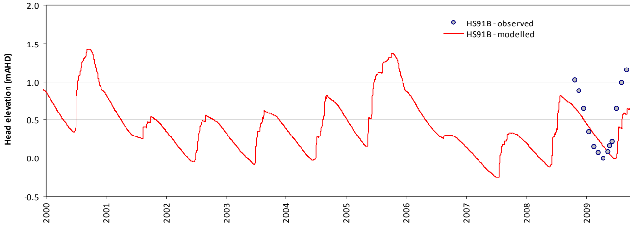
Modelled vs observed time-series plot - HS91B
