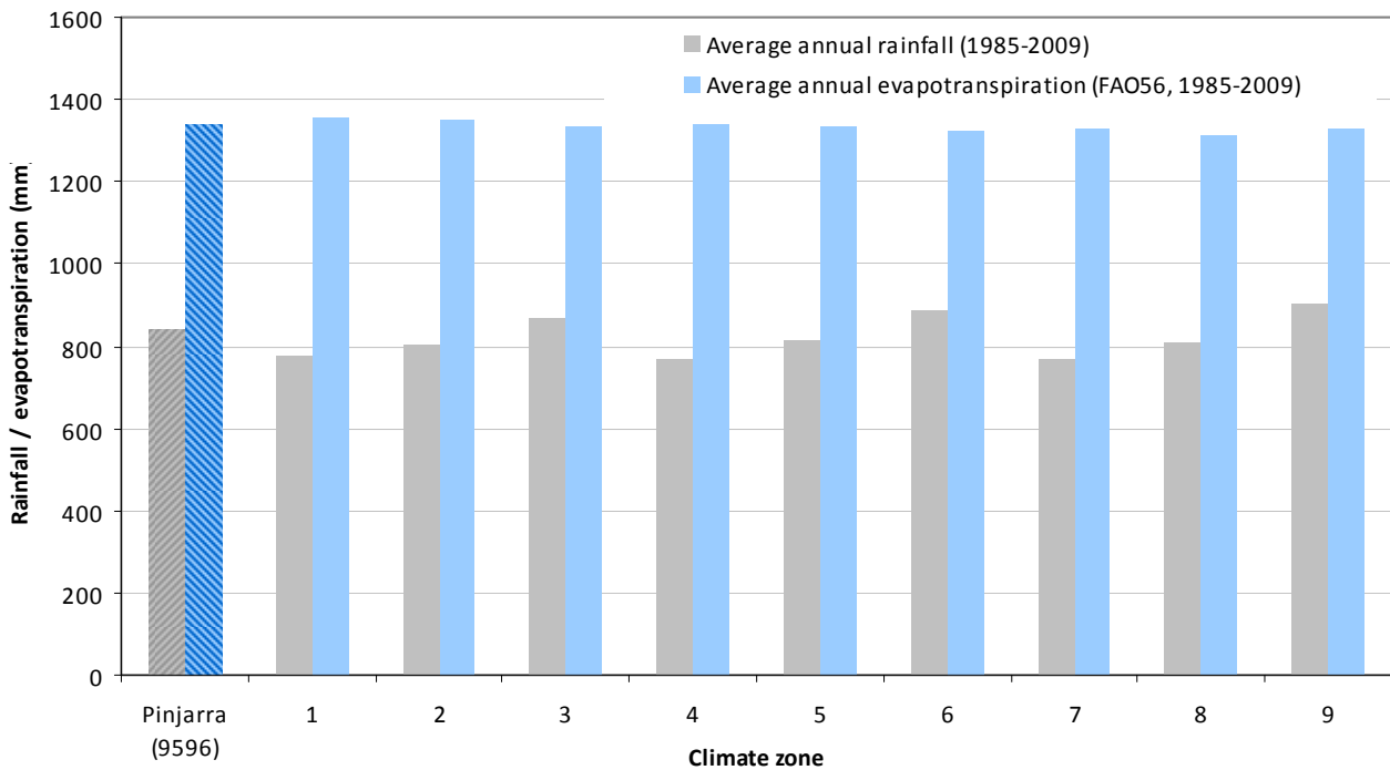
Figure 3-5: Average annual rainfall (1985 - 2009) and Penman-Monteith evapotranspiration for the nine climate zones in the Murray study area and for the Pinjarra rainfall gauging station (9596)
