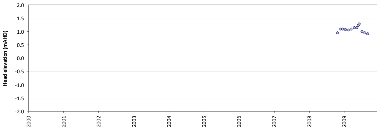
Residual time-series plot - HS98B
