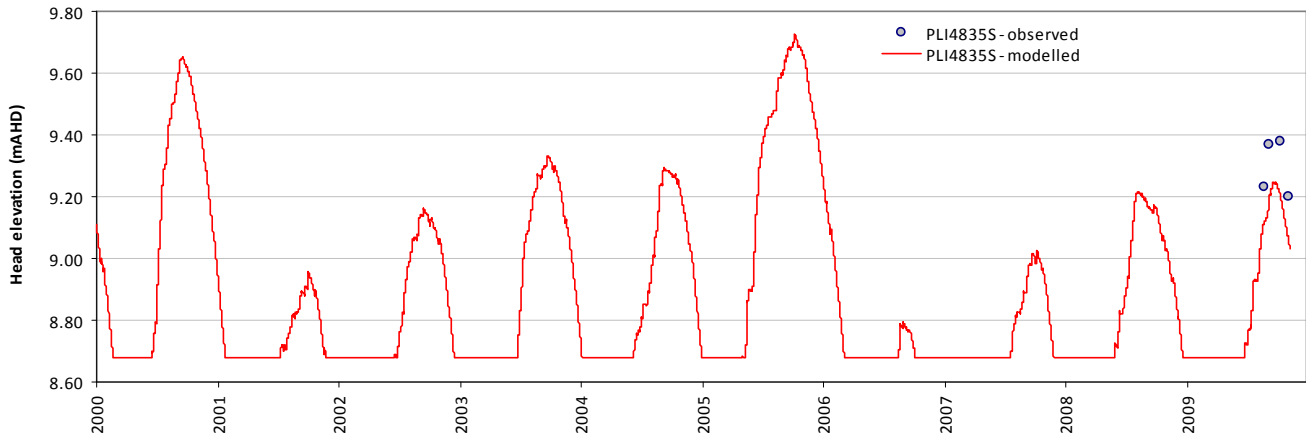
Modelled vs observed time-series plot - PLI4835S
