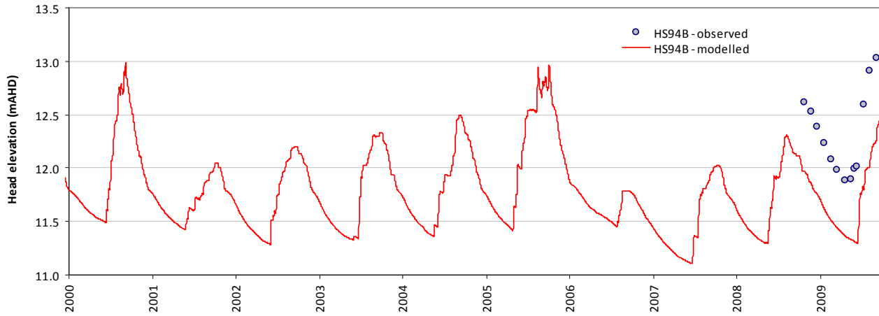
Modelled vs observed time-series plot - HS94B
