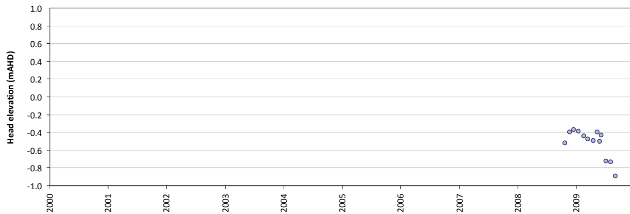
Residual time-series plot - HS98A
