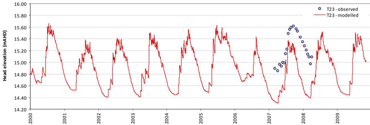
Modelled vs observed time-series plot - T23
