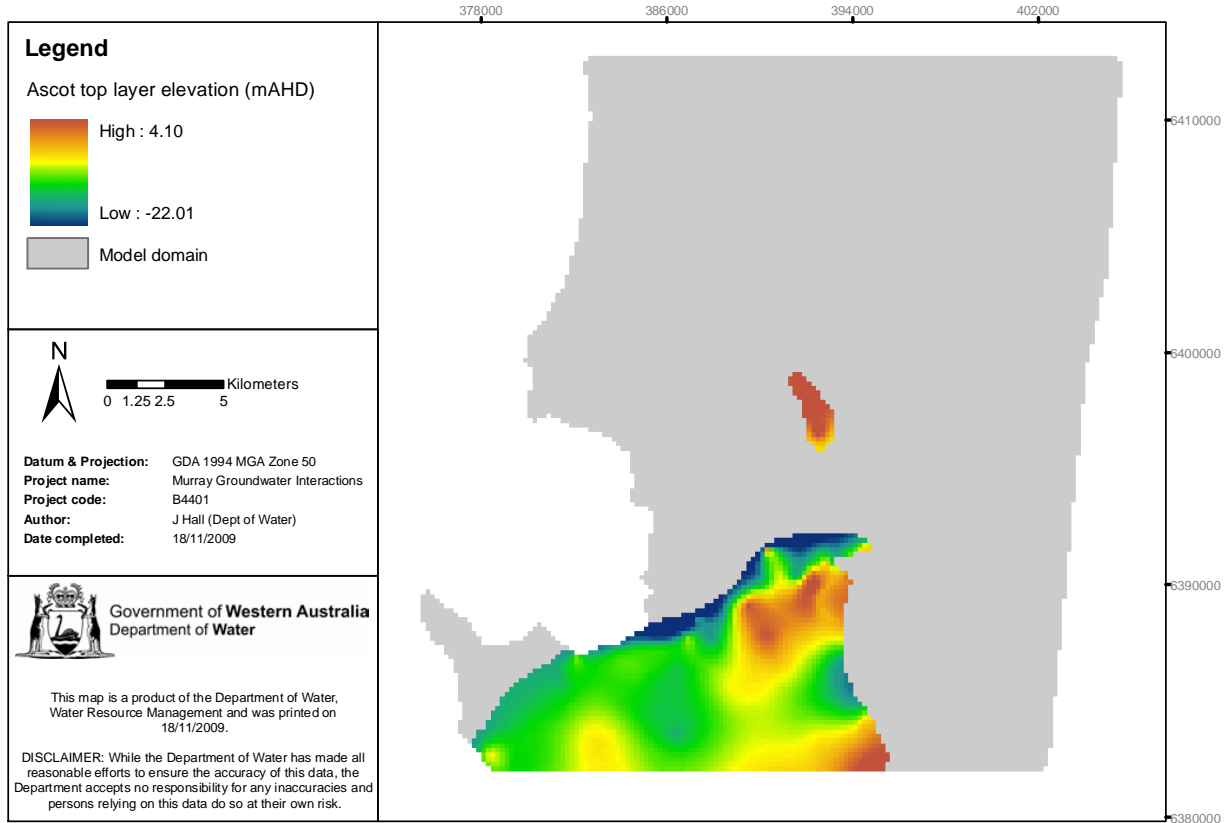
Figure 3-16: Ascot Formation: top of geological formation (mAHD)
