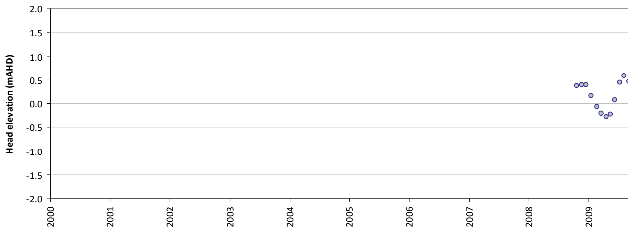
Residual time-series plot - HS92B
