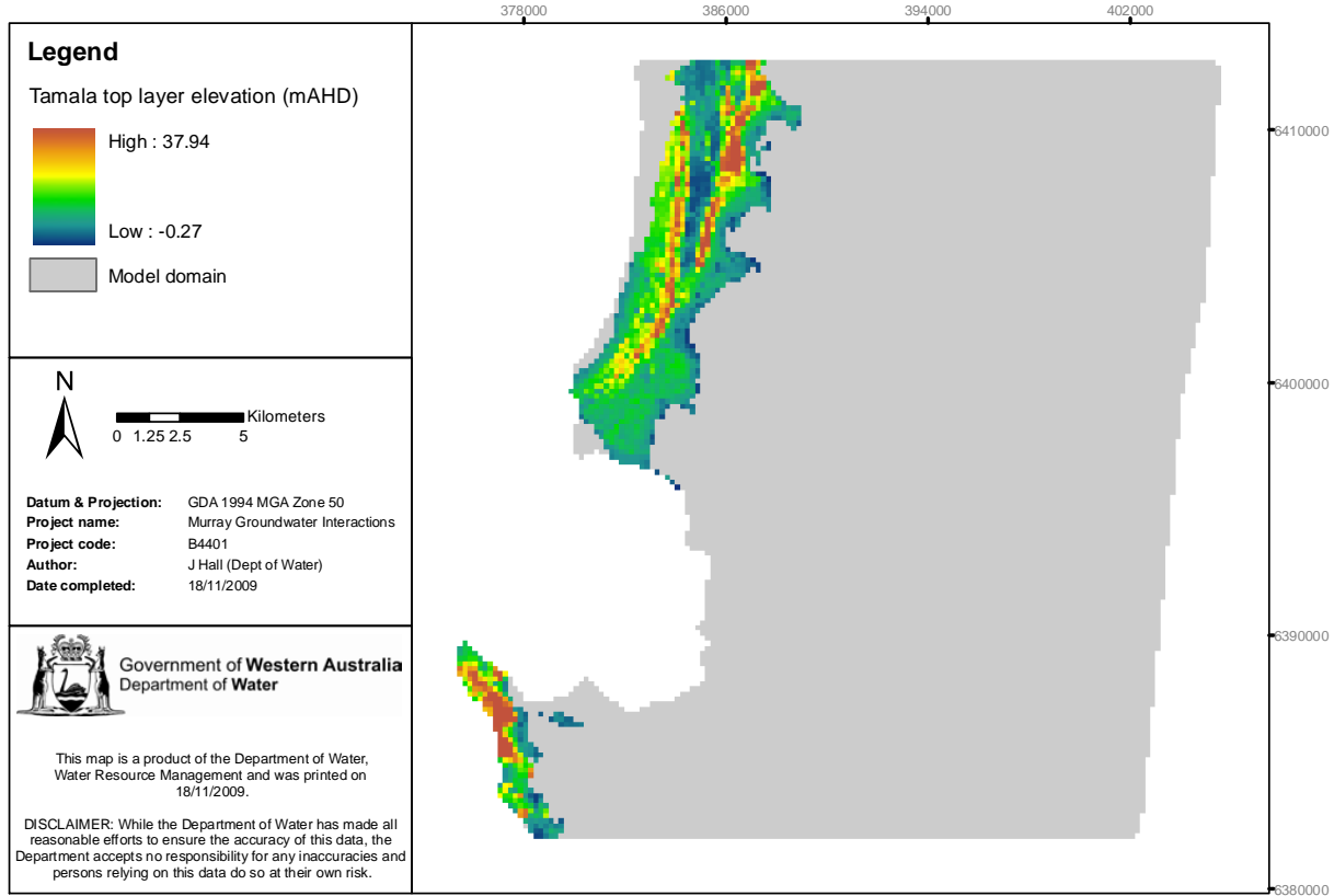
Figure 3-24: Tamala Limestone: top of geological formation (mAHD)
