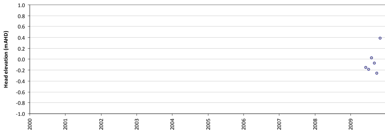
Residual time-series plot - HS104-3A
