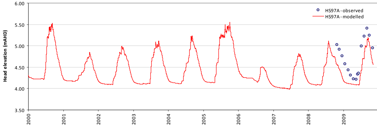
Modelled vs observed time-series plot - HS97A
