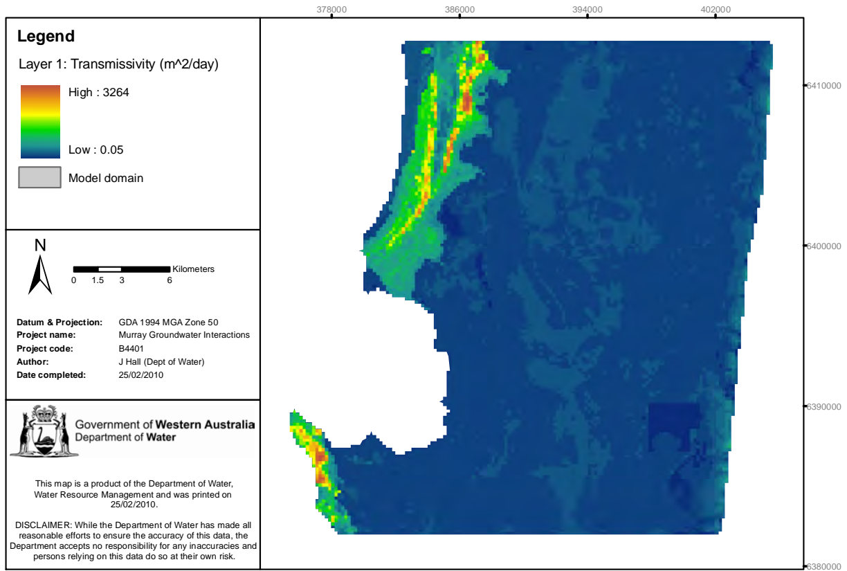
Figure 4-13: Computational layer 1 - transmissivity (m 2 /day)
