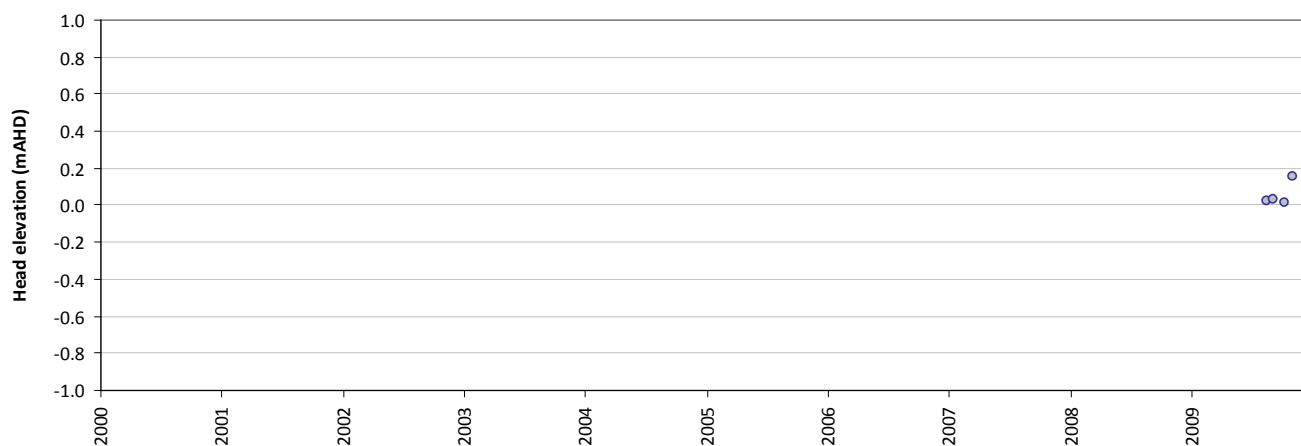
Residual time-series plot - PLI5033
