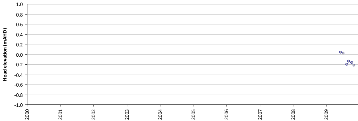
Residual time-series plot - HS087-3
