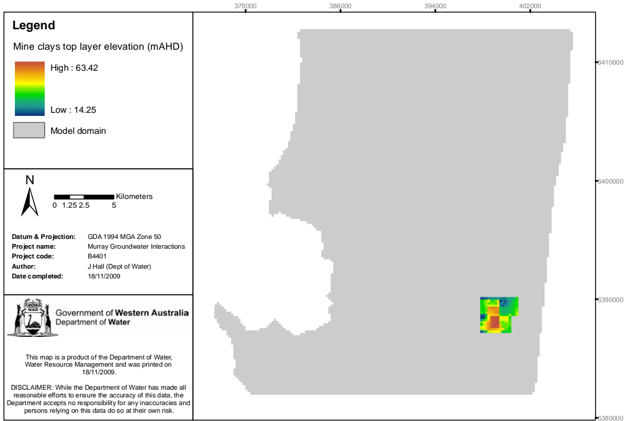
Figure 3-30: Mine clays: top of geological formation (mAHD)
