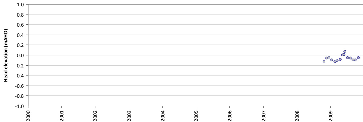
Residual time-series plot - HS91A
