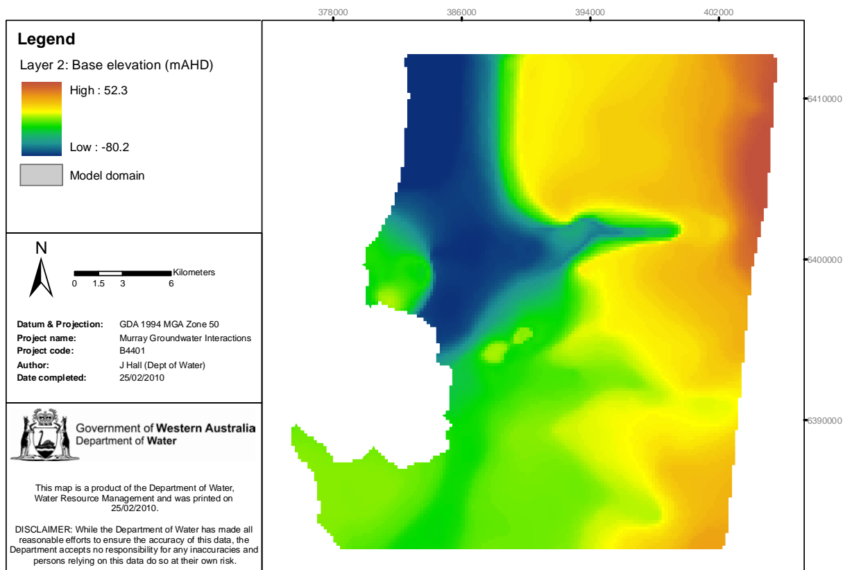
Figure 3-34: Base of computational layer 2 (mAHD)
