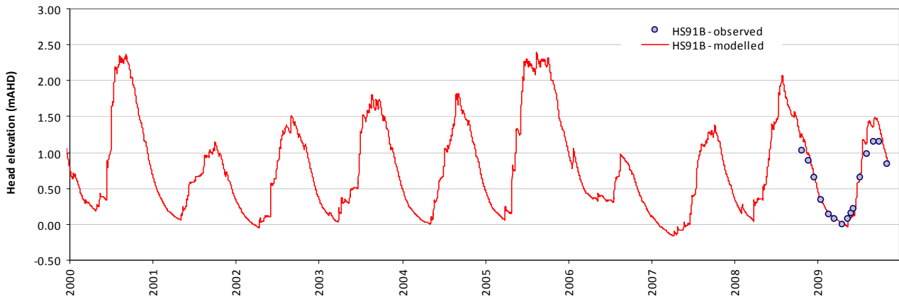
Modelled vs observed time-series plot - HS91B
