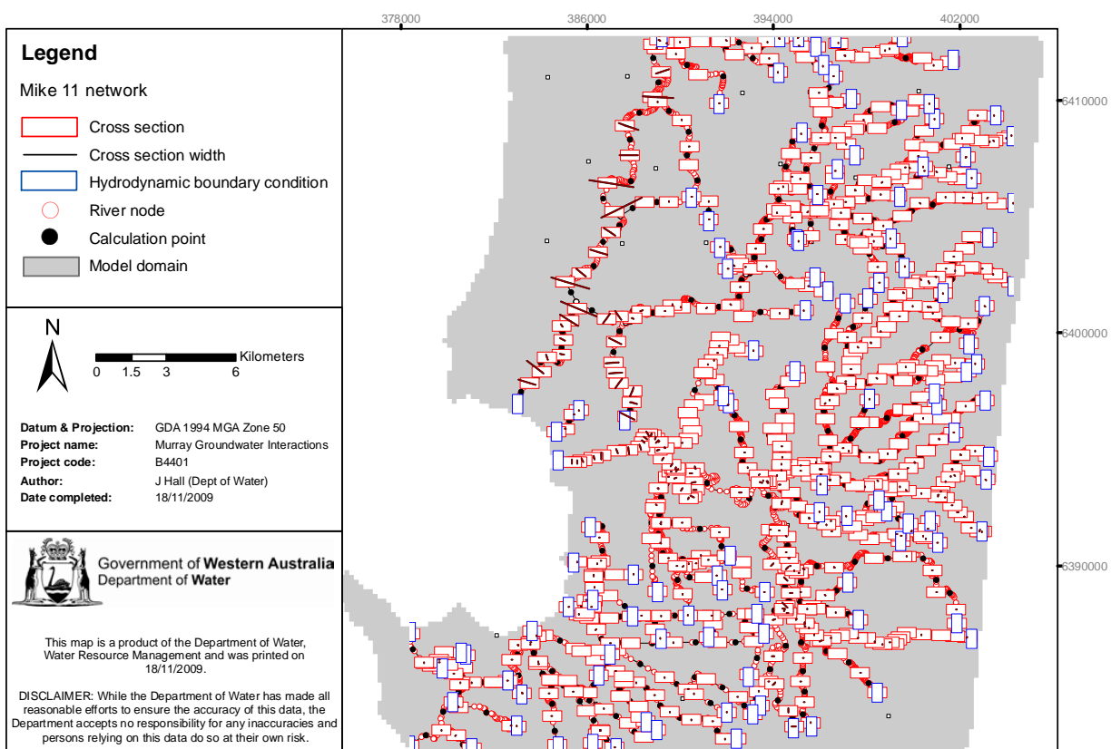
Figure 3-11: Mike 11 channel nodes, cross sections and boundary locations
