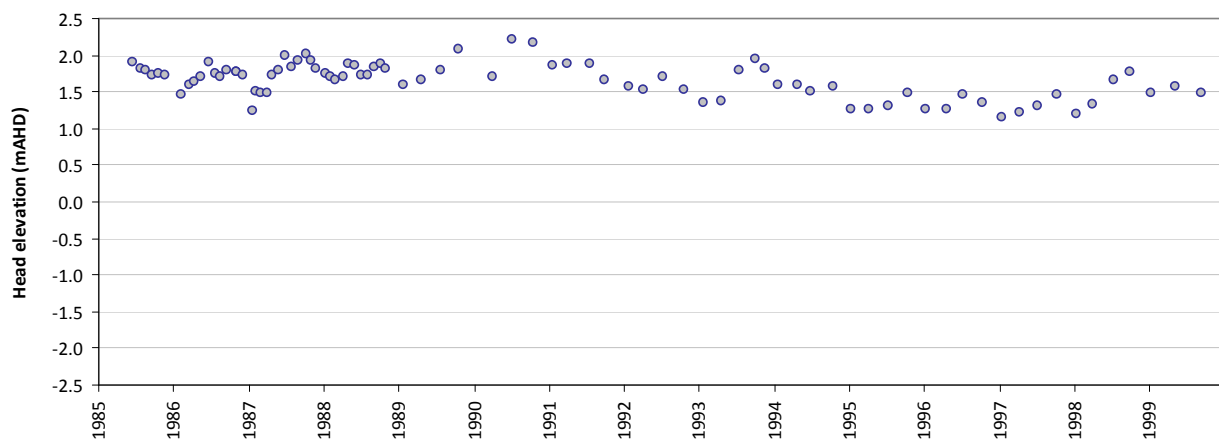
Residual time-series plot - T650
