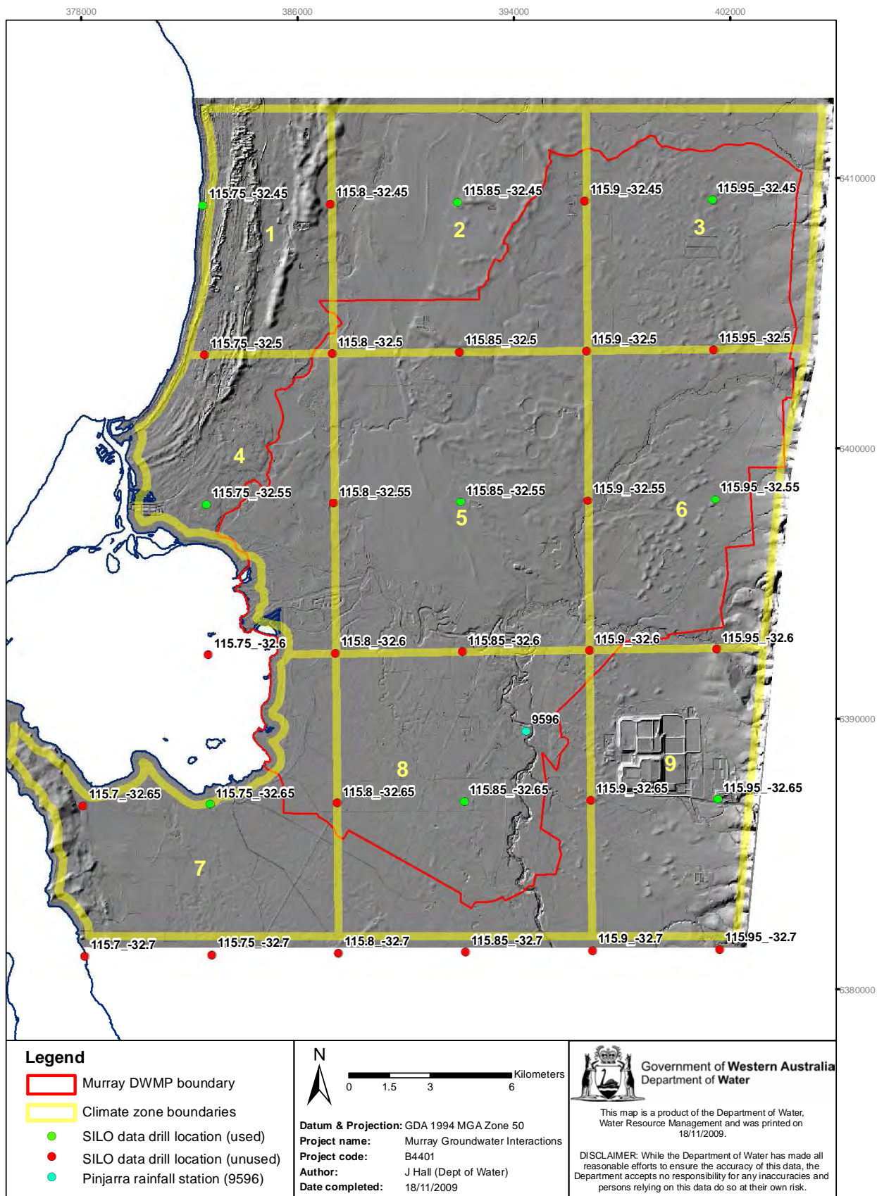
Figure 3-3: SILO rainfall locations and climate zones for the Murray regional model
