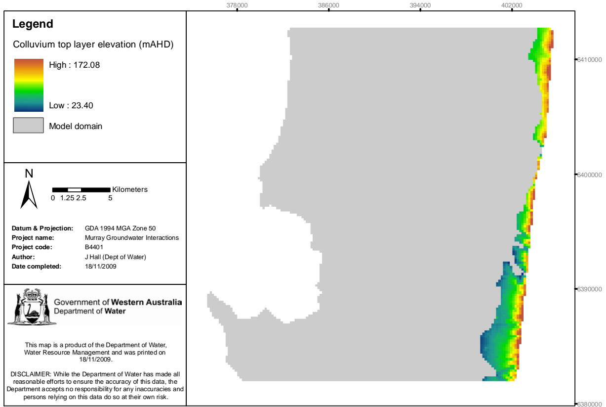
Figure 3-28: Colluvium: top of geological formation (mAHD)
