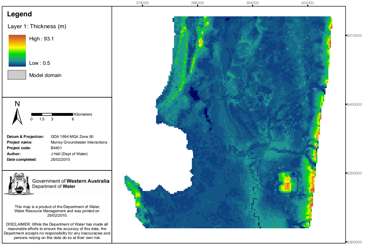
Figure 4-5: Computational layer 1 - thickness (m)
