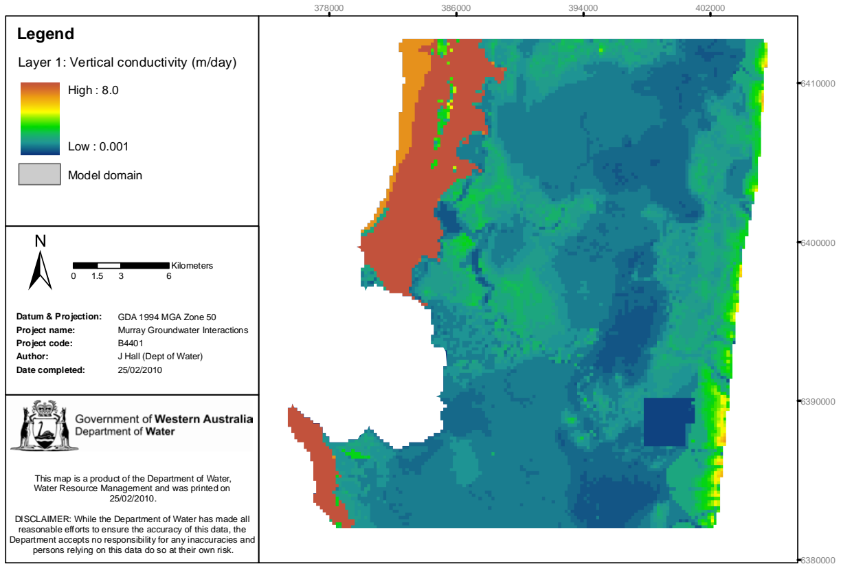
Figure 4-9: Computational layer 1 - vertical hydraulic conductivity (m/day)
