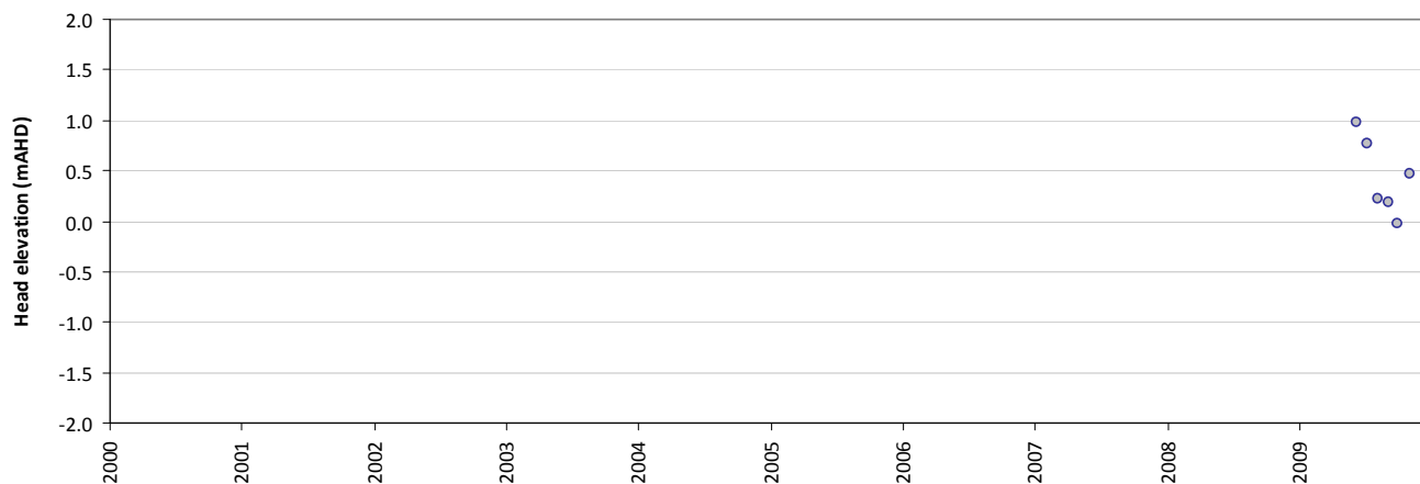
Residual time-series plot - HS108-1B
