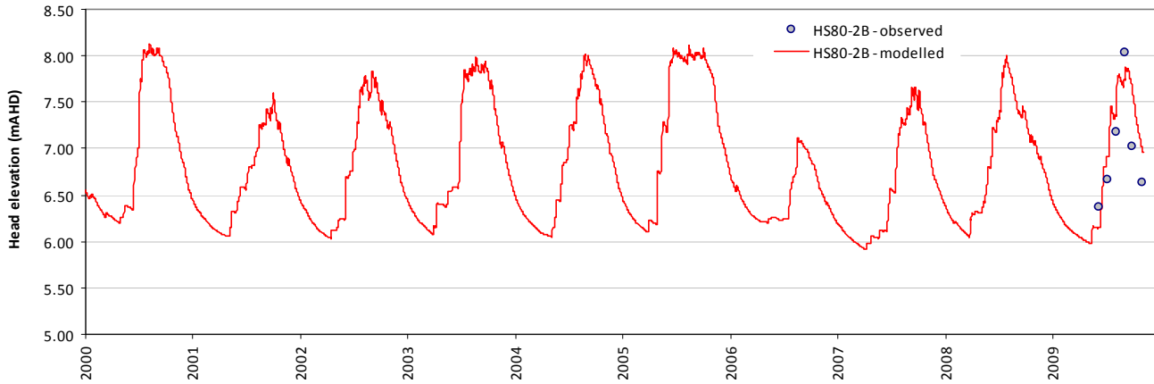
Modelled vs observed time-series plot - HS80-2B
