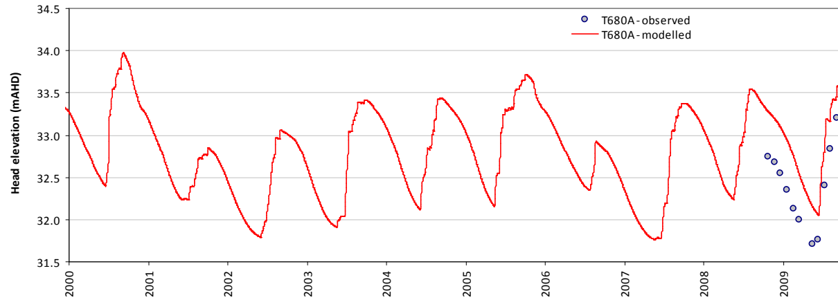
Modelled vs observed time-series plot - T680A
