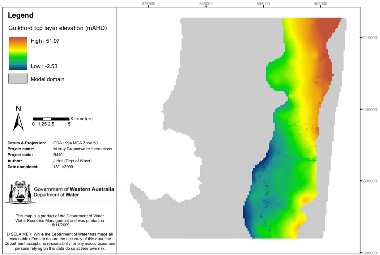
Figure 3-20: Guildford Clay: top of geological formation (mAHD)
