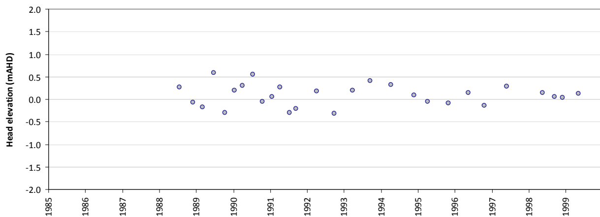
Residual time-series plot - HS56A
