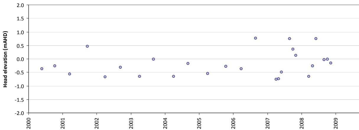
Residual time-series plot - HS50A
