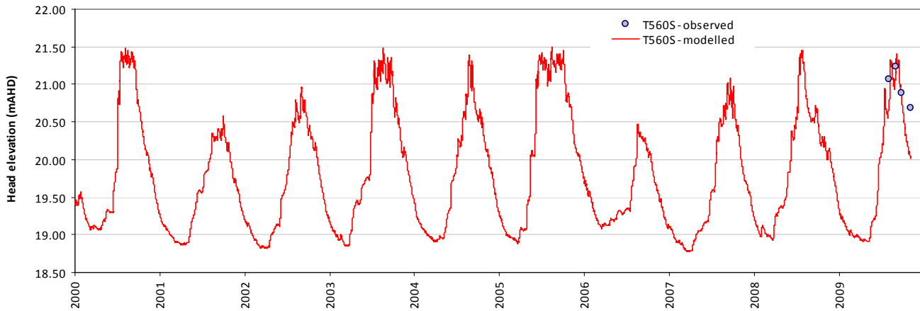
Modelled vs observed time-series plot - T560S
