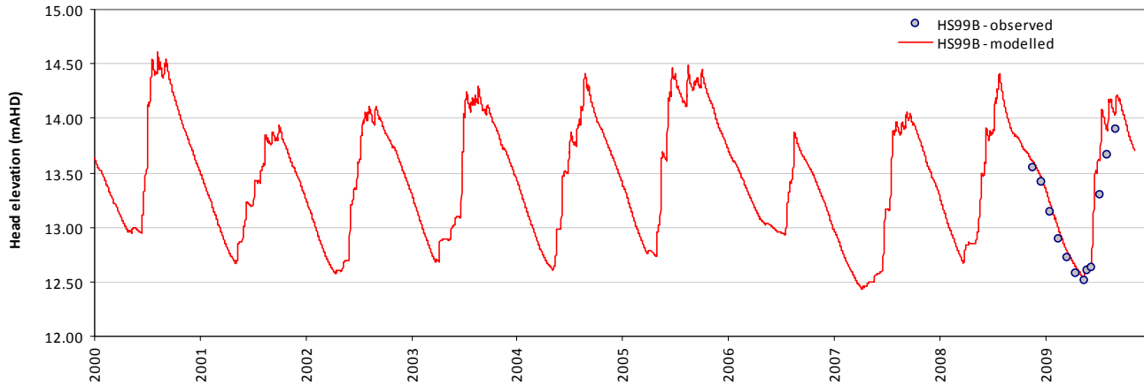
Modelled vs observed time-series plot - HS99B
