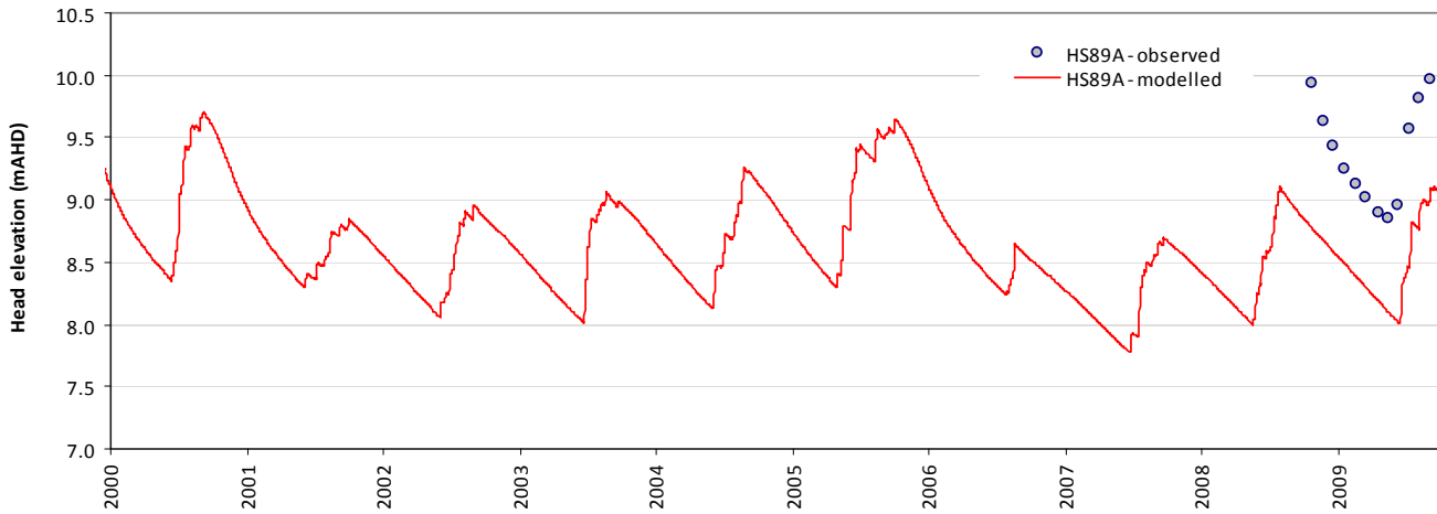
Modelled vs observed time-series plot - HS89A
