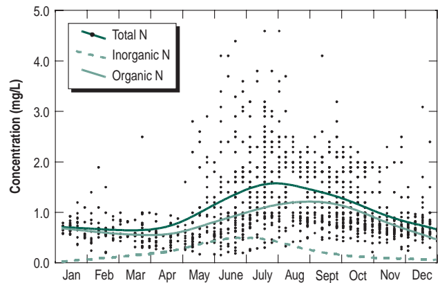
Figure 6: Seasonal variation in total nitrogen and fractions for all monitored sites in the Wilson Inlet catchment.
