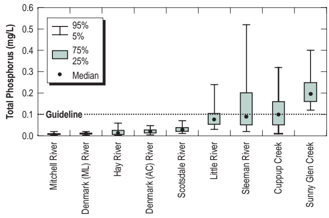
Figure 3: Box plots showing the combined distribution of nutrient (TN and TP) concentration data for rivers in Wilson Inlet catchment since monitoring commenced. The guideline concentrations are 1.0 mg/L for TN and 0.1 mg/L for TP.
