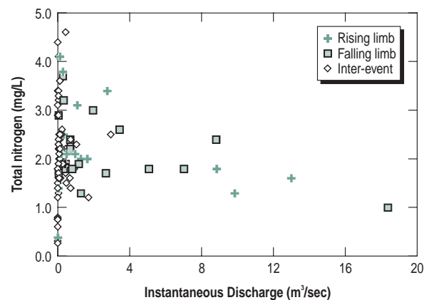
Figure 10: A combined positive and negative flow response in TN for Cuppup Creek.
