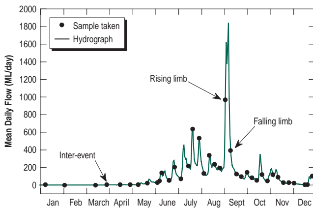
Figure 8: A comparison of when samples were taken relative to the 1995 Hay River hydrograph. According to the time the samples were taken, they were classed either as rising limbs (rising flow), falling limbs (falling flow) or inter-event (steady or base flows).
