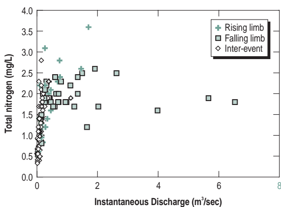
Figure 9: A positive flow response in TN for Sleeman River. This plot is typical of the rivers of Wilson Inlet catchment.
