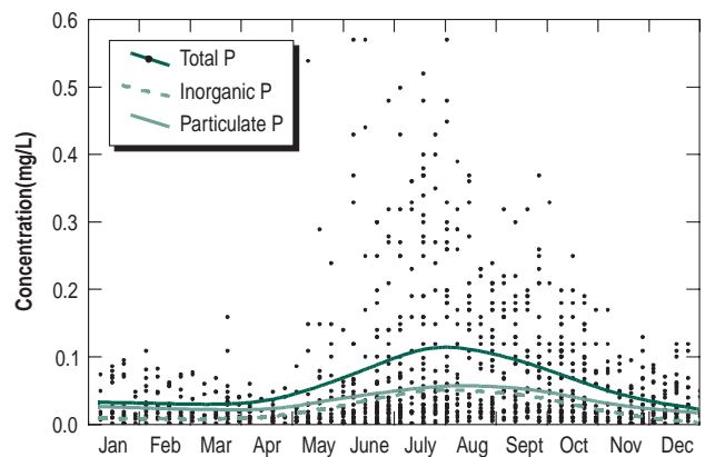
Figure 7: Seasonal variation in total phosphorus and fractions for all monitored sites in the Wilson Inlet catchment.
