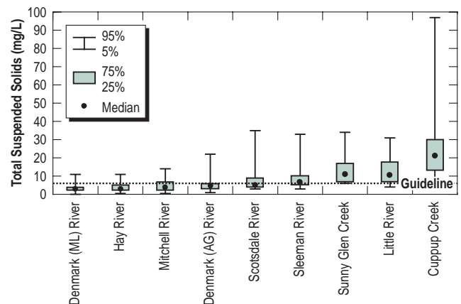
Figure 4: Box plots showing the distribution of TSS data for monitored sites in Wilson Inlet catchment. The guideline TSS concentration is 6 mg/L.
