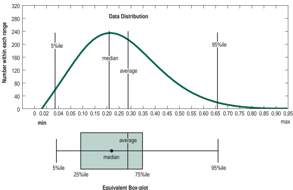
Figure 2. An example of a typical data distribution curve of total phosphorus concentrations for a monitored river. The box plot also describes the data distribution and can represent specific points, such as median and percentiles, of the data distribution curve.
