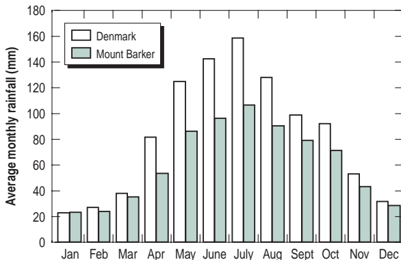
Figure 5: Average monthly rainfall for Denmark and Mount Barker weather stations (source: Bureau of Meteorology).
